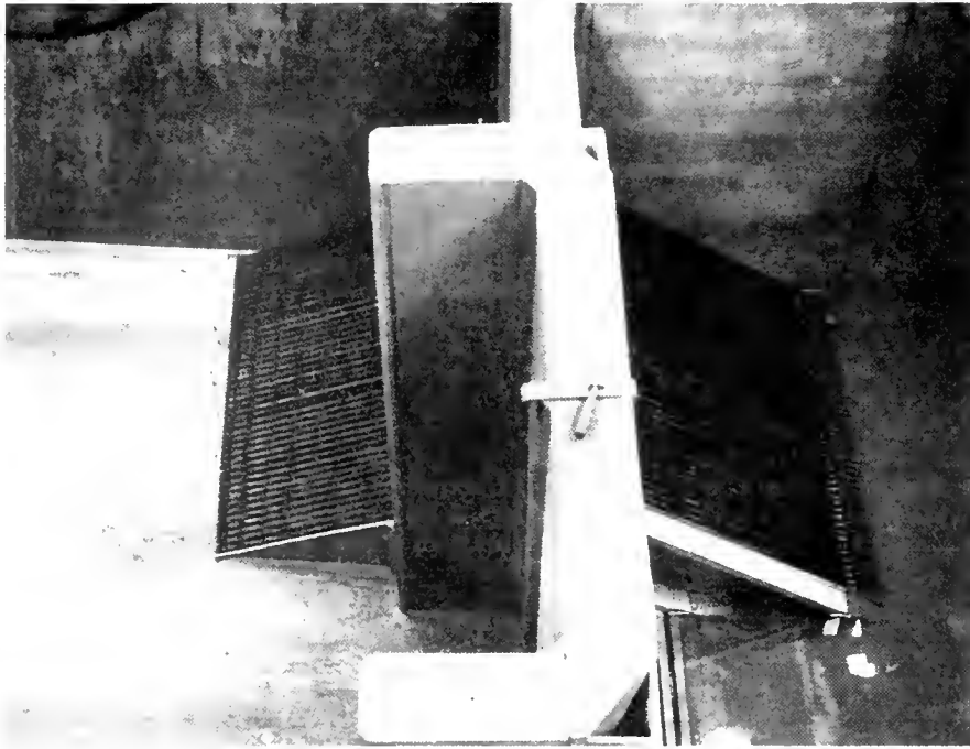
Figure 12.--Grills prevented orifice passage of fish at weir 54. All fish entering fishway passed over weir crest where they could be observed.
