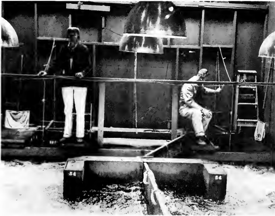
Figure 11.--Two release compartments and introductory area of the Ice Harbor fishway. Observer on right has opened gate to receive a fish from the collection pool. Observer on left has released a fish into the divided fishway and is recording progress of the fish as it passes over weirs in the six-pool ascent. Button switches on the handrail are used to transmit weir crossings to a time-event operations recorder.
