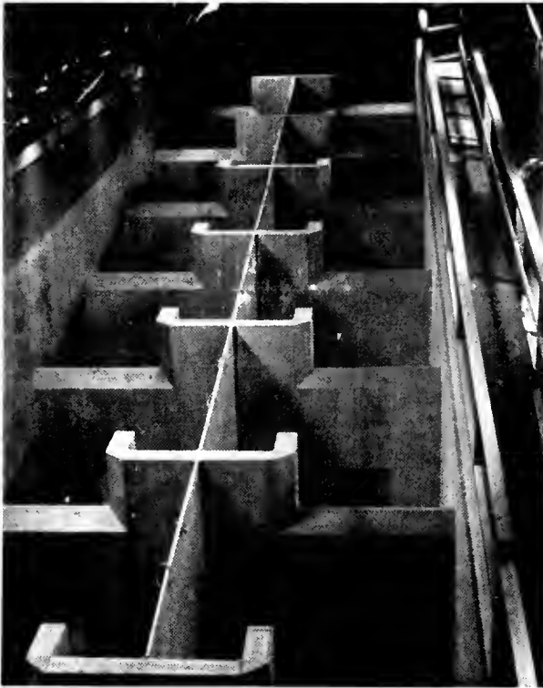
Figure 3.--Six-pool test section of the 1-on-10-slope Ice Harbor fishway design. Divider panels inserted for optional testing under a half-width condition.
