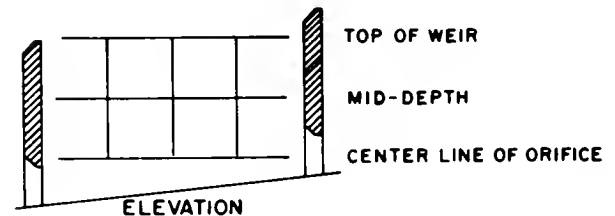
Figure 5.--Metering stations in the test fishway pool divided at center line. Dotted lines in plan view indicate additional metering stations at center line (elevation) of orifices only.
