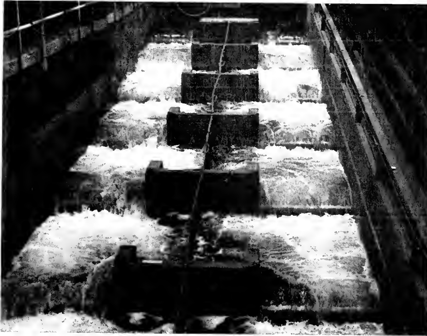
Figure 16.--Operational view of the Ice Harbor fishway with McNary-type weir crests on both sides. Orifices are functional on the left and closed on the right. Weirs have 0.95-foot head.
