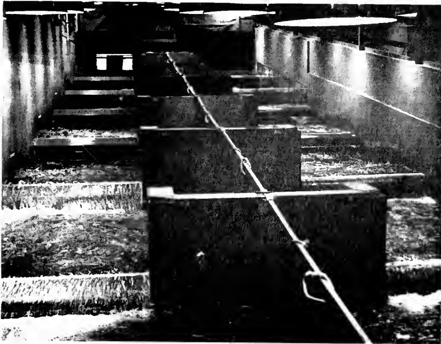
Figure 17.--Operational view of the Ice Harbor fishway during orifice flow.
