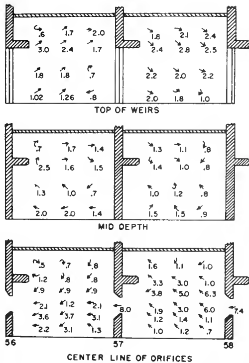
Figure 8.--Velocities (f.p.s.) and direction of flow with all of the discharge confined to the orifices.
