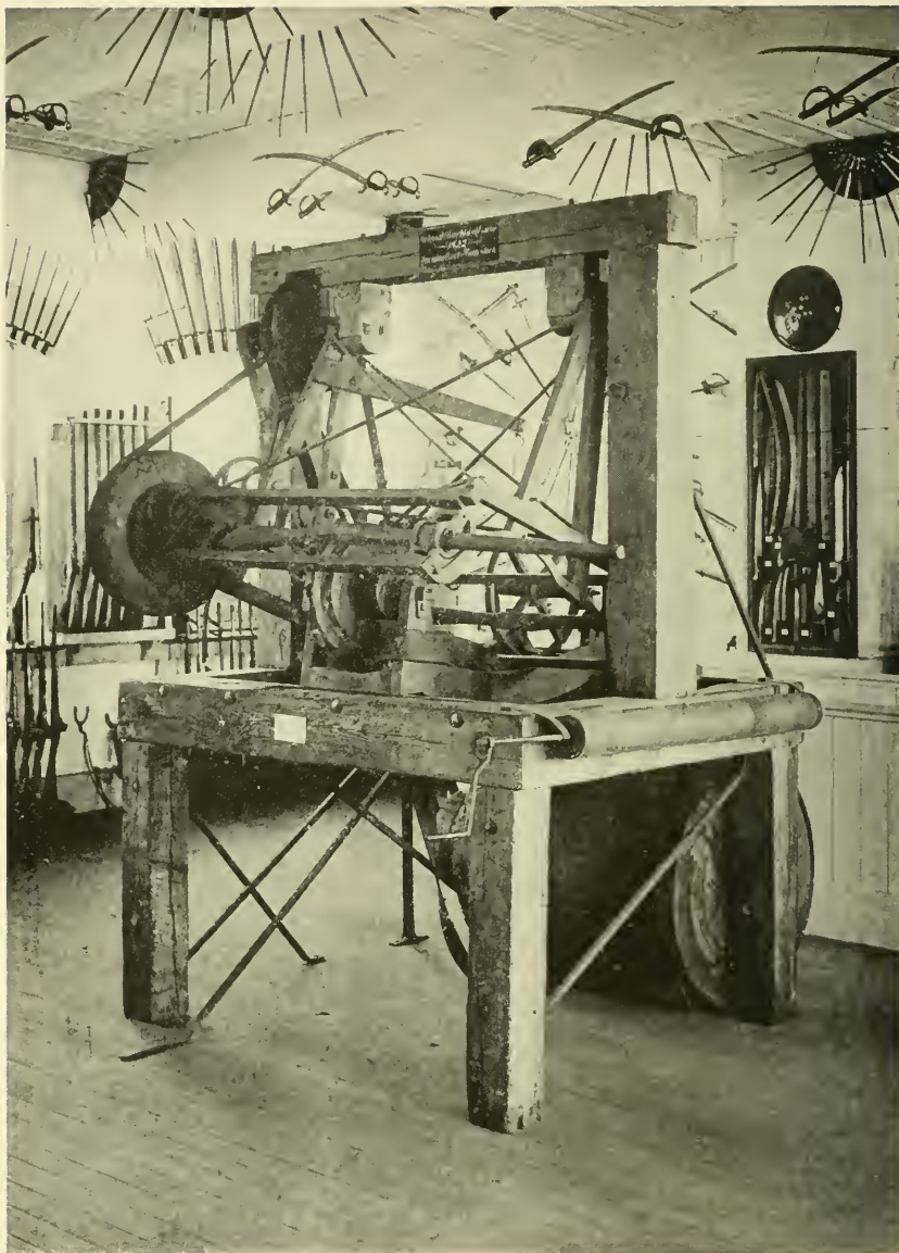
The Old Blanchard Invention for Turning Gun stocks
