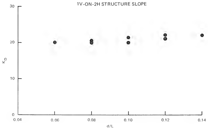
Figure 2. Stability coefficient ( K_D ) versus relative depth ( d/L )
