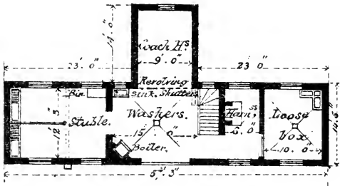
GROUND PLAN.
