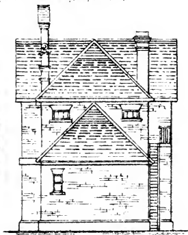
END ELEVATION.
