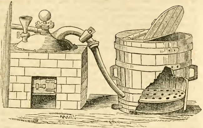
FIG. 17.—STEAMING APPARATUS.
