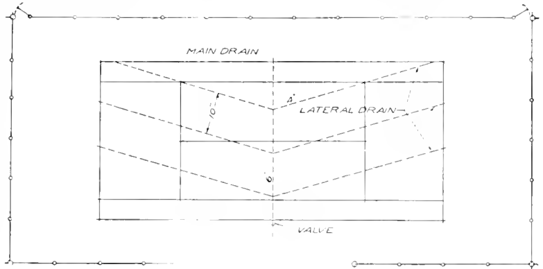
1357. Draining a tennis-court.
