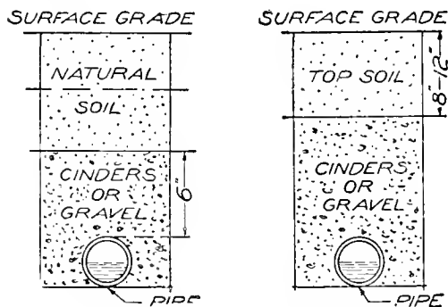
1354. The filling of a drain.
