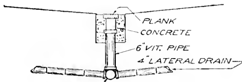
1360. Detail of drain connections. (See Fig. 1356.)
