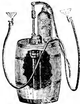
1331. An orchard barrel pump.
