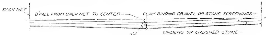
1356. Draining a tennis-court.
