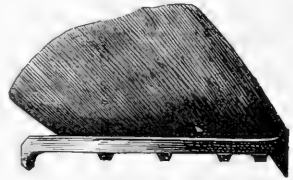
FIG. 489.—Ordinary Calks.
