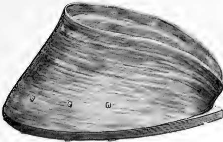
FIG. 487.—Shoe Properly Adjusted and Nailed.
