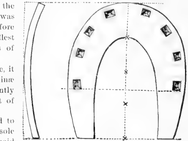
FIG. 578.—French Shoe.
