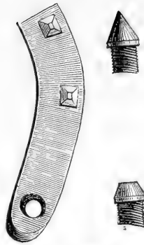
FIG. 491.—Adjustable Calks.
