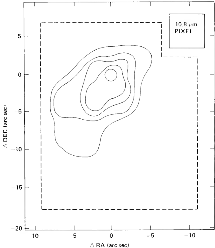
Figure 2. NGC 1808 (Sbc pec.) at 10.8 \mu\text{m} . The contour levels (mJy/pxel) are: 200, 300, 400, 500, and 600.
