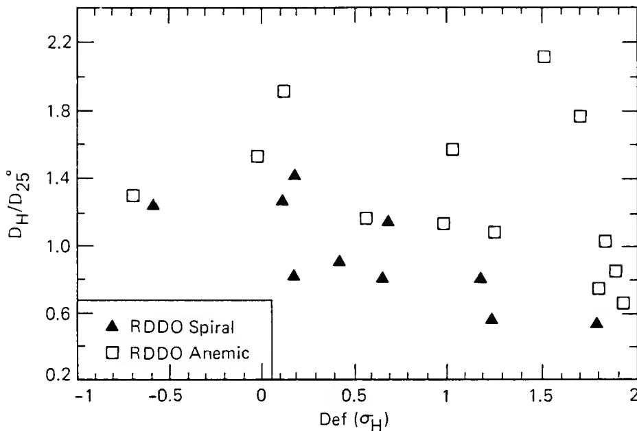
Figure 2 - HI/optical diameter ratio D_{\text{H}}/D_{25}^{\circ} versus deficiency parameter \text{Def}(\alpha_{\text{H}}) . See text for definitions. Triangles = RDDO spirals. Squares = RDDO anemics.
