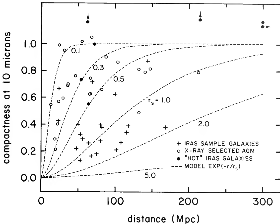
Figure 1. The 10\ \mu\text{m} "compactness" (see text) of IRAS sources plotted against their distance in megaparsecs. The dashed lines represent a model in which the surface brightness drops as \exp(-r/r_0) for a series of characteristic radii r_0 in kpc. Data for the main sample of "representative" and "hot" IRAS galaxies were obtained at the IRTF with a 5.5'' aperture. Data on the X-ray-selected AGN are taken from McAlary et al. (1983), with apertures ranging from 5'' to 9'' .
