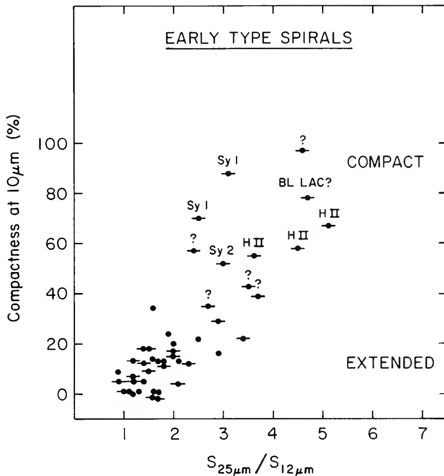
Figure 4. Compactness at 10\ \mu\text{m} versus IRAS S_{25\ \mu\text{m}}/S_{12\ \mu\text{m}} . Galaxies for which the central region dominates the flux at 12\ \mu\text{m} are compact. The IRAS S_{25\ \mu\text{m}}/S_{12\ \mu\text{m}} colors for the compact galaxies indicate that the central region dominates the 25\text{-}\mu\text{m} flux also. Barred galaxies are indicated by horizontal bars.
