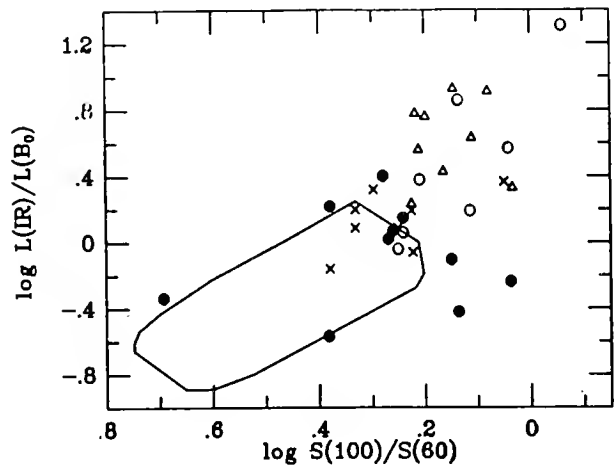
Fig. 2-The outlined region shows the area occupied by normal spiral galaxies (de Jong et al. 1984).
