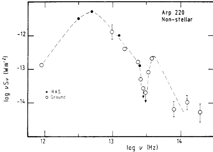
Figure 5: Energy distribution from 1 to 350 \mu\text{m} .
