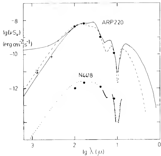
(f) Models for Arp 220 (broken curve: 'starburst' model with an additional A_V = 78 mag. of extinction by interstellar dust. Solid curve: power-law ( \alpha=0.7 ) continuum source embedded in uniform spherically symmetric dust cloud with \tau_{UV} = 186 ( A_V=40 ). The upper and lower solid curves at larger wavelengths correspond to whether the power-law source continues beyond 100 \mu or not.) and NGC 4418 (dotted curve: 'starburst' model with an additional A_V = 39 mag. of extinction by interstellar dust).
