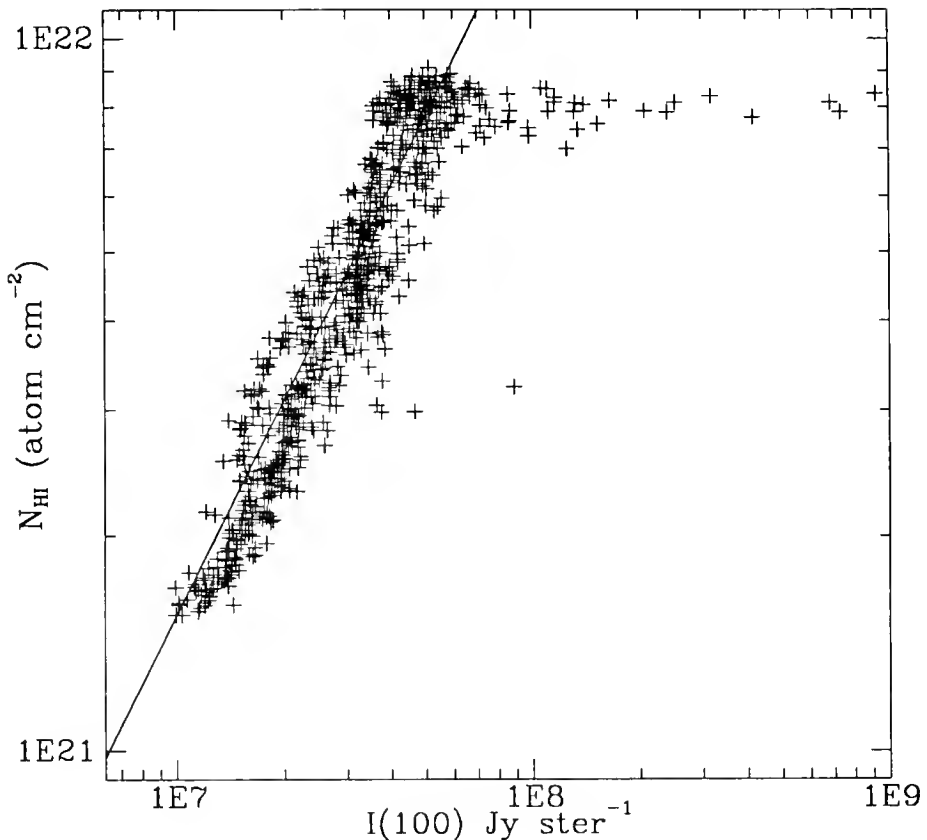
Figure 1. The HI column density is plotted against the IRAS 100\ \mu\text{m} intensity in the l = 125^\circ field. Contamination by non-cirrus infrared sources produces the high intensity 100\ \mu\text{m} points that don't follow the correlation. Solid line shows a least squares fit to the data (excluding non-cirrus sources).
