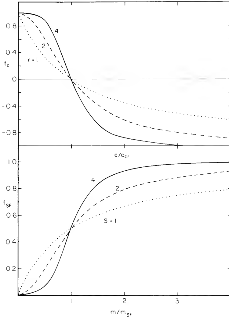
Figure 2. Several examples of the parametrized coalescence - disruption function f_c and star formation function f_{SF} are shown (from Struck-Marcell and Scalo 1986). Depending on the values of the parameters (especially the exponents r, s ), the form of these functions can range from nearly linear to an almost step function form. The latter implies a strong threshold behavior.
