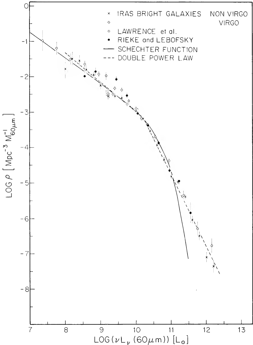
Figure 3: The 60 \mu\text{m} luminosity function derived for the Bright Galaxy sample, plotted as space density in galaxies per cubic Megaparsec per magnitude range in 60 \mu\text{m} luminosity vs 60 \mu\text{m} luminosity. The 60 \mu\text{m} luminosity is taken as \nu L_{\nu} (60 \mu\text{m}) . For comparison the luminosity functions derived from different IRAS samples are shown as well. These are taken from Lawrence, et al. 1986 and Rieke and Lebofsky, 1986. Both a double power law and a Schechter type luminosity function are shown for comparison with the observed luminosity functions.
