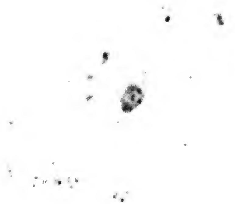
Figure 1. Continuum-subtracted H\alpha + [NII] image of the nuclear region of NGC 5248. The ring of HII regions around the actual nucleus is evident. The field is 160" square, with north at the top.
