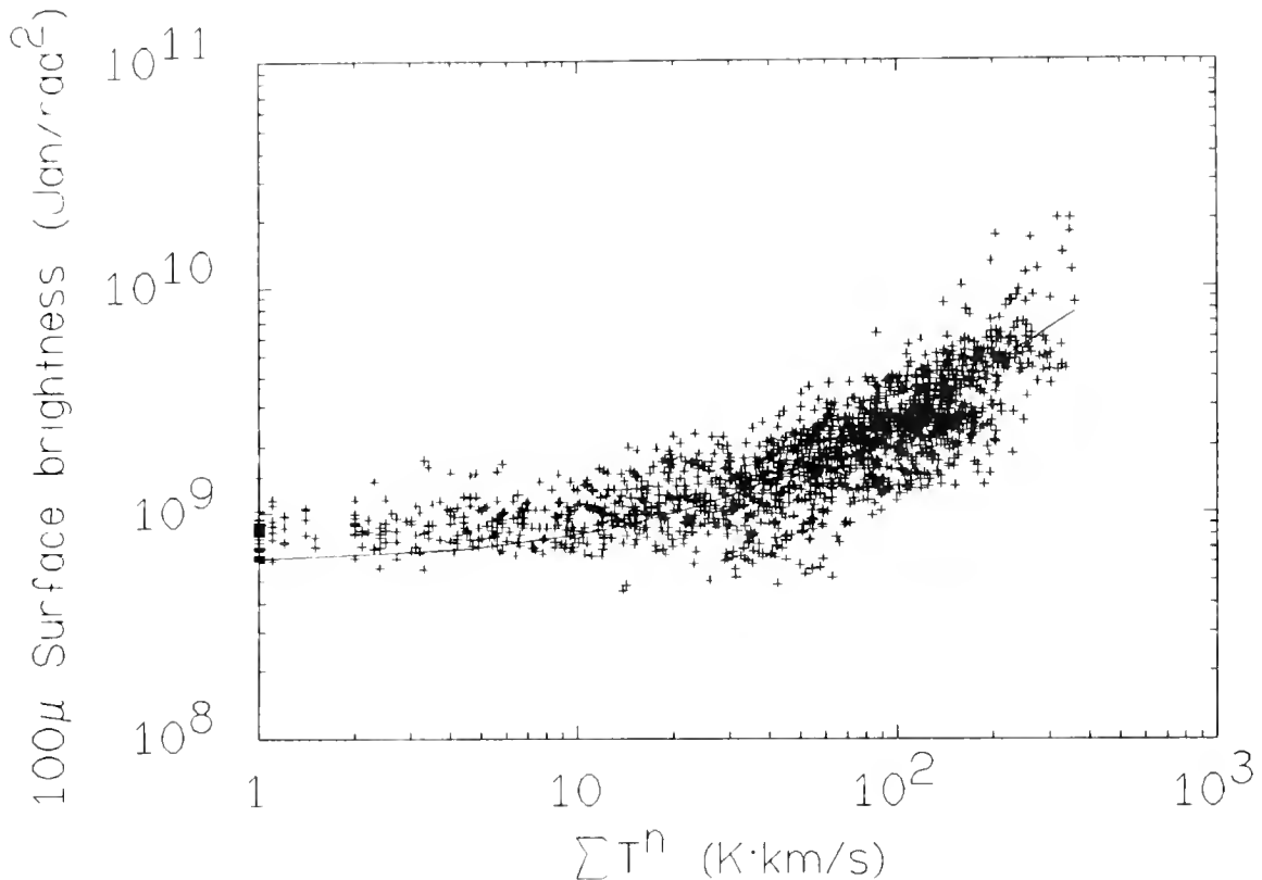
Figure 5. A point by point correlation of IR brightness as a function of CO integrated intensity ( T_R' > 1 K; -40 < v < +140 km \cdot s ^{-1} ) for a 2^\circ by 2^\circ region of the galactic plane between \ell = 29^\circ to 31^\circ , b = -1^\circ to +1^\circ . There is substantial far IR emission uncorrelated with CO integrated intensity below about 40 K \cdot km \cdot s ^{-1} , which provides an estimate of the IR background wrt the molecular clouds. The 100 micron background here is about 8 \times 10^8 Janskys/steradian.
