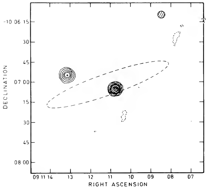
Figure 1b - A VLA map of A 09111-1007 at 20 cm. Peak brightness is 22 mJy/beam. This figure is taken from Farouji et al. (1986).
