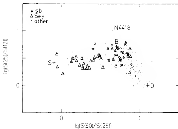
Fig 2 IRAS colour-colour diagrams for unresolved IRAS galaxies with high-quality fluxes in all 4 bands. Circled dots are star-burst (or HII) galaxies, triangles are Seyferts, dots are neither of these or unclassified to date. The crosses labelled D, B, S, are the adopted colours of the 'disc', 'starburst' and 'Seyfert' components used to synthesize the observed far infrared spectra.
