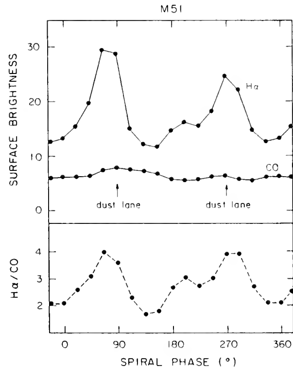
Figure 5. H\alpha and CO azimuthal distributions in M51 at 45" resolution (top) plotted as a function of spiral phase, with 90^\circ and 270^\circ chosen to be the locations of the arms ( H\alpha from Kennicutt 1983; CO from Lord and Young 1986). Also shown (bottom) is the H\alpha/CO ratio as a function of spiral phase; the highest values of this quantity are found on the spiral arms in M51.
