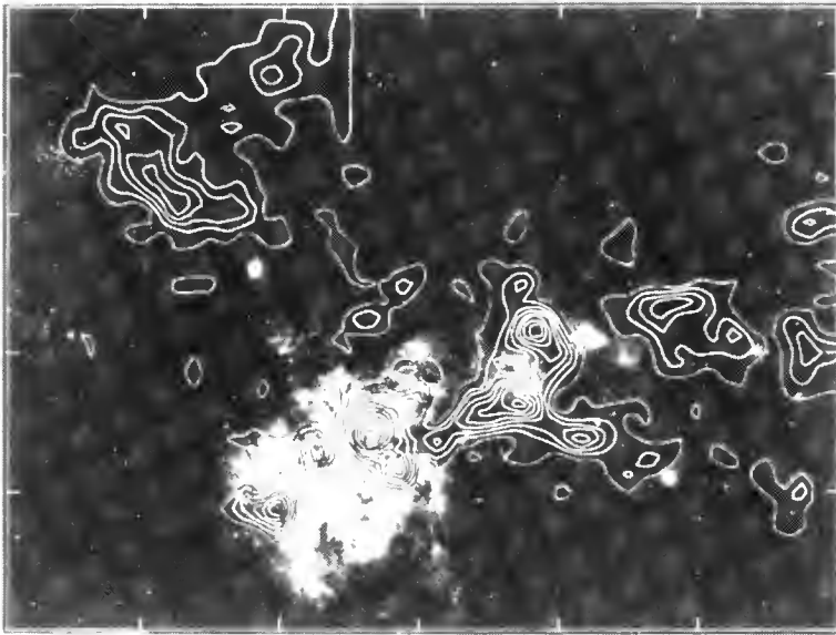
FIGURE 1. Mosaic of ESO J plates showing the \eta Carinae nebula and its surroundings. The overlaid contours show CO emission integrated over velocity from -50 to -9 \text{ km s}^{-1} . The contour interval is 5 \text{ K km s}^{-1} . Note the good correlation between the CO and the dust lanes in the vicinity of the bright gas. This dust represents a fragment of the molecular cloud that is being driven out by the HII region.
