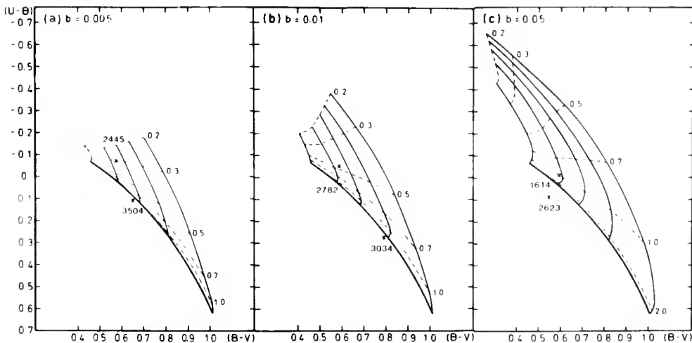
Figure 4. (U-B) vs (B-V) diagram : starburst galaxies.
