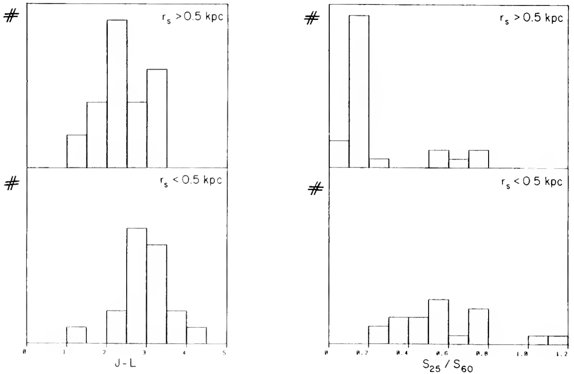
Figure 2. The distributions in J-L and 25-60 \mu\text{m} flux density ratio ( S_{25\mu\text{m}}/S_{60\mu\text{m}} ) for sources with characteristic 10 \mu\text{m} radii r_0 > 0.5 \text{ kpc} and < 0.5 \text{ kpc} (sources for which there are only L' rather than L measurements have been corrected).
