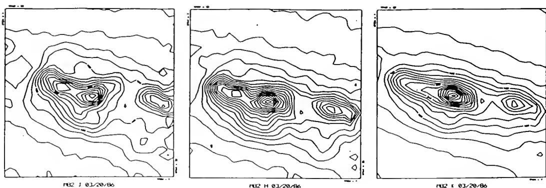
Figure 1. Images of M82 at J, H, and K (left to right). The frames are 27 arcsec on a side and the pixels are 0.85"; the data have been smoothed to a final resolution of 1.7". At K, the image shows a reasonably symmetric, smooth distribution of stars that suggests an edge-on disk around a brighter nucleus. Note the strong distortions from interstellar extinction as the wavelength becomes shorter.
