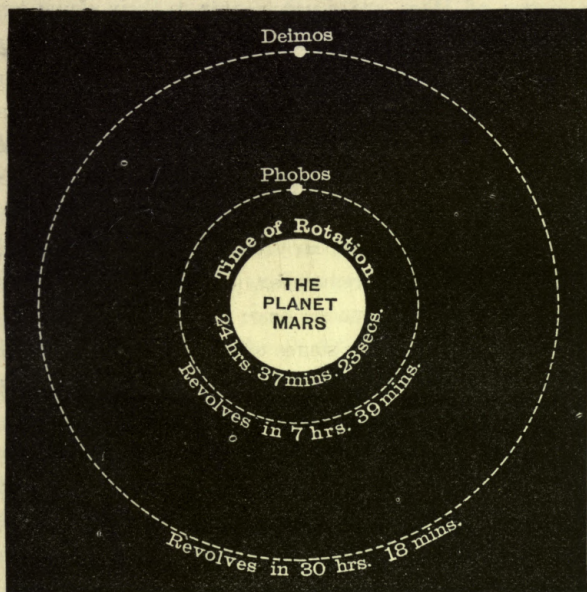
Fig. 61.—Mars and his two Satellites.
