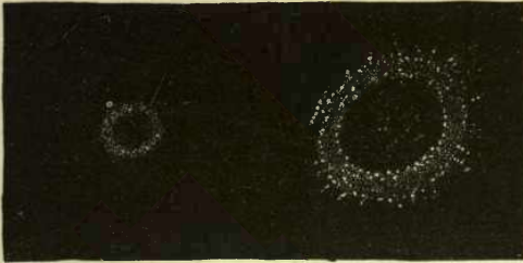
Fig. 85.—The Ring Nebula in Lyra, under different telescopic powers.
