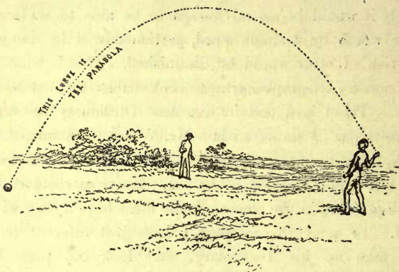
Fig. 72.—The Path of a Projectile is a Parabola.
