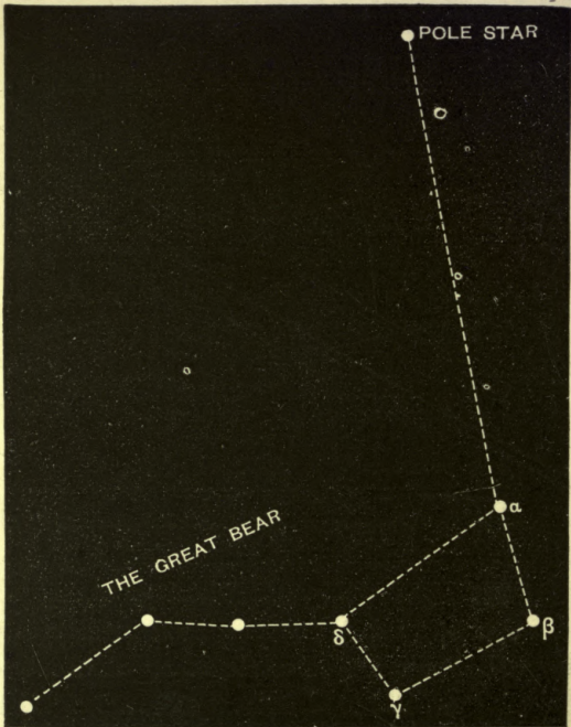
Fig. 90.—The Great Bear and the Pole Star.
