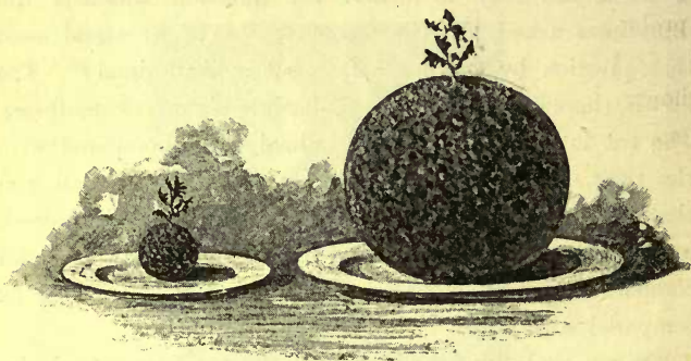
Fig. 31.—Relative Sizes of the Earth and the Moon.
