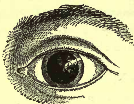
This shows the eye in the dark.
