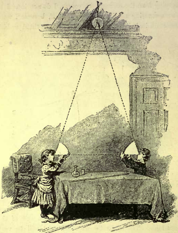
Fig. 5.—How we measured the height of the ball.
