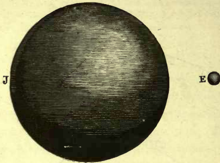
Fig. 64.—Jupiter and Earth compared.
