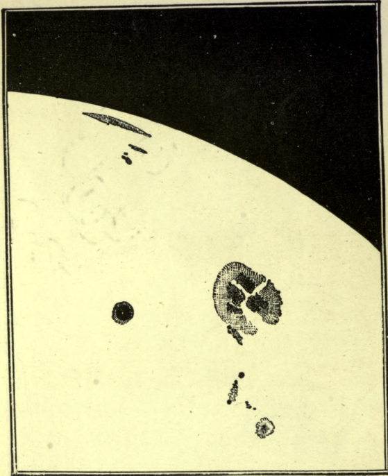
Fig. 16.—Spot nearing the Sun's Edge.
