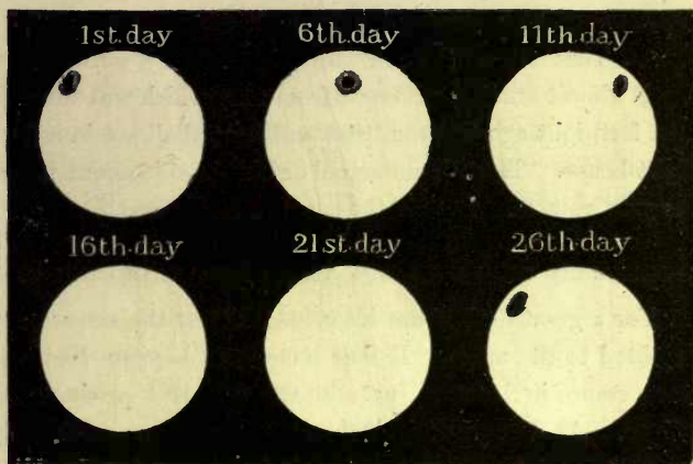
Fig. 17.—How the Sun turns round.
