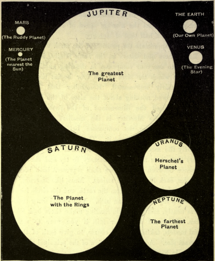
Fig. 46.—Comparative Sizes of the Planets.
