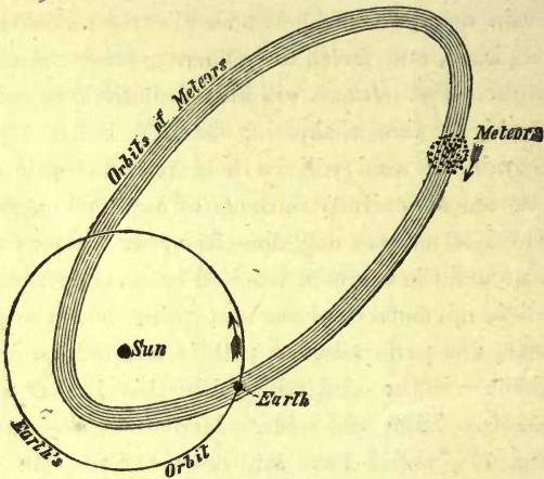
Fig. 78.—The Earth crossing the track of Meteors.
