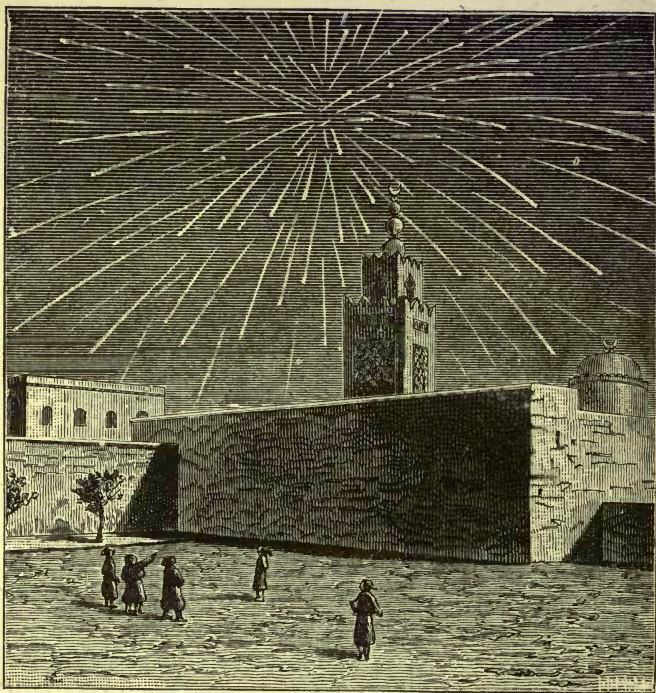
Fig. 77.— A Great Shower of Shooting Stars.
