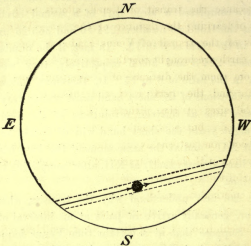
Fig. 50.—Venus in transit across the Sun.
