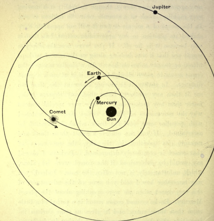
Fig. 71.—The Orbit of Encke's Comet.
