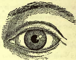
This shows the eye in daylight.
