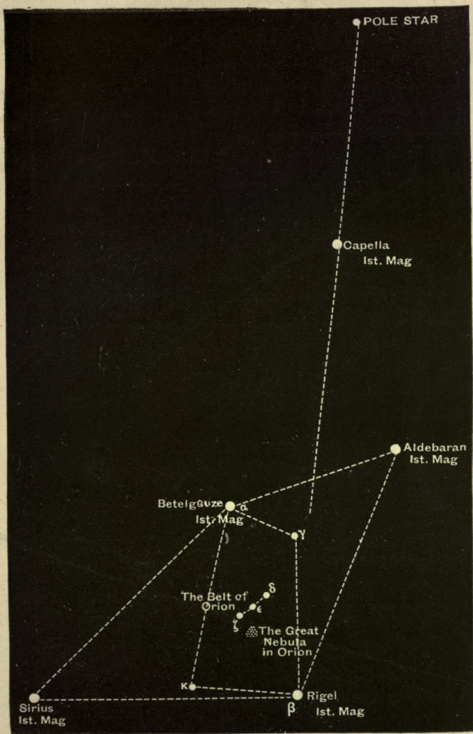
Fig. 92.—Orion and Sirius.
