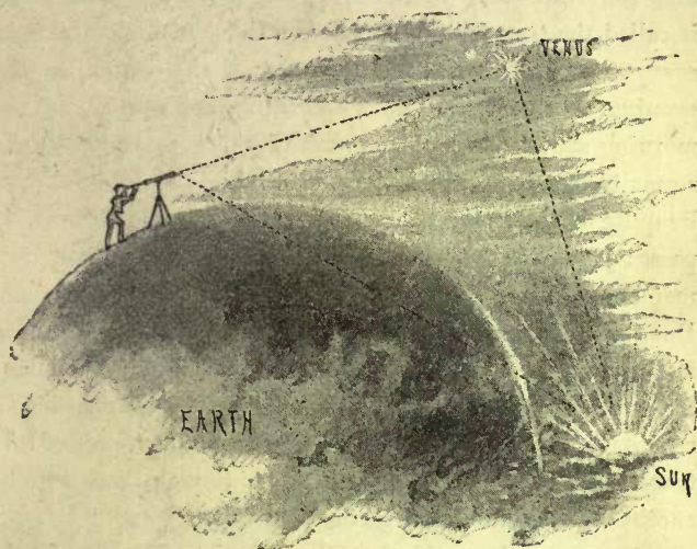
Fig. 49.—To show that Venus shines by Sunlight.
