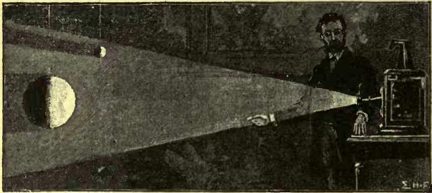
Fig. 27.—To show that the Moon is lighted by Sunbeams.
