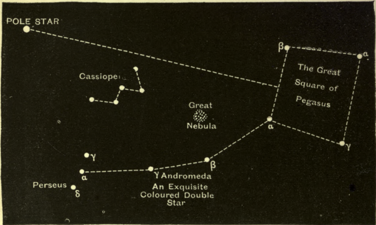
Fig. 91.—The Great Square of Pegasus.
