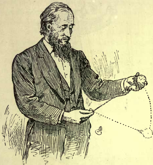
Fig. 41.—The Moon always turns the same face to the Earth.
