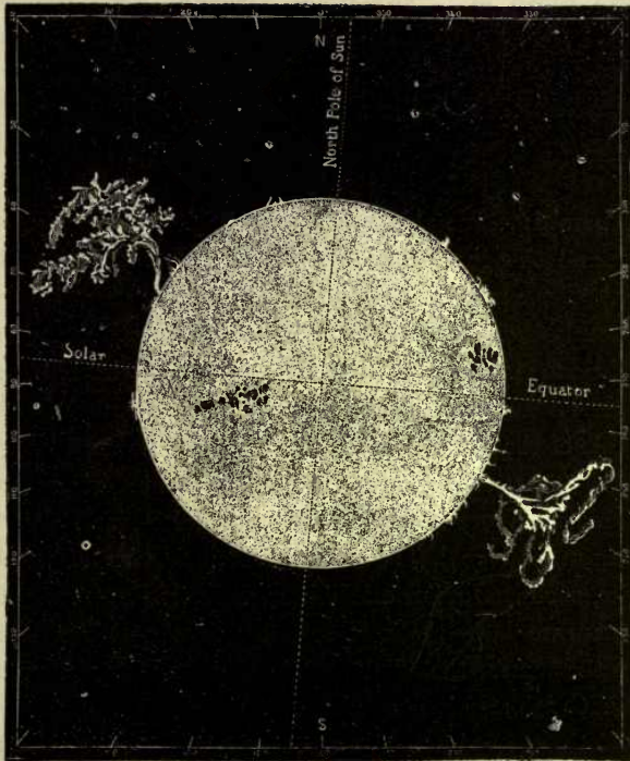
Fig. 19.—Solar Prominences. (Drawn by Trouvelot.)
