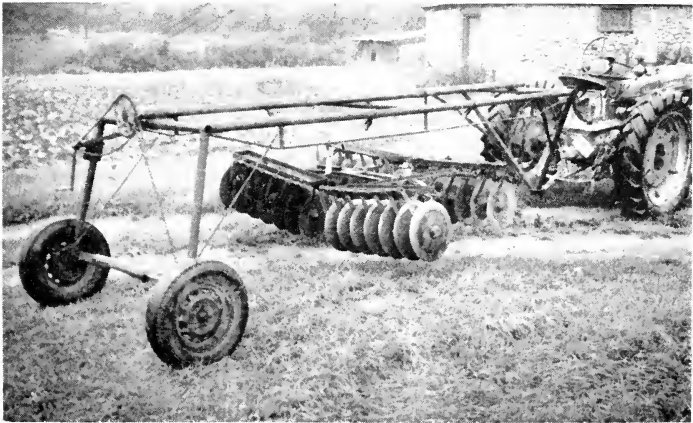
Figure 1. The overhead suspension type harrow carrier which was built by agricultural engineers at the University.
