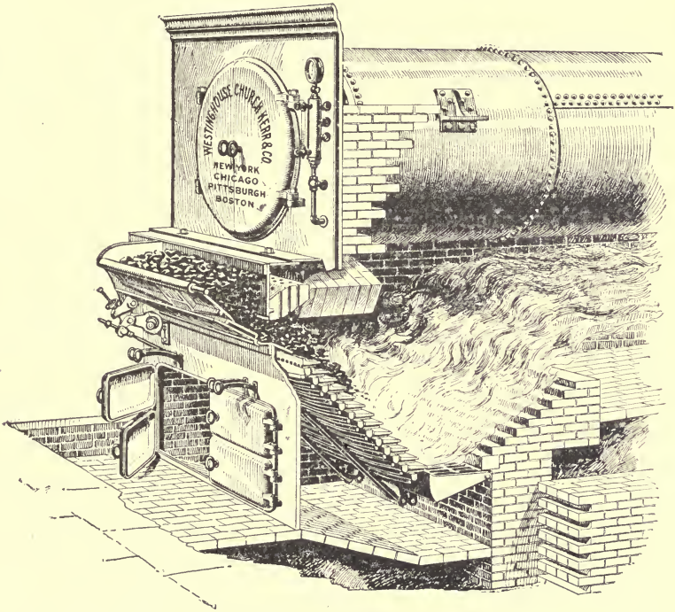
FIG. 26.—THE ROONEY MECHANICAL STOKER.
