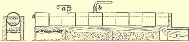
FIG. 41.—PLAIN CYLINDER BOILER.
