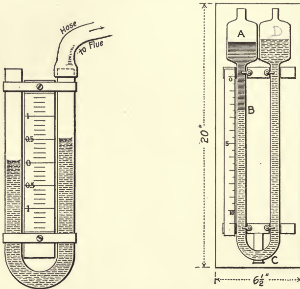
FIG. 112.—U-TUBE DRAFT-GAUGE, HALF SIZE.
