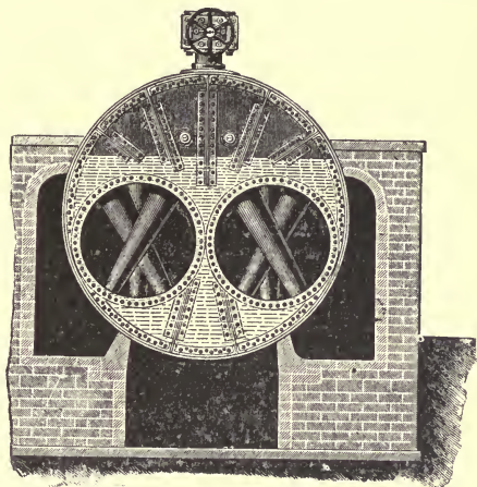
FIG. 60.—LANCASHIRE BOILER WITH GALLOWAY TUBES.
