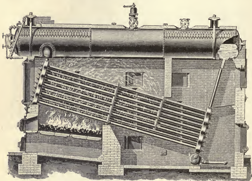
FIG. 94.—THE BABCOCK & WILCOX BOILER.
