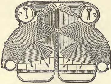
FIG. 105.—THE MOSHER BOILER.
