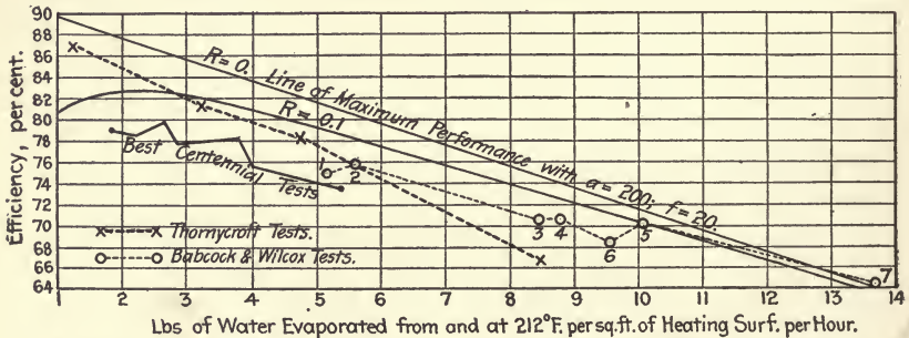
FIG. 121.—THORNYCROFT AND BABCOCK & WILCOX TESTS COMPARED.
