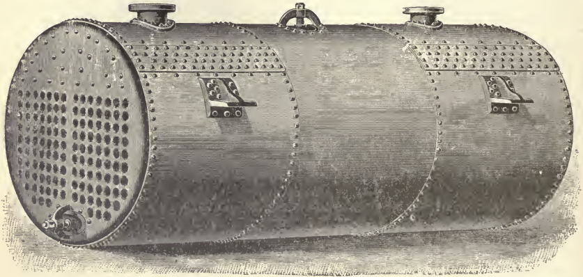
FIG. 61.—HORIZONTAL RETURN TUBULAR BOILER.
