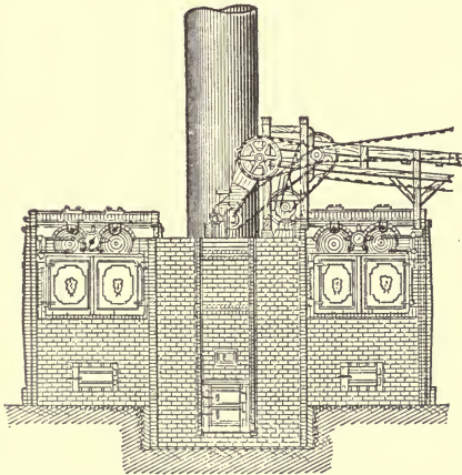
FIG. 40a.—BAGASSE FURNACE, END VIEW.
