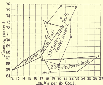
FIG. 119.—SPENCE'S EXPERIMENTS.
