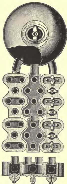
FIG. 95 — HEADERS OF THE GILL BOILER.
