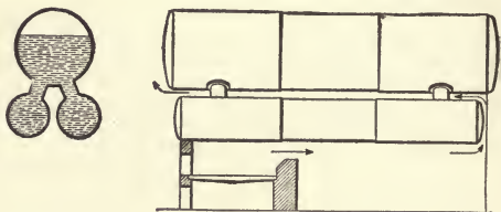
FIG. 56.—THE "ELEPHANT" BOILER.
