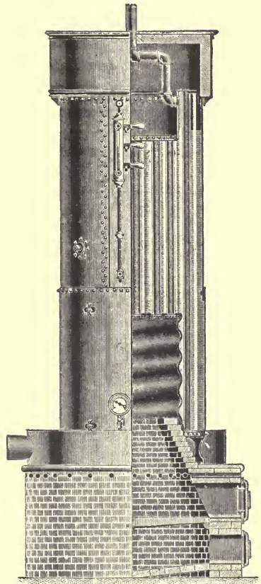
FIG. 64.—THE WEBBER VERTICAL BOILER.
