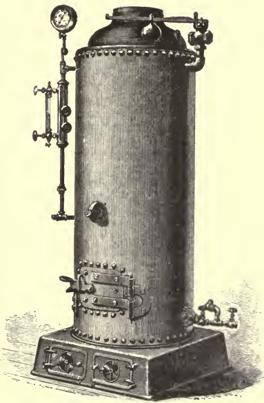
FIG. 63.—THE VERTICAL TUBULAR BOILER.
