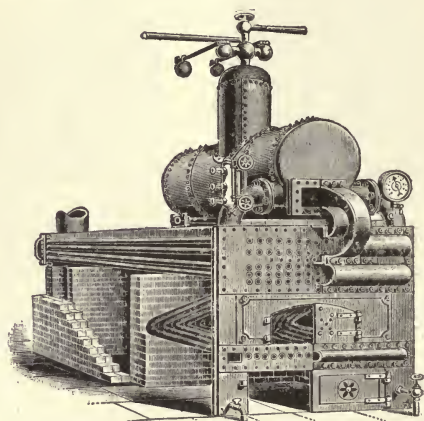
FIG. 82.—PHLEGER, 1871.
