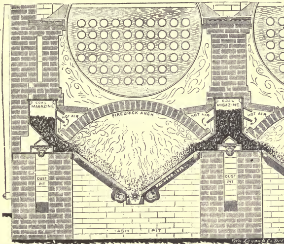
FIG. 29.—THE MURPHY AUTOMATIC FURNACE.
