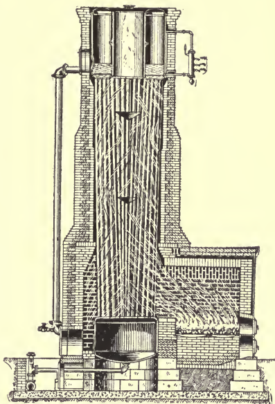
FIG. 200.—THE CAHALL VERTICAL BOILER.
