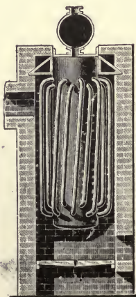
FIG. 83.—ROGERS & BLACK, 1876.
