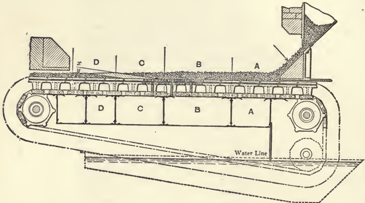
FIG. 23.—THE COXE AUTOMATIC STOKER.
