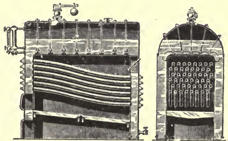
FIG. 80.—WILCOX, 1856.
