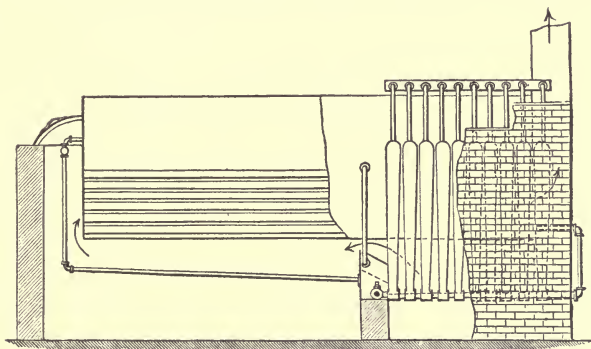
FIG. 125.—THE SMITH BOILER.
