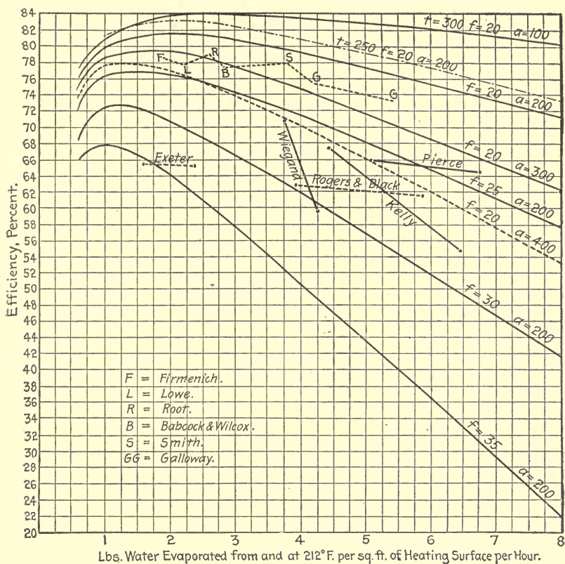
FIG. 49.—CURVES OF CALCULATED EFFICIENCIES FOR DIFFERENT RATES OF DRIVING, for K = 14,800 , R = 0.1 , t = 300 (except one curve, t = 250 ) f = 20 to 35, a = 100 to 400.
