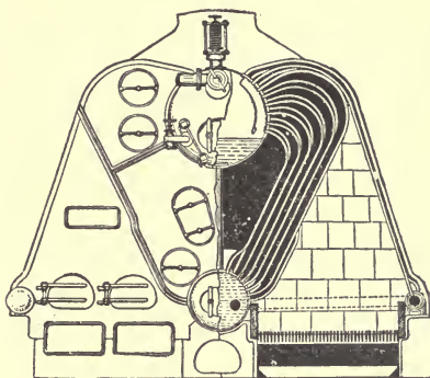
FIG. 104.—THORNYCROFT BOILER.
