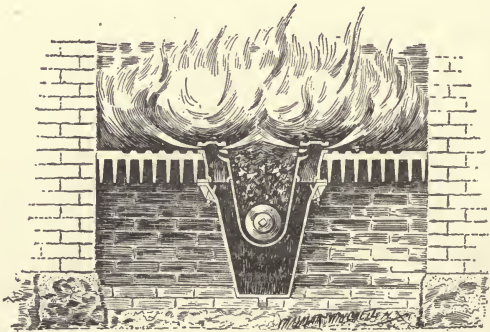
FIG. 31.—THE AMERICAN STOKER.
