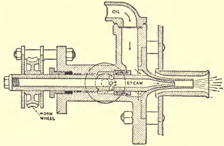
FIG. 40.—THE URQUHART OIL-BURNER.
