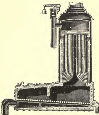
FIG. 79.—CHURCH, 1832.
