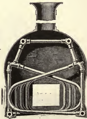
FIG. 84.—DANCE, 1833.
