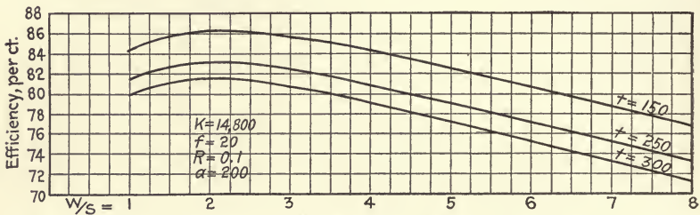
FIG. 51.—EFFECT OF STEAM-PRESSURE UPON EFFICIENCY.
