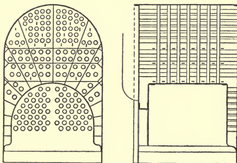
FIG. 126.—THE ANDREWS BOILER.
