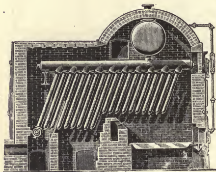
FIG. 74.—ALLEN, 1871.
