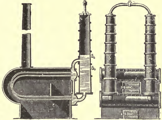
FIG. 78.—GURNEY, 1826.
