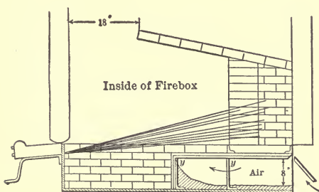
FIG. 38.—PETROLEUM FURNACE.
