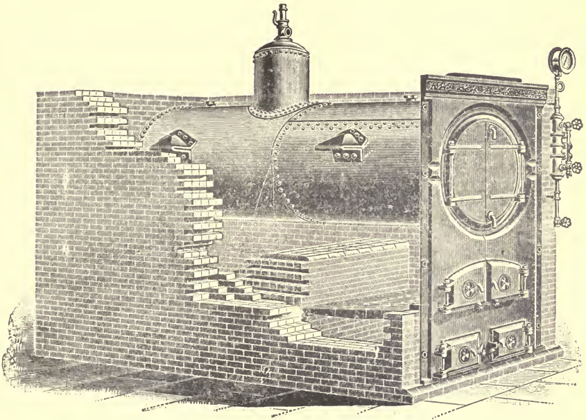
FIG. 62.—RETURN TUBULAR BOILER WITH SETTING.
