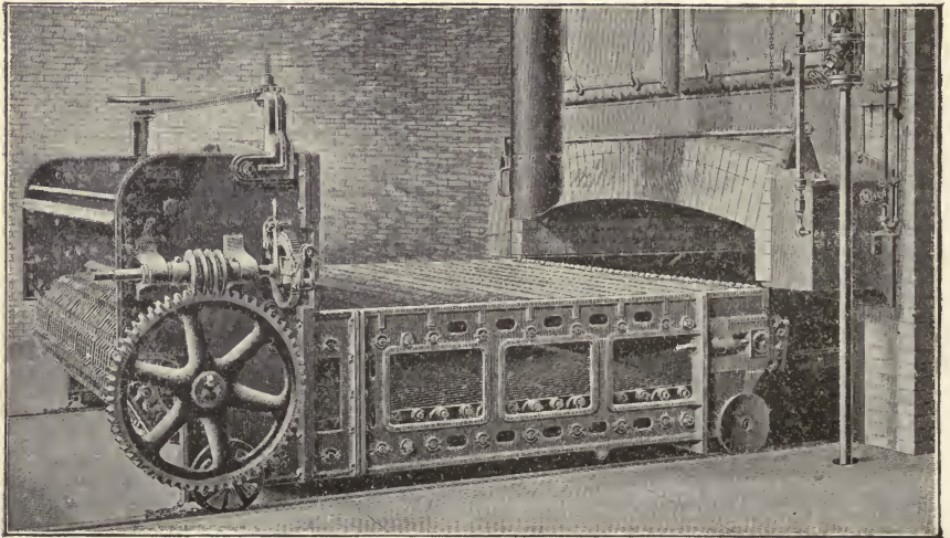
FIG. 25.—THE BABCOCK & WILCOX STOKER.
