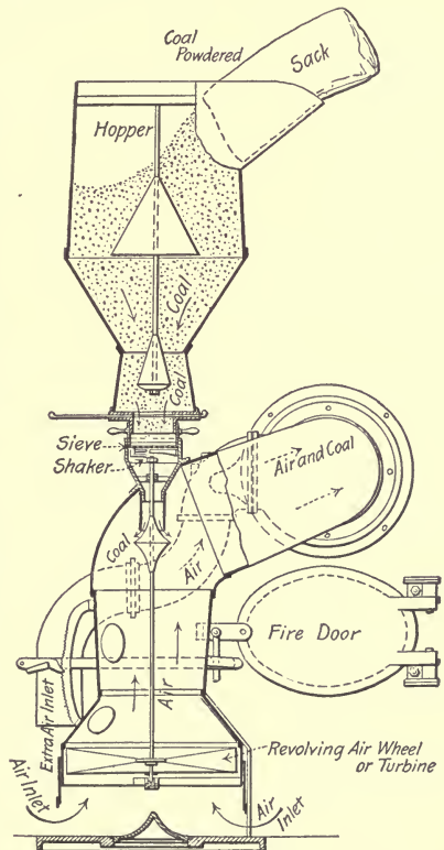
FIG. 36 —WEGENER'S POWDERED COAL APPARATUS.
