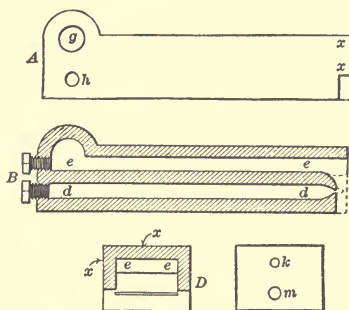
FIG. 39.—OIL-BURNER.
