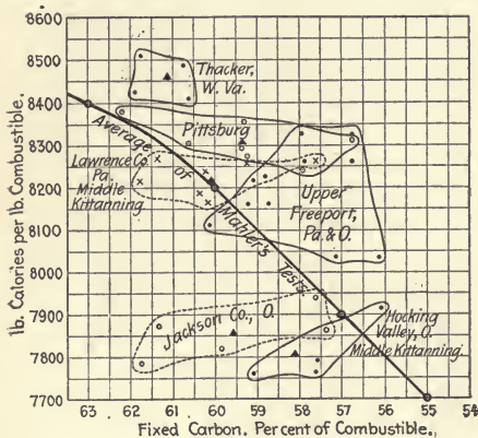
FIG. 7.—RELATION OF HEATING VALUE TO PER CENT OF FIXED CARBON. (Tests of Profs. Lord and Haas.)
