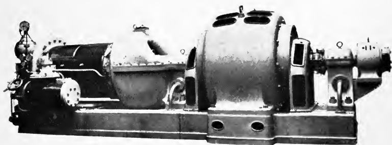
PLATE 18C.—Brush & Parsons' Turbine directly connected to Alternator and its Excitor.
