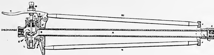
FIG. 127.—Sectional view of the Brooke Steam Trap. A is the Steam Pipe to be drained; E is the Valve, which is opened and closed by the lever D , actuated by the expansion and contraction of A .
