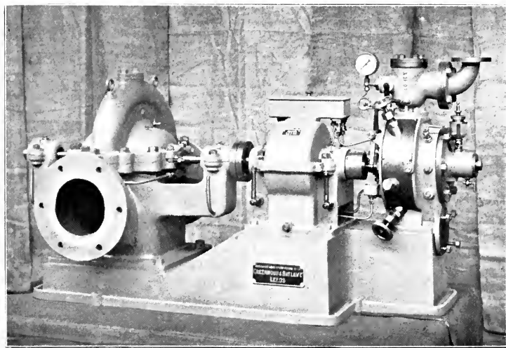
PLATE 21B.—De Laval Turbine directly connected to a De Laval 15 Horse-power Turbine Pump. [To face p. 304.]
