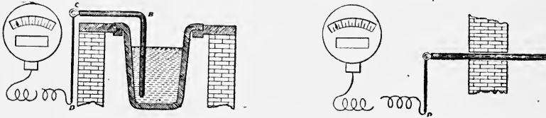
FIG. 4.—Bristol's Thermo-Electric Pyrometer as arranged for taking the Temperature of a Bath of Metal, or a Furnace or Flue.
