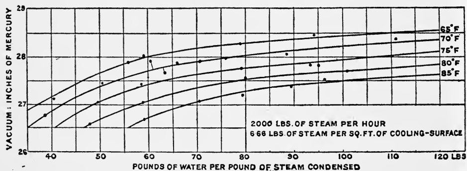
Figs. 174 and 175.—Curves showing the different quantities of Circulating Water, with different Initial Temperatures and different Vacua, in Mr. Richard Allen's experiments. ( Trans. Inst. C.E. )
