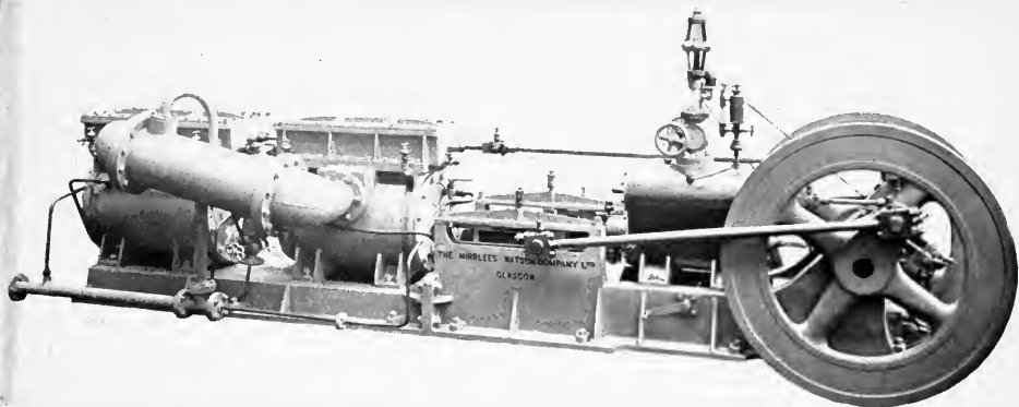
PLATE 26A.—Two-stage Horizontal Steam-driven Slide-valve Dry-air Pump, by the Mirrlees Watson Co., specially designed for high vacua.
