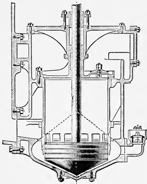
FIG. 182.—Section of Edwards Air Pump, showing the Form of the Piston.
