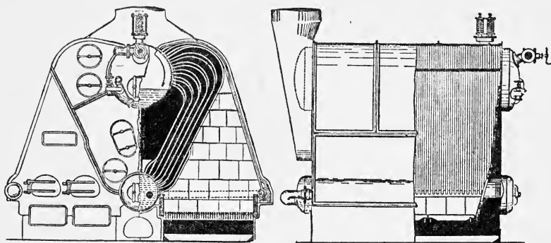
FIG. 18.—Transverse and Longitudinal Sections of the Thornycroft Water-tube Boiler, "Daring" type.
