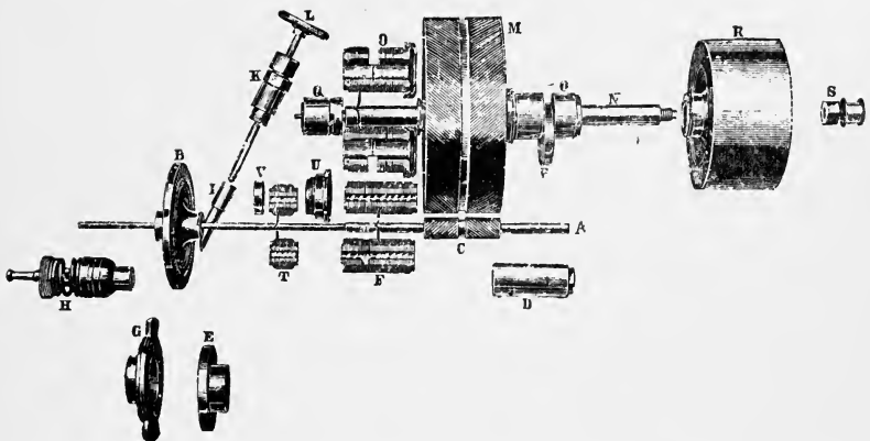
FIG. 144.—Parts of the De Laval Turbine. B is the Turbine Wheel; I the Nozzle; A the Shaft; M Gear Wheel, etc.
