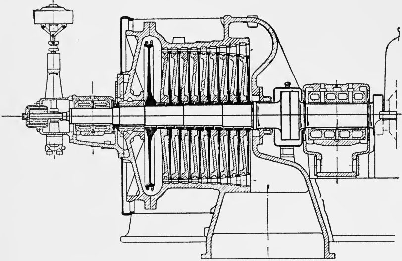
FIG. 150.—Section of one Form of the A.E.G. Steam Turbine.
