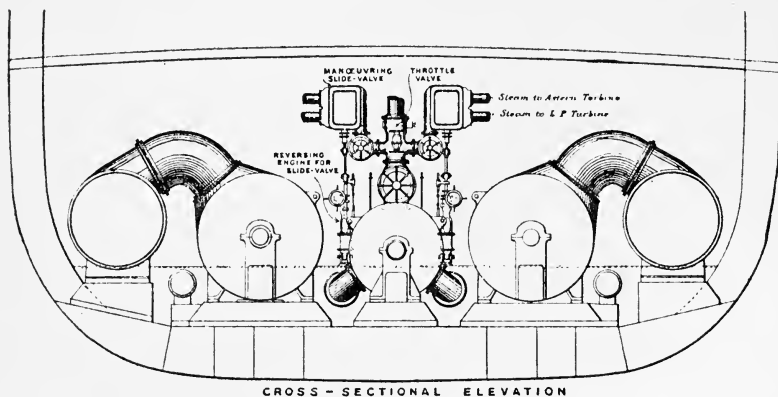
CROSS-SECTIONAL ELEVATION
