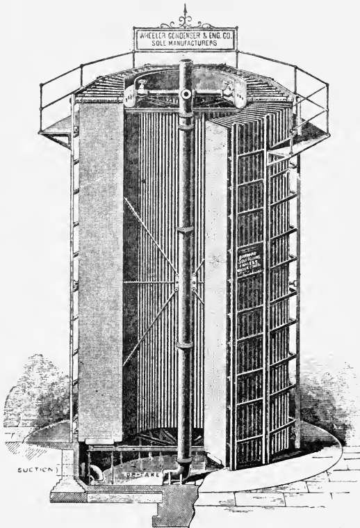
FIG. 187.—Another form of Barnard Chimney Cooling Tower. The Air passes up through the Centre and out at the Sides, the Water trickling over the Mats, which are arranged radially round the Centre.
