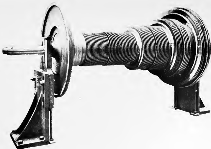
PLATE 18A.—Rotor of Brush and Parsons' Steam Turbine.
