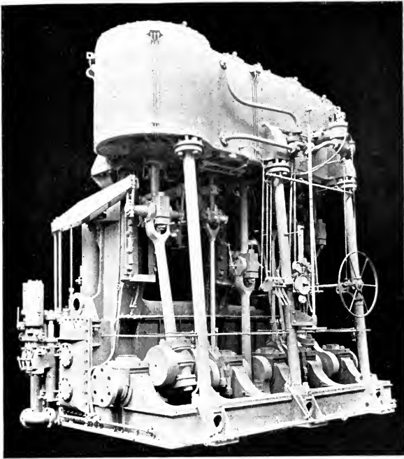
PLATE 15A.—Triple Expansion Marine Engine, made by the Central Engineering Works, Hartlepool.
