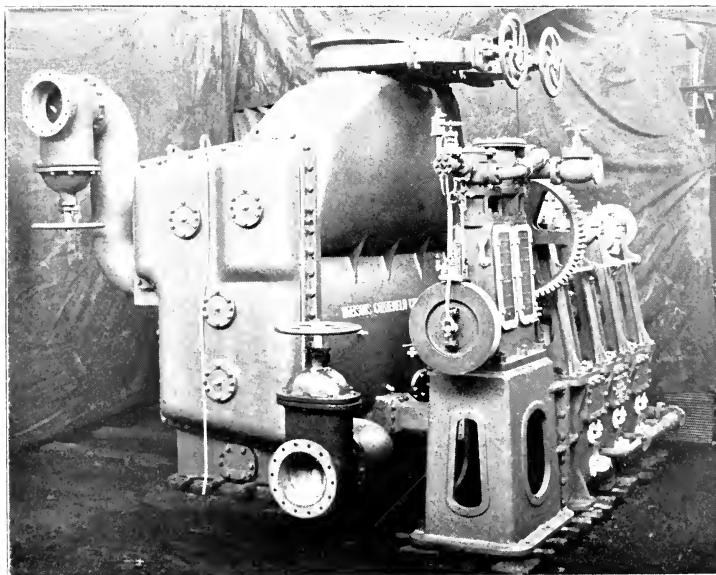
PLATE 23B.—Contraflo Condenser, with Air Pump. [To face p. 328.
