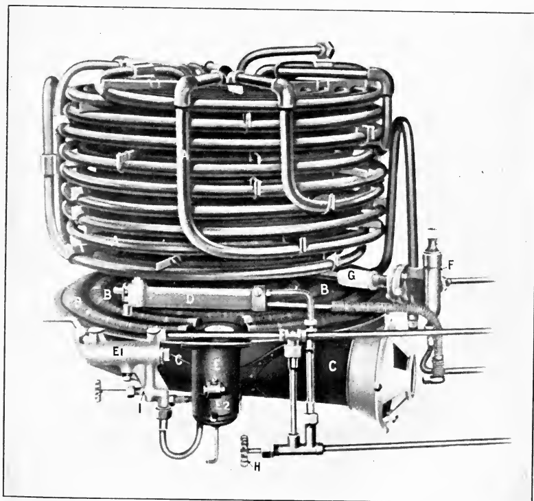
PLATE 6B.—Boiler used in the White Steam Cars. The water circulates through the Tubes, heat being supplied by the Petrol Burner shown below.
