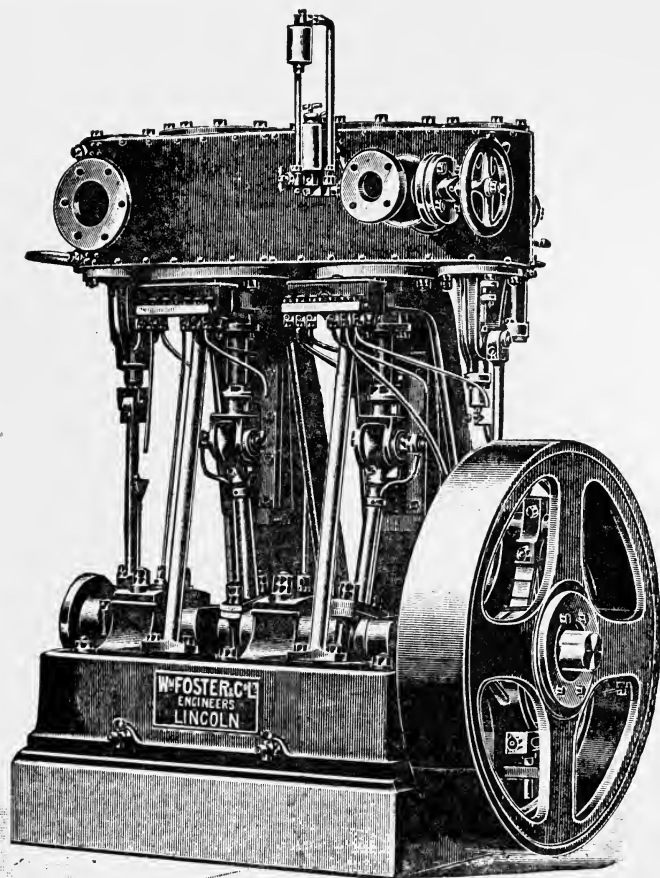
FIG. 93.—Compound Vertical Engine, unenclosed, with Shaft Governor.
