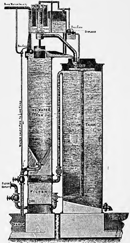
FIG. 68.—Section of Criton Water Softener. The Syphon Tank which receives the Water to be softened is seen at the top, where the Soda Tank is also fixed, the Lime-water Tank and the Filter and Settling Tank being below.
