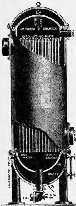
FIG. 56.—The Riblet Steam-feed Water Heater. The Water passes through the Tubes and the Steam on the outside.
