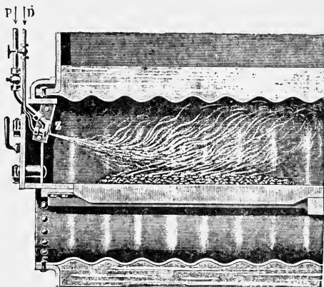
FIG. 27.—Shows its application to a Lancashire Boiler.
