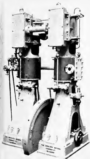
PLATE 26B.—Two-throw Steam-driven Slide-valve Dry-air Pumps, made by Mirrlees Watson Co. The Air Pumps are seen above the Steam Cylinders.
