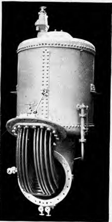
PLATE 10A.—Evaporator made by the Central Engineering Works, Hartlepool.
