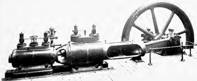
PLATE 13C.—Marshall's Horizontal Tandem Compound Engine, with Trip-gear Valves. [To face p. 224.]
