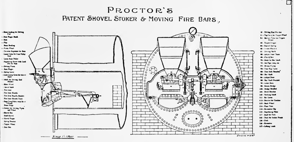
Fig. 30.—Longitudinal and Transverse Section of Lancashire Boiler fitted with Proctor's Shovel Mechanical Stoker. The Coal is fed from the Hoppers into the Boxes below, and is thence ejected on to the Fire Bars by the action of the Swing Shovel.
