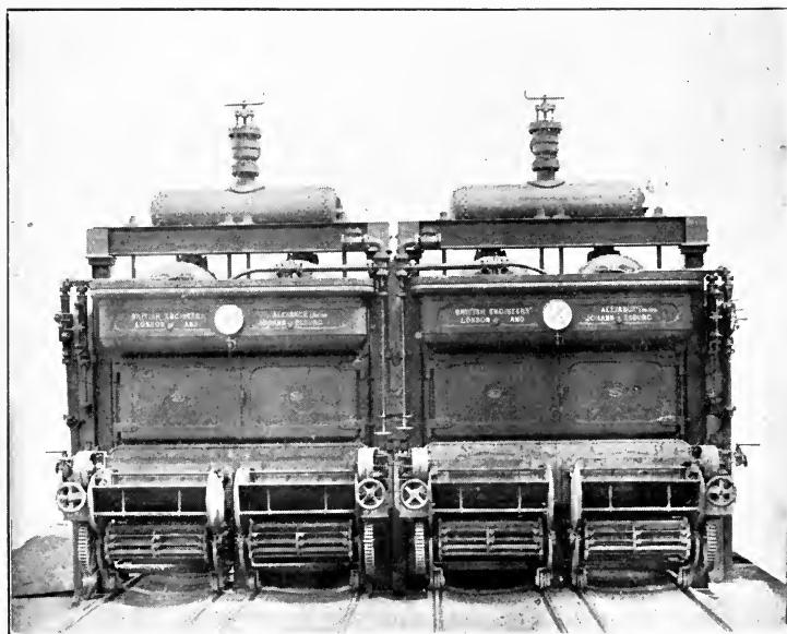
PLATE 7B.—A Pair of Water Tube Boilers, with Chain Grate Stokers. [To face p. 112.]
