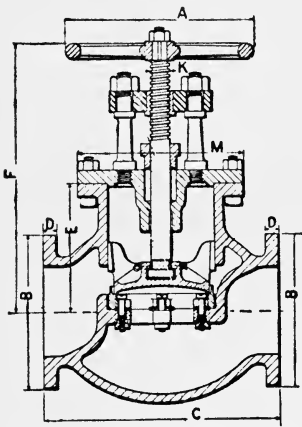
FIG. 109.—Section of a Stop Valve made by Messrs. Alley & Maclellan. The moving portion is of the equilibrium type. Steam passes from one side of the Valve to the other when the moving member is raised.
