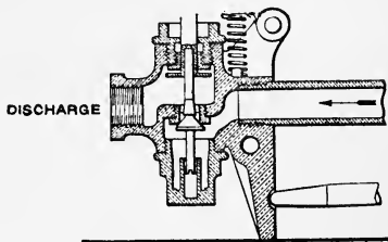
FIG. 128.—Section of Discharge End of Brooke's Steam Trap. Steam enters by the Pipe shown, in the direction of the Arrow, and when Water also enters, the cooling effect contracting the Steam Pipe actuates the Levers operating the Valve shown, opening it, the reverse operation closing it.
