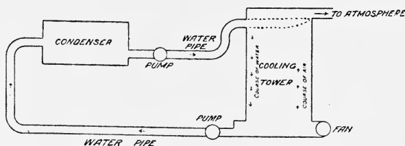
FIG. 183.—Diagram showing the Course of the Water when a Cooling Tower is used, in connection with a Condenser.
