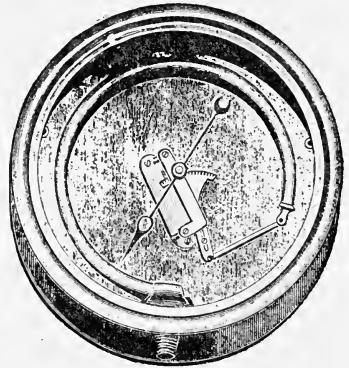
FIG. 47.—The Steam Gauge shown in Fig. 46, with Dial removed, showing the Tube upon which the Steam acts and the Gearing giving motion to the Pointer.
