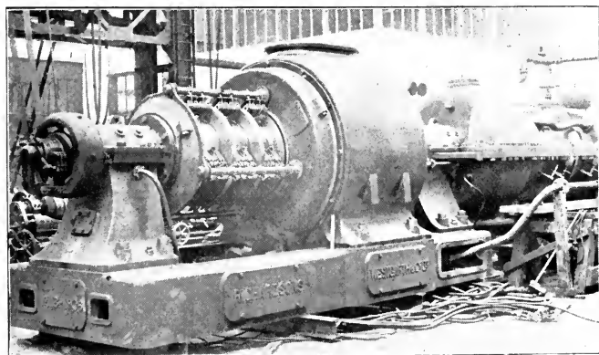
PLATE 19C.—Richardson's, Westgarth's, and Parsons' Steam Turbine directly connected to a Tube, whose Alternator and its Excitor are seen from the Generator end. [To face p. 288.]
