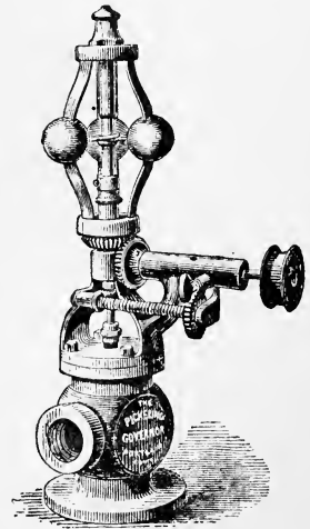
FIG. 116.—Pickering Governor.
