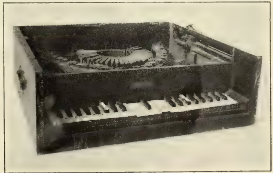
AN EARLY FORM OF TYPE-WRITER, HAVING THE PIANO KEYBOARD.
