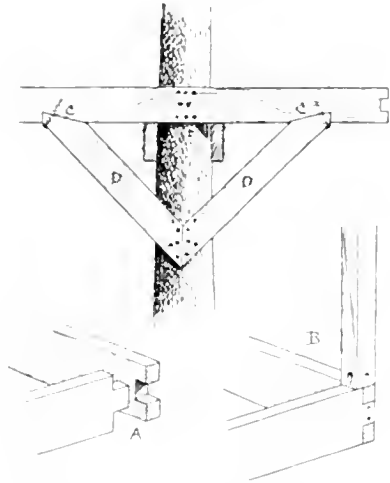
FIG. 5. DETAILS OF FRAMING OF THE BRACKET.
