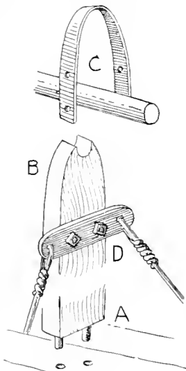
FIG. 2. DETAILS OF FLOOR HORIZONTAL BAR.
