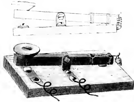
FIG. 28. A TELEGRAPH-KEY.
