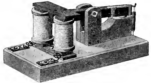
FIG. 33. A TELEGRAPH-SOUNDER.
