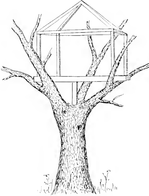
FIG. 9. DETAILS OF FRAMING OF A LOW SINGLE-TREE HOUSE.
