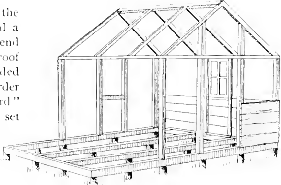
FIG. 9. SHOWING THE FRAMING OF THE HOUSE-ENT.
