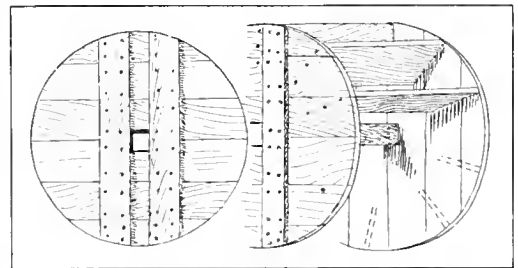
FIG. 12. DETAILS OF WHEEL SHOWN ON OPPOSITE PAGE.
