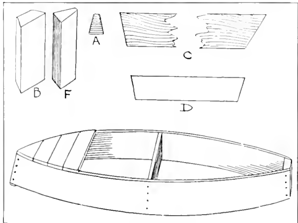
FIG. 2. DETAILS OF A DOUBLE-ENDED SHARPIE.
