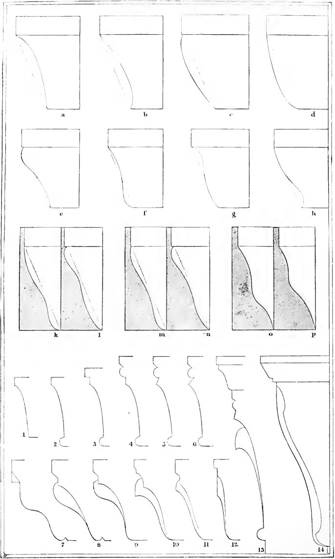
PLATE XV.—CORNICIE PROFILES.
