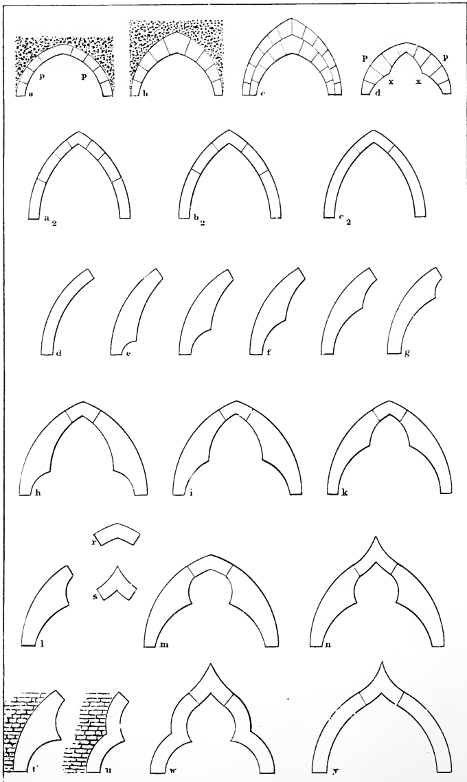
PLATE III.—ARCH MASONRY.
