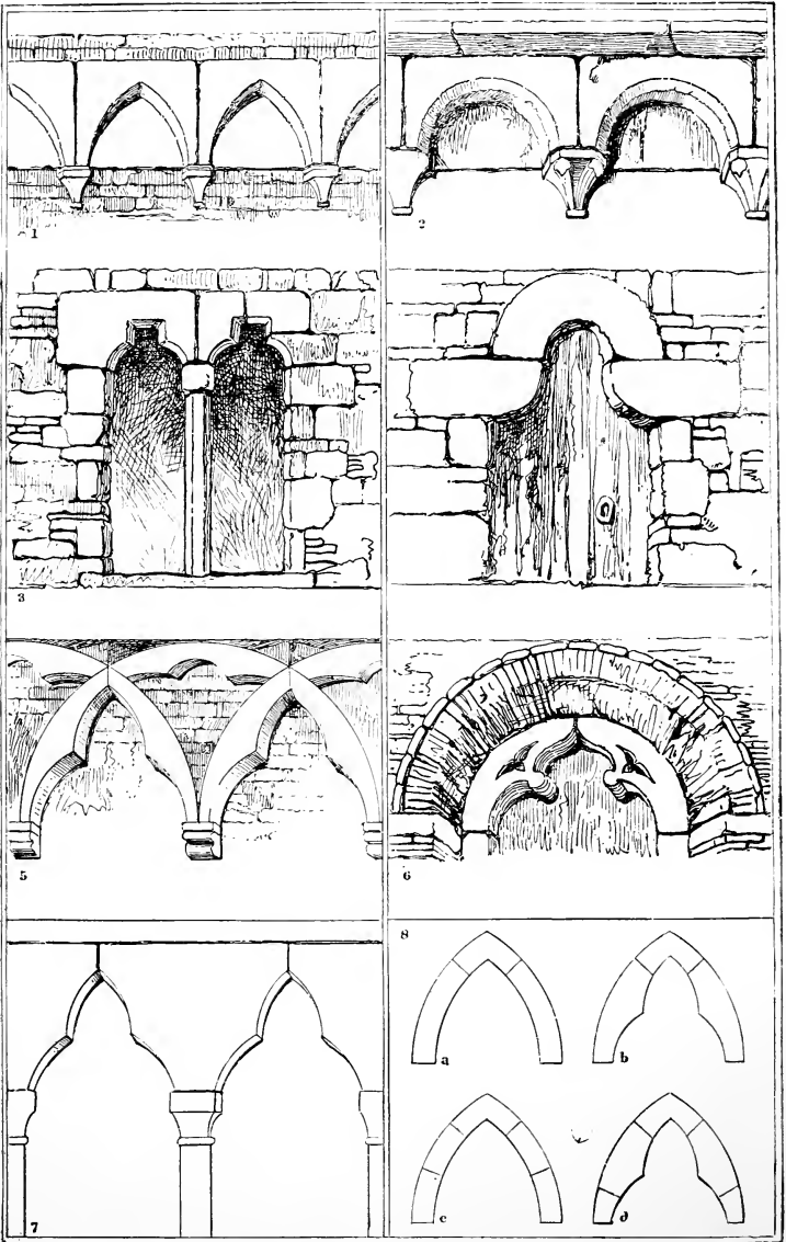
PLATE IV.—ARCH MASONRY.
