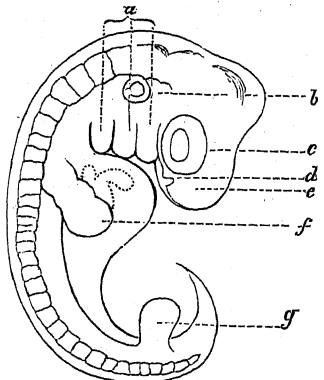
FIG. 76.—Tortoise. (4 weeks).
