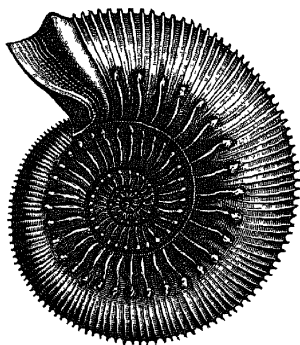
FIG. 18.—Ammonite.
