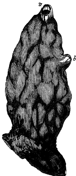
FIG. 54. Sea-squirt.
