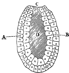
FIG. 68.—Gastrula Stage.
