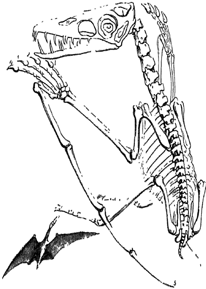
FIG. 16. - Pterodactyl (Wing-finger).
