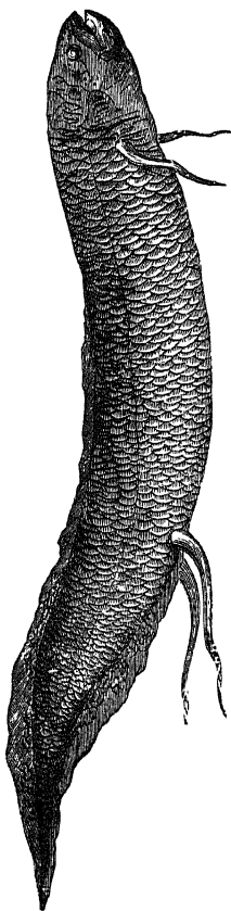
FIG. 57.—Mud-fish.
