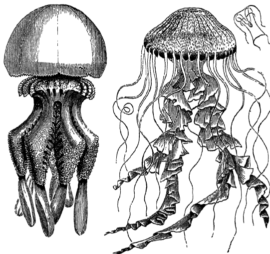
FIG. 40.—Jelly-fish.
