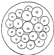
FIG. 67.—Morula Stage.
