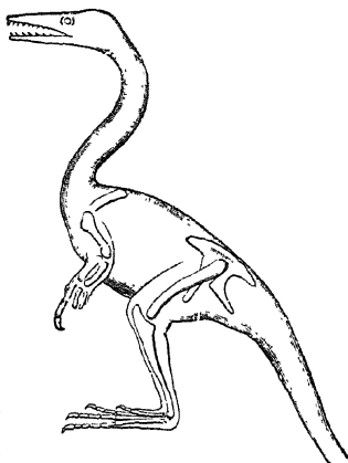
FIG. 78.— Compsognathus .
