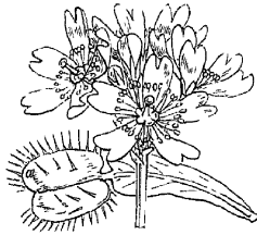
FIG. 26.—Venus's Fly-trap
