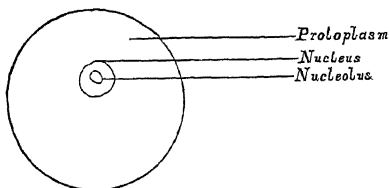
FIG. 65.—Cell.
