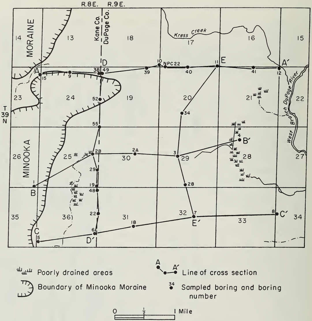
Fig. 2 - NAL site showing main physical features, location of borings used for stratigraphic control in this study, and lines of cross sections.
