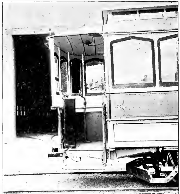
SIDE VIEW—COLUMBUS VESTIBULE.
