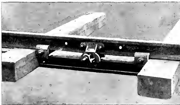
JOINT SUGGESTED BY MR. ANTHONY.
