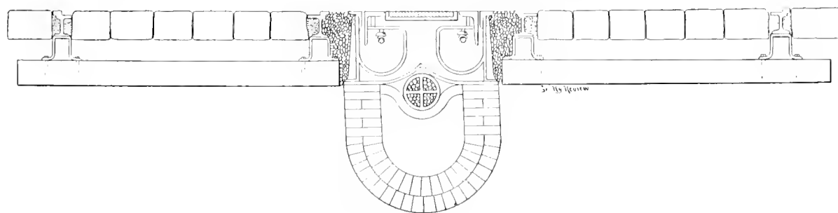
CROSS SECTION—HIEATZMAN CONDUIT SYSTEM.
