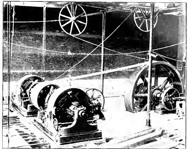
ONE ROPE DRIVE UNIT—CHICAGO CITY RAILWAY.
