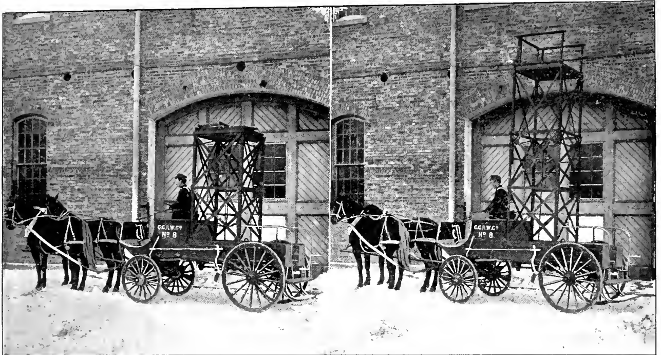
THE COMBINED TOWER AND WRECKING WAGON.
