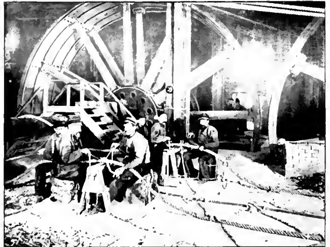
SPLICING THE TRANSMISSION ROPES.
