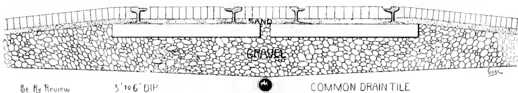
DOUBLE TRACK DRAIN CONSTRUCTION.
