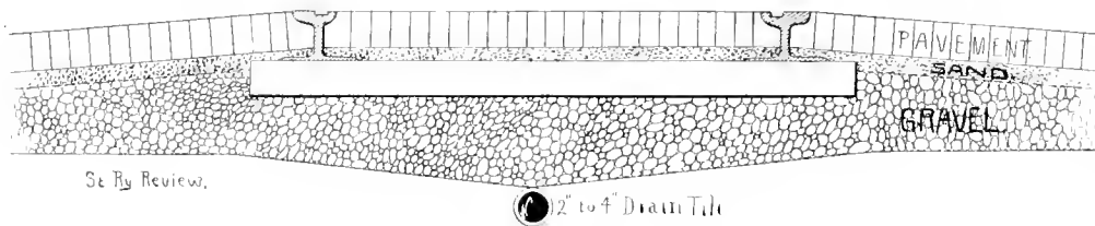
SINGLE TRACK DRAIN CONSTRUCTION.
