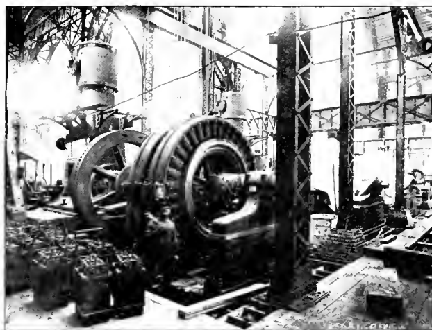
WESTINGHOUSE GENERATOR—MACHINERY HALL.
