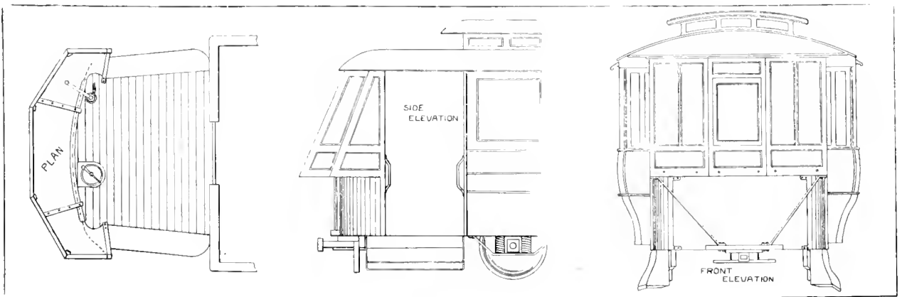
ANOTHER VESTIBULE PLAN.
