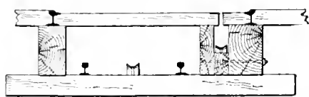
SECTION OF CONDUITS FOR COUNTERWEIGHTS—SEATTLE.
