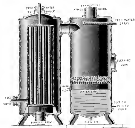
BASS WATER HEATER AND PURIFIER.
