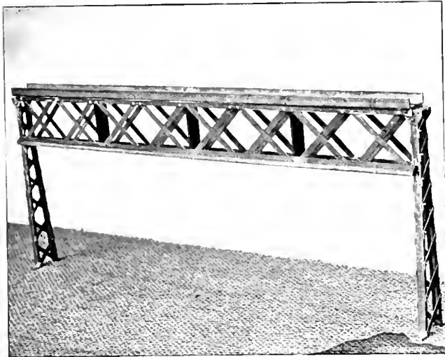
LATTICE GIRDER CONSTRUCTION.
