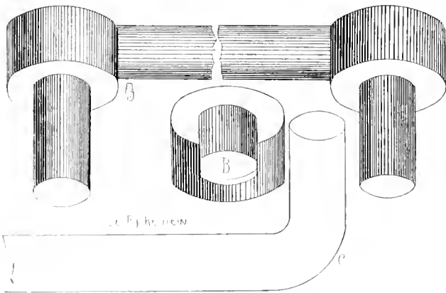
RAIL BONDING AT LA CROSSE.
