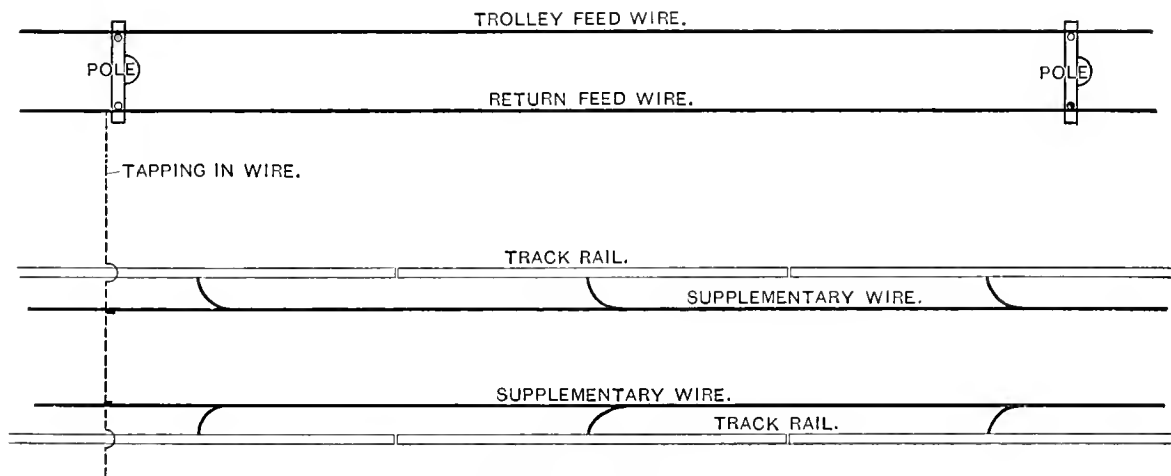
DIAGRAM OF WASON'S METHOD.
