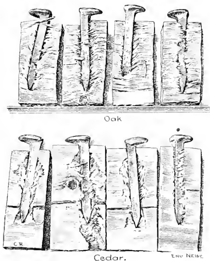
F. Railroad, in Kansas, showing the effects of spikes driven into oak ties and cedar ties.
