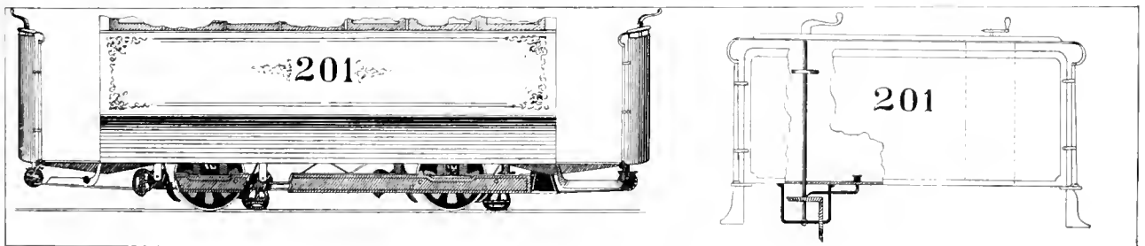
THE BRANDAU TRACK AND WHEEL BRAKE.
