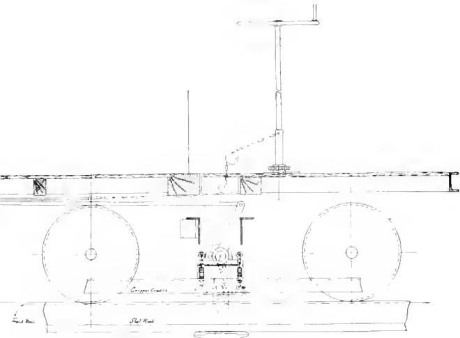
SIDE ELEVATION—SLOT RAIL BRAKE.
