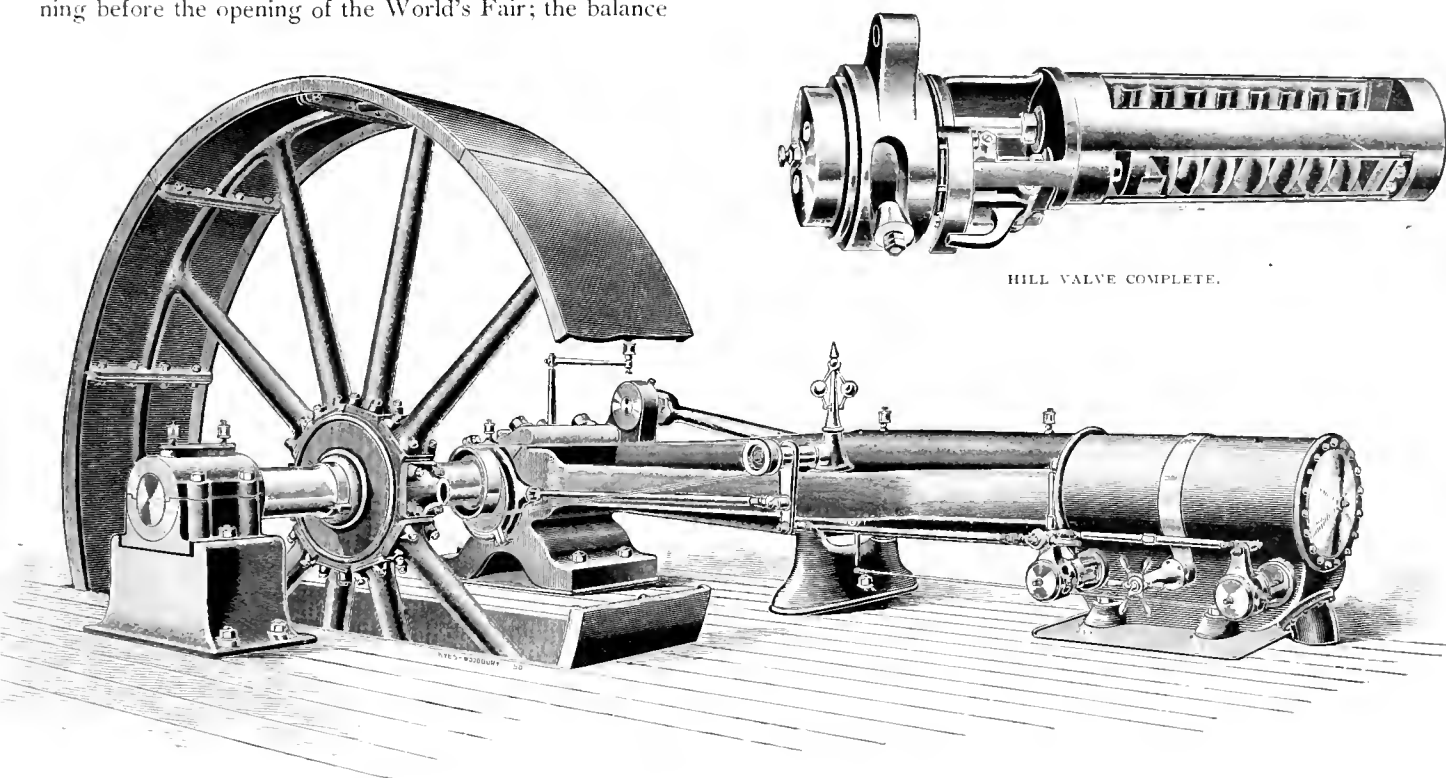
IMPROVED WHEELLOCK ENGINE, WITH HILL VALVE GEAR—CHICAGO CITY RAILWAY.
