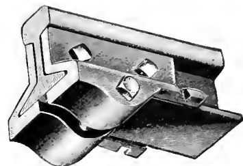
CROSS SECTION STEVER JOINT, WITH TEE RAIL.
