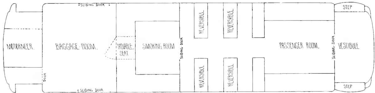
PLAN OF COMBINATION BAGGAGE, SMOKING AND PASSENGER CAR.
