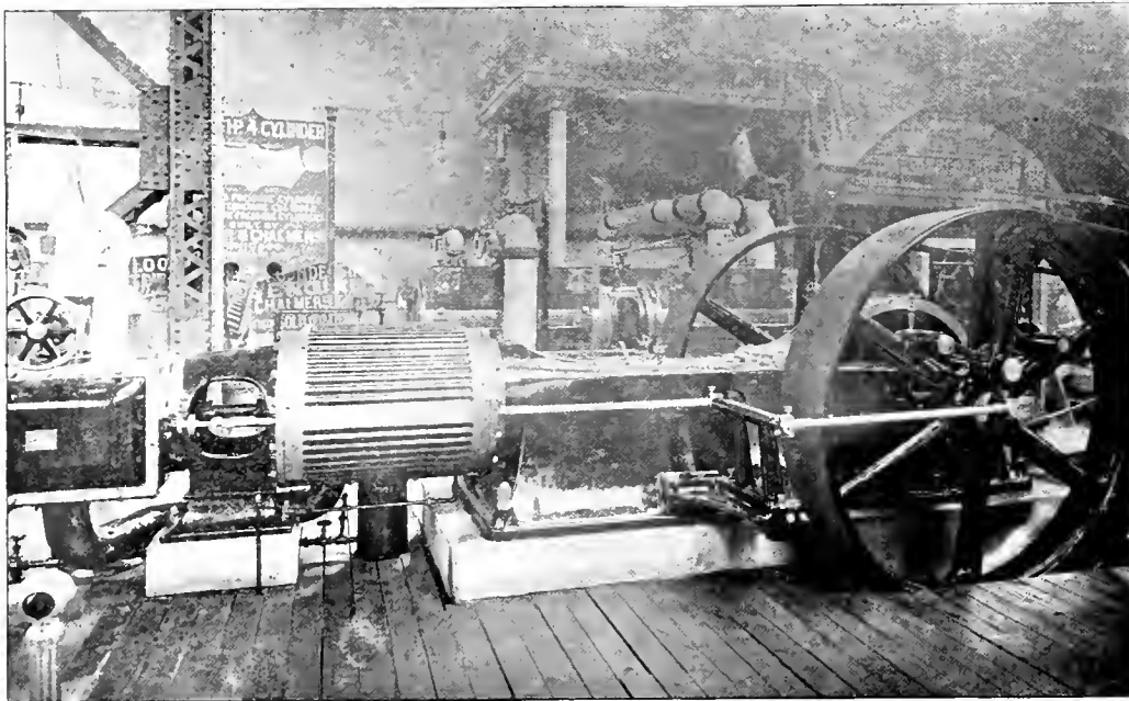
MCEWEN ENGINE AT WORLD'S FAIR.
