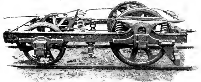
BALTIMORE NEW PIVOTAL TRUCK.
