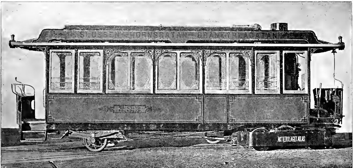
SIDE VIEW STEAM MOTOR USED AT STOCKHOLM, SWEDEN.
