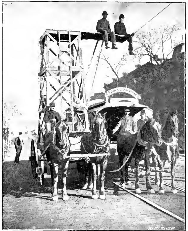
NEW TOWER WAGON—MONTREAL.
