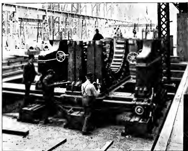
ERECTING WESTINGHOUSE GENERATOR—MACHINERY HALL.
