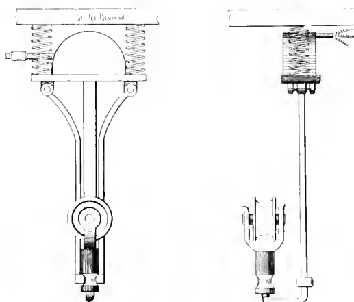
SIDE VIEW.—THE UNDERGROUND TROLLEY.—END VIEW.
