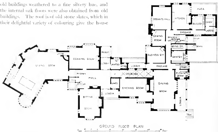
GROUND FLOOR PLAN OF STOKES BARN, FULMER
