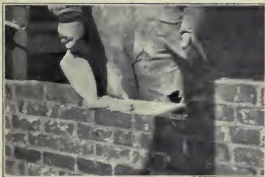
Fig. 24. — Spreading mortar on exterior face tier.
