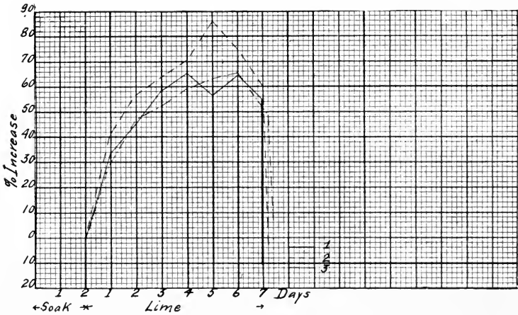
EXPERIMENT 39.—WEIGHT. Per cent. increase on 48-hour soaked weight.
