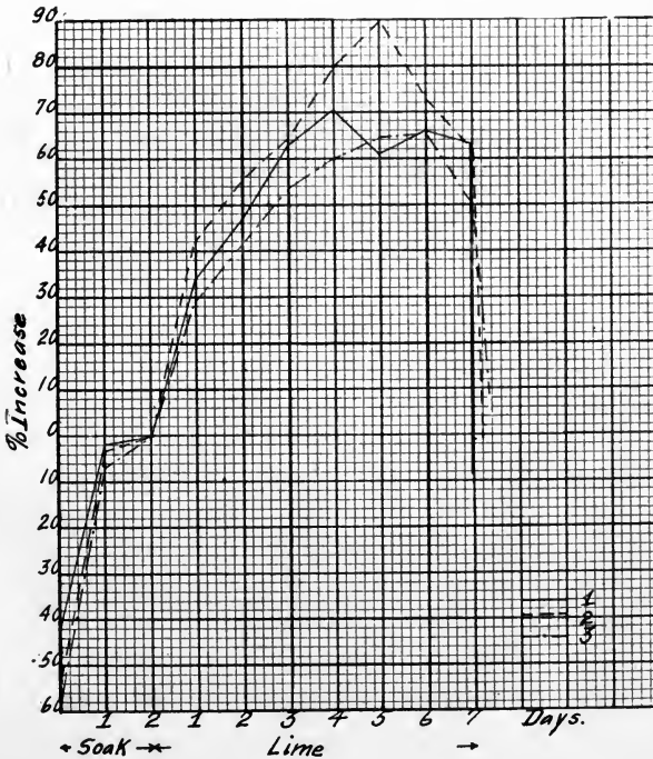
EXPERIMENT 39.—VOLUME. Per cent. increase on 48-hour soaked volume.
