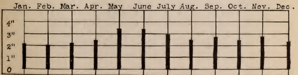
Fig. 11. Average monthly precipitation by sections.
