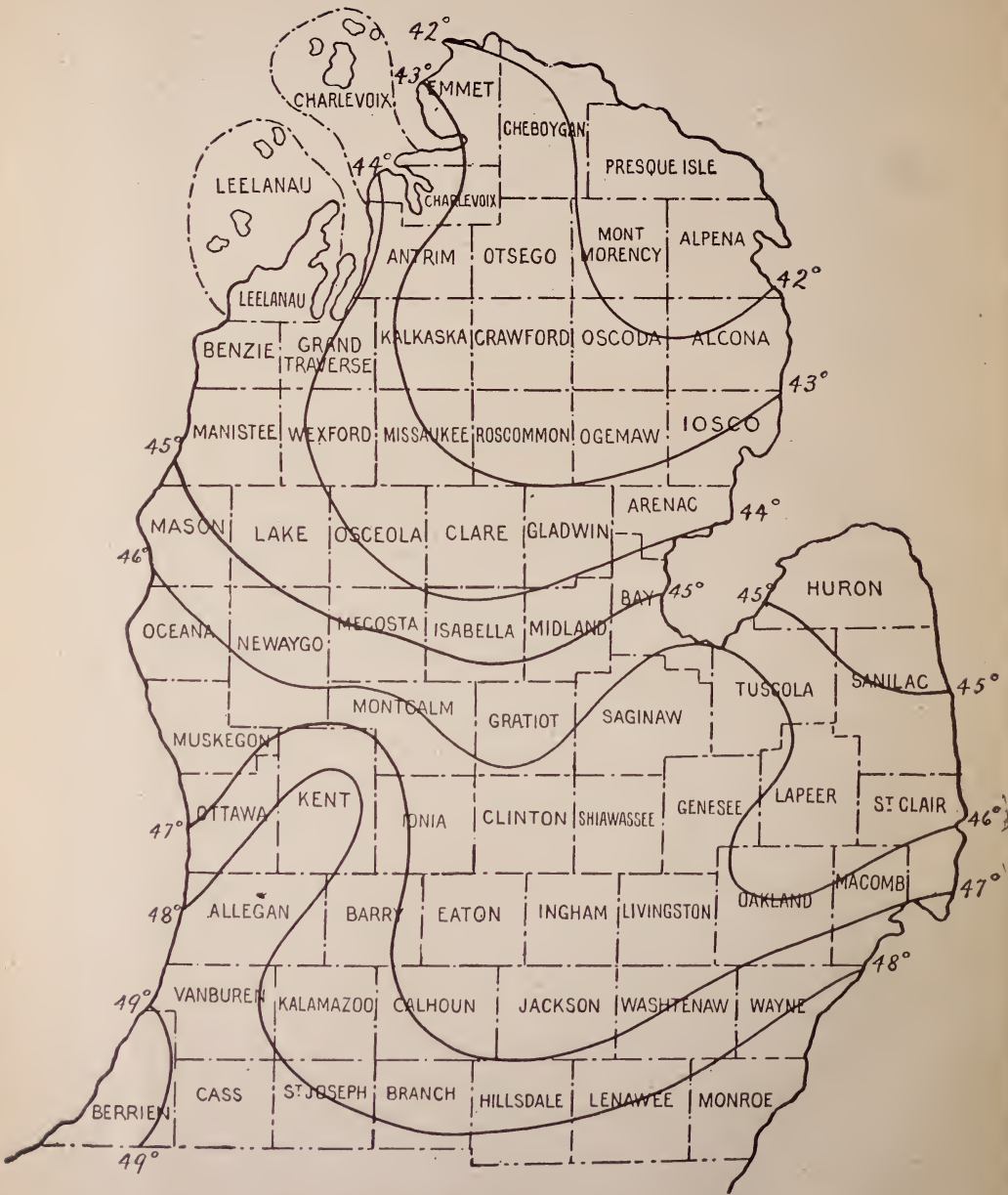
Fig. 2. Annual mean temperature, 1886 to 1911.
