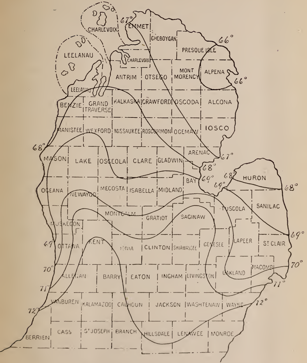
Fig. 2. July mean temperature, 1886 to 1911.
