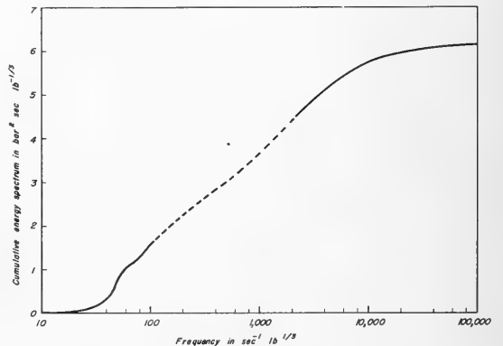
Fig. 7. Cumulative energy spectrum.
