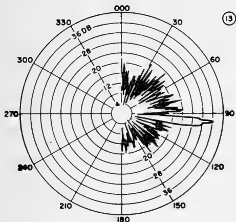
Fig. 4A. Signal from 20-foot Projector Hydrophone at 100 feet Range 12,450 yards.
