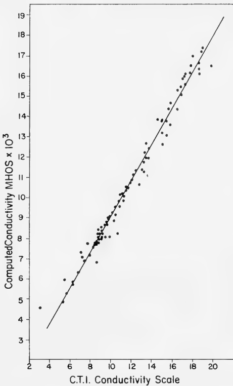
Fig. 3. CTI field calibration. Computed conductivity obtained by using titration chlorinity results, CTI temperature, in the Thomas, Thompson, and Utterback interpolation formulas. Data obtained over several months period during winter of 1951-52.
