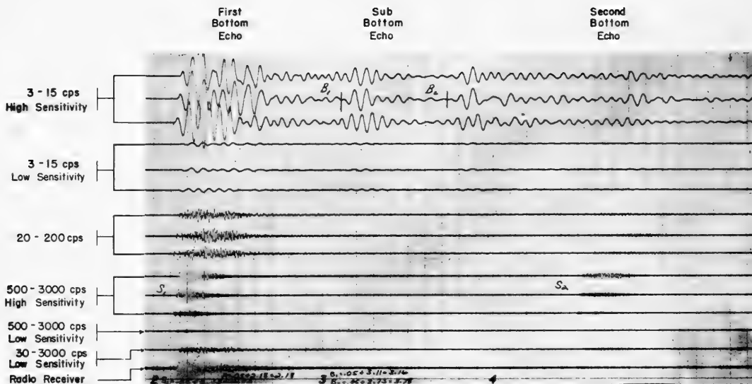
Fig. 17. Oscillogram of Bottom Echo in San Nicolas Basin.
