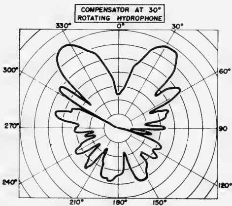
Fig. 3C. 10-foot Line Hydrophone with Compensator at 2.5 kc.
