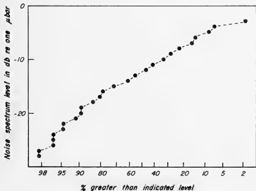
Fig. 15. Cumulative distribution of low-frequency noise spectrum levels observed in the North Equatorial Pacific.
