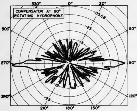
Fig. 2A. 10-foot Line Hydrophone with Compensator at 8 kc.
