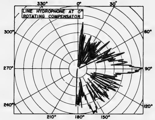
Fig. 2B. 10-foot Line Hydrophone with Compensator at 8 kc.
