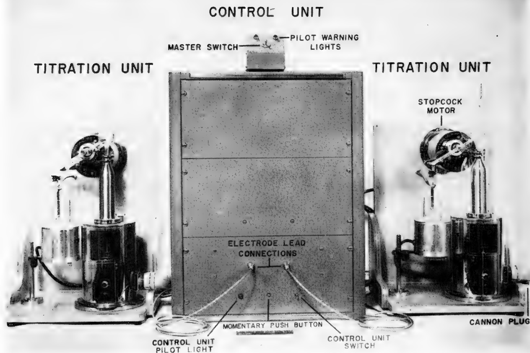
Fig. 5. The Automatic Chlorinity Titrator (ACT-I)
