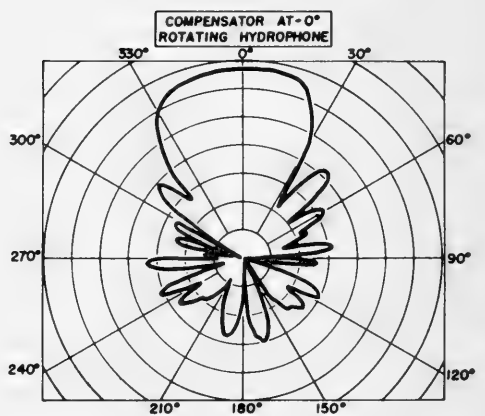
Fig. 3D. 10-foot Line Hydrophone with Compensator at 2.5 kc.
