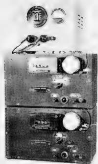
Fig. 1. Conductivity Temperature Indicator (CTI). A. Deck-side units. Top unit contains constant voltage transformer, and meters for monitoring voltage and frequency of supply to instruments. Center unit, temperature indicator. Bottom unit, Conductivity indicator. Dials read temperature in degrees centigrade and conductivity in millimhos, respectively. Circular unit to right of dials contain indicating dehydrating agent. Middle, four position switch on each unit has three calibrate positions and a "normal use" position. Bottom row of controls are, right to left, fuse, power switch, power indicator light, and switch to turn the balancing motor on and off while keeping unit energized.
