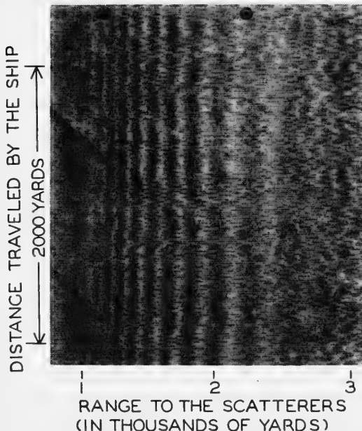
Fig. 1. Chemical recorder trace showing interference patterns resulting from scattering layer.
