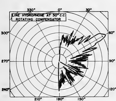
Fig. 2C. 10-foot Line Hydrophone with Compensator at 8 kc.
