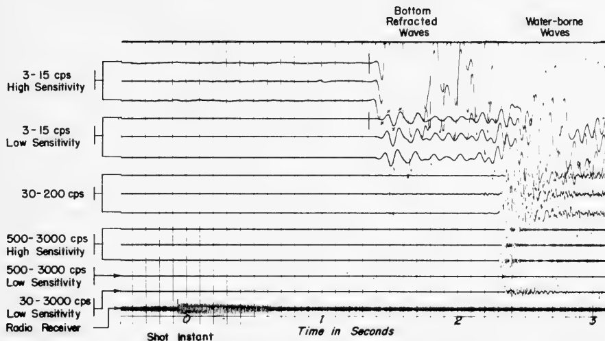
COMPLETE RECORD OF A 1-LB CHARGE, 40 KM DISTANCE Bikini Lagoon
