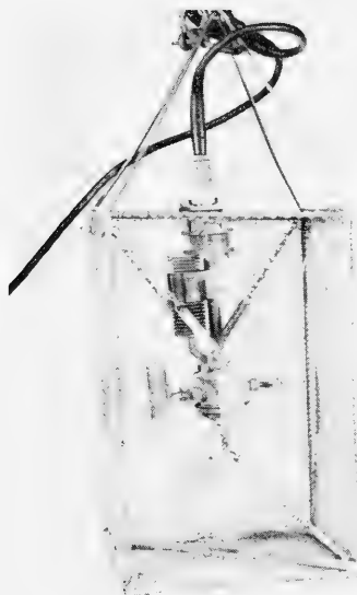
Fig. 1. B. Underwater head. Sensing elements and junction box suspended on eight springs. Portion protruding through top of cage is water proof connector for MCOS-6 cable. Entire unit below water proof connector is oil filled, bellows on left prevent pressure differential across case. Conductivity cell on right, resistance thermometer on leucite web on left.
