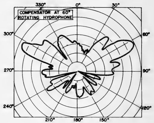
Fig. 3B. 10-foot Line Hydrophone with Compensator at 2.5 kc.
