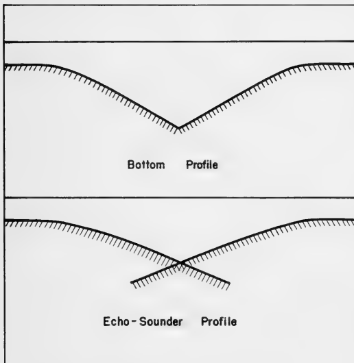
Fig. 1. Echogram of V-shaped bottom trench.
