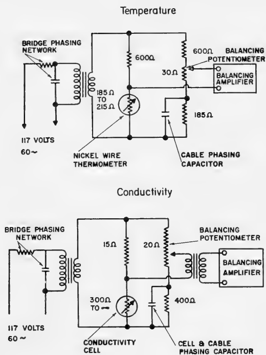
Fig. 2. Schematic equivalent circuits of CTI temperature and conductivity units. Commercial components have been used where possible.
