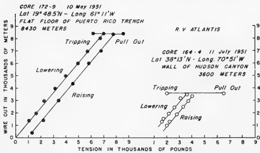
Fig. 4. Typical plot of wire tension during coring.
