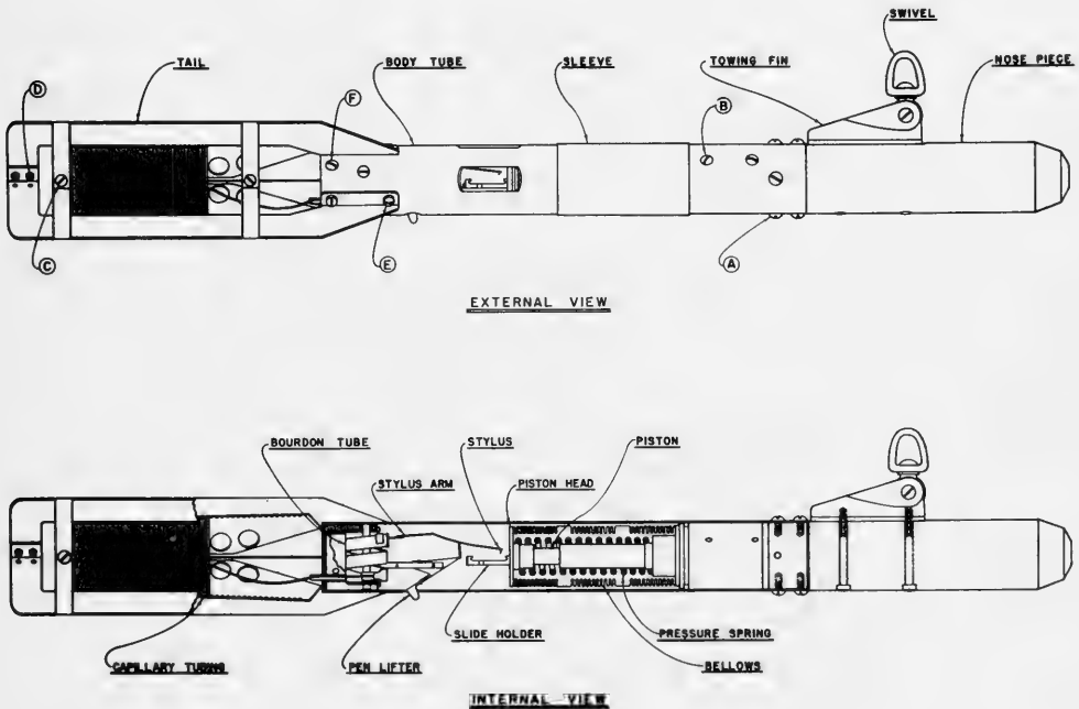
Fig. 1. The Bathythermograph
