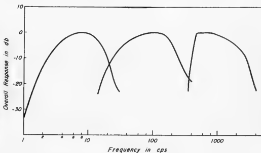
Fig. 11. Frequency response of recording system.
