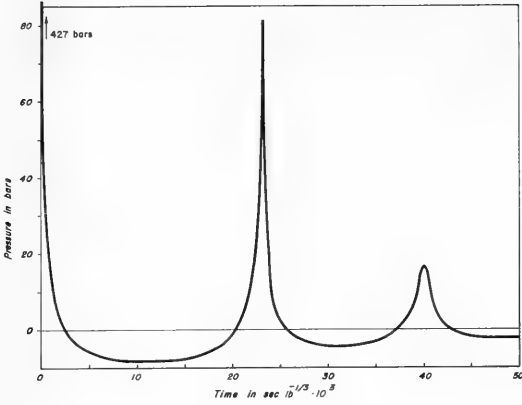
Fig. 4. Pressure-time curve of a TNT explosion at 500 feet depth.
