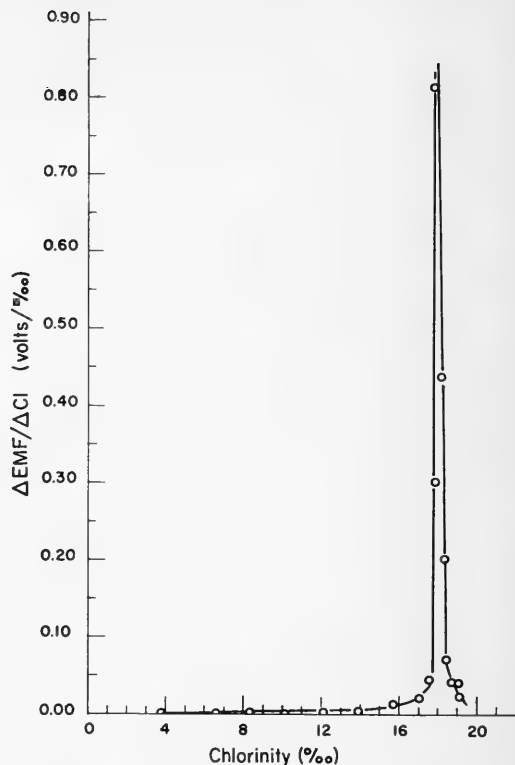
Fig. 8. Derivative curve for potentiometric titration of sea water with silver nitrate. Maximum of this curve corresponds to equivalence point shown in Figure 7.
