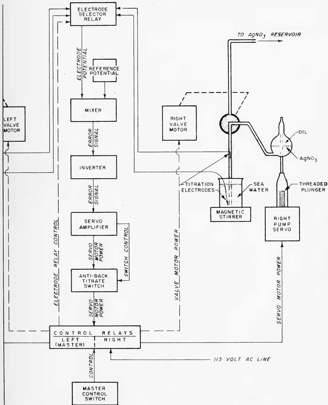
Fig. 6. Block diagram, Automatic Chlorinity Titrator, showing Servo System and Right Titration Unit.
