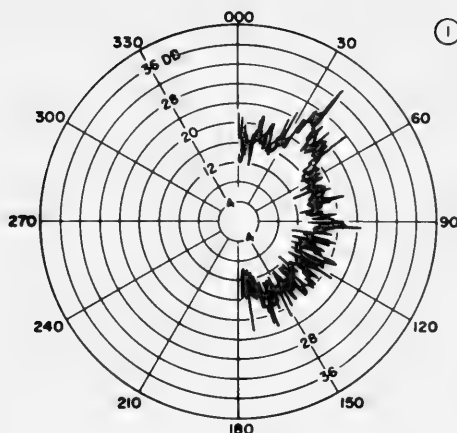
Fig. 4B. Noise-field Hydrophone at 100 feet Receiver Attenuator at 0 db
