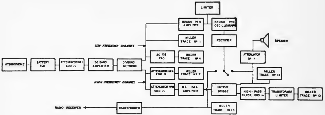
Fig. 12. Block diagram of recording system.
