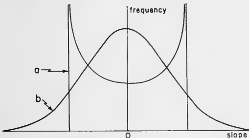
Fig. 1. Frequency distribution of slopes for (a) a single train of sine waves, and (b) a Gaussian sea surface.
