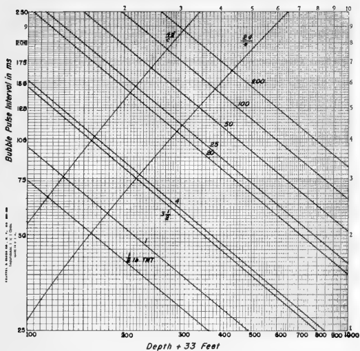
Fig. 8. Dependence of bubble-pulse frequency.
