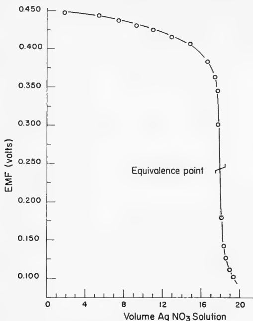
Fig. 7. Potentiometric titration curve of sea water with silver nitrate. Indicator electrode was Ag:AgCl. Reference electrode was Ag:Ag
