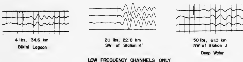
Fig. 14. Sample oscillogram of seismic refraction shots in Bikini Lagoon and in deep water outside Bikini Atoll.
