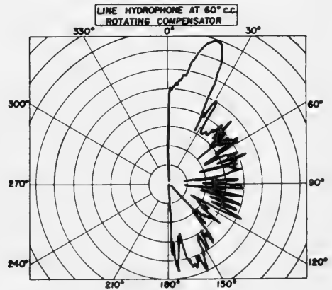
Fig. 2D. 10-foot Line Hydrophone with Compensator at 8 kc.
