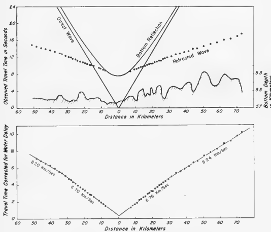
Fig. 2. Seismic refraction observations at a station southeast of Hawaii.
