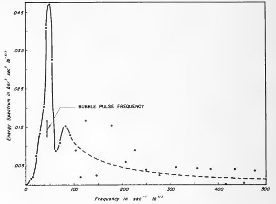
Fig. 5. Low-frequency part of the Fourier energy spectrum of an explosion at 500 feet depth.
