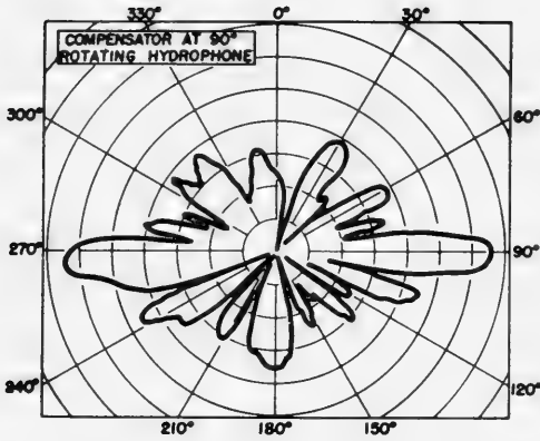
Fig. 3A. 10-foot Line Hydrophone with Compensator at 2.5 kc.
