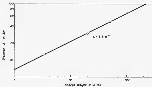
Fig. 16. Maximum range of detection of beginning of the bottom refracted wave, as a function of charge weight.
