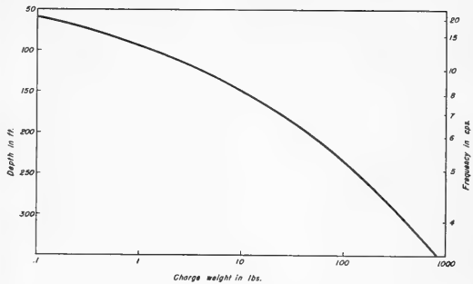
Fig. 9. Optimum charge depth as a function of charge weight.
