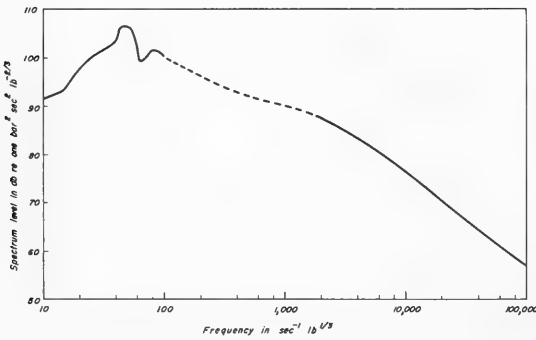
Fig. 6. Complete Fourier energy spectrum.
