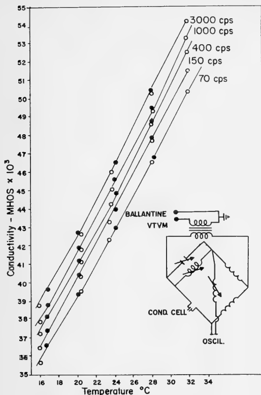
Fig. 4. Variation of apparent conductivity cell as a function of frequency and temperature. Insert is schematic of circuit containing conductivity cell. Sequence of measurements was 16°C, 70 to 3000 cps; 20°C, 70 to 3000 cps; etc. to 32°C, and then repeat as system cooled to 16°C. Open circles measurement on heating cycle; closed circles while cooling.
