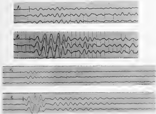
Fig. 10. Effect of increasing charge weight from 4 to 50 lbs. In each of the two pairs of oscillograms the upper one represents a 4 lb. charge and the lower one a 50 lb. charge. The distances are approximately 25 km.
