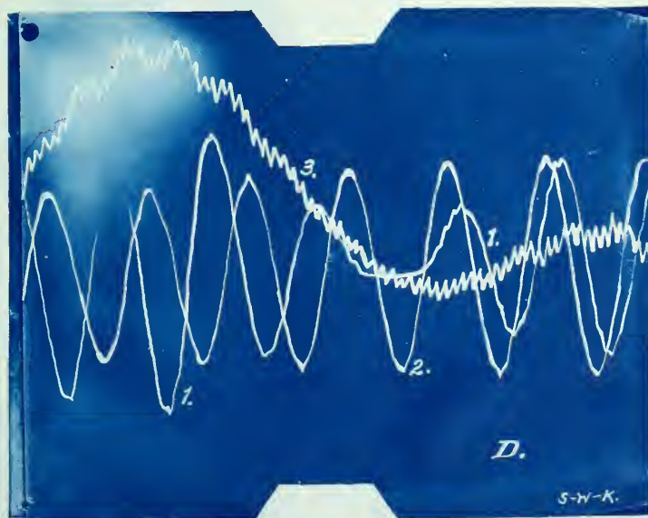
3-phase. I_p = 5 amperes. Load = 0. 1 = stator current. 2 = impressed e.m.f. 3 = rotor current.
