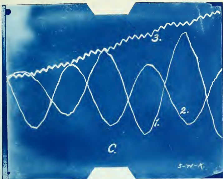
3-phase. I_p = 4 amperes. Load = 0. 1 = stator current. 2 = impressed e.m.f. 3 = rotor current.
