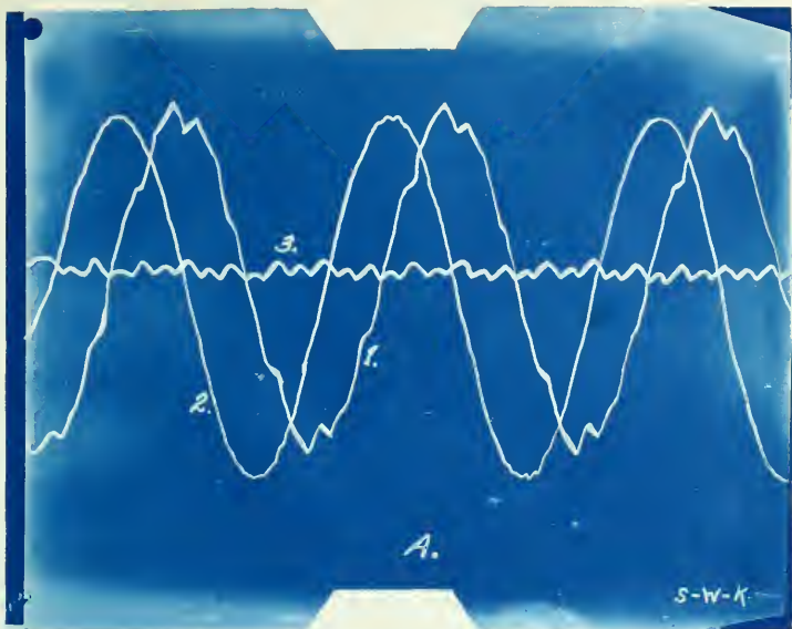
3-phase. I_f = 2 amperes. Load = 0. 1 = stator current. 2 = impressed e.m.f. 3 = rotor current.
