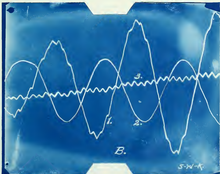
3-phase. I_f = 3 amperes. Load = 0. 1 = stator current. 2 = impressed e.m.f. 3 = rotor current.
