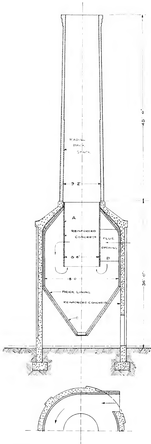
Fig. 5—A Cross Section Through the Cinder Collector and the Stack
