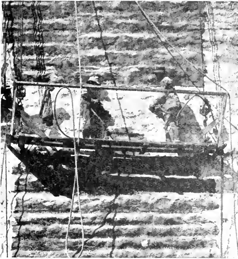
Fig. 3. Part of Basin Wall showing method of removing asphalt coating
