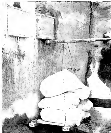
Fig. 7. Showing test to determine adhesion of gunite to asphalt membrane
