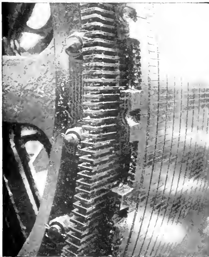
Fig. 3. A Portion of Rotor Showing Double Squirrel-Cage Winding
