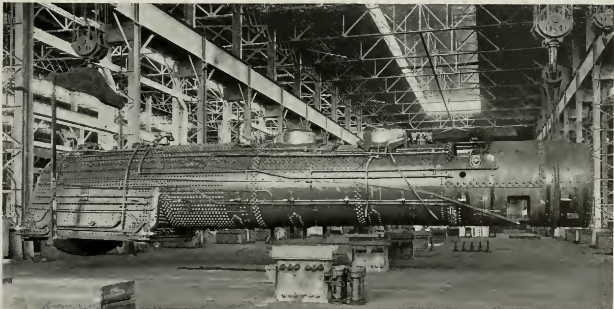
Boiler and Firebox for Northern Pacific 4-8-4 Locomotive, Built 1934. Length Overall 53 feet, 7 inches
