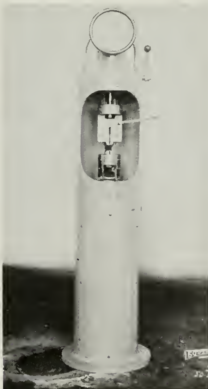
Courtesy Welding Engineer Weld Testing Machine
