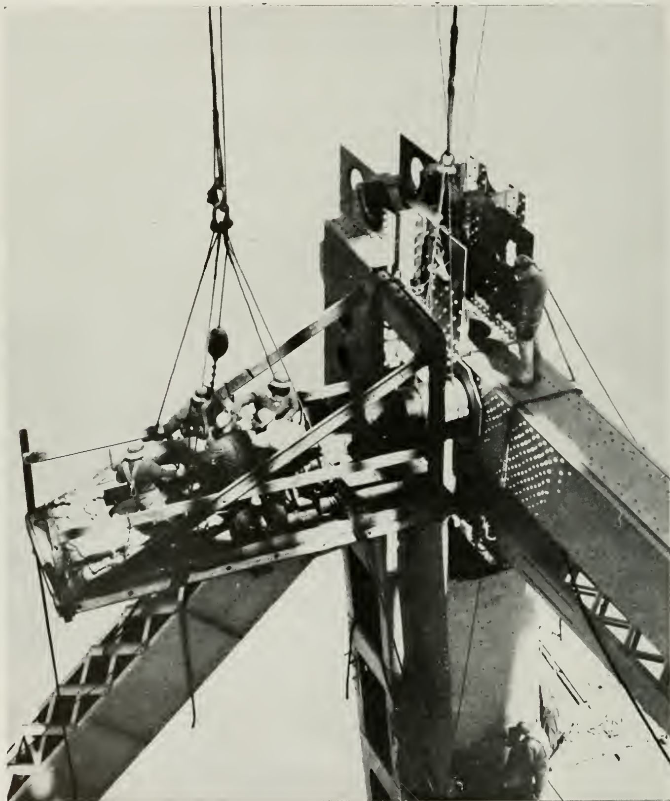
Workmen driving a 24-inch pin at the junction of the West Anchor Span of the longest cantilever bridge in the United States, the east bay crossing of The San Francisco-Oakland Bay Bridge.
