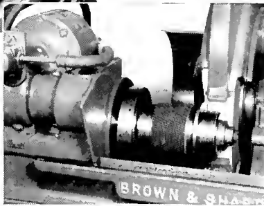
Right—Accurately sizing base of cylinder on No. 20 Plain Grinding Machine.
