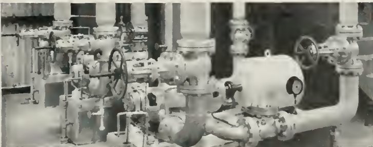
POWER PLANT. Boiler feed water pumps and Jenkins Valves shown. MAIN ARCHITECTS: Paul Charbonnet, Jr. GENERAL CONTRACTOR: Gervais Fayrol Co. MECHANICAL & PLUMBING CONTRACTOR: Comfortaire Co., Inc. CONSULTING ENGINEERS: Leo S. Weil; Walter B. Moses.
