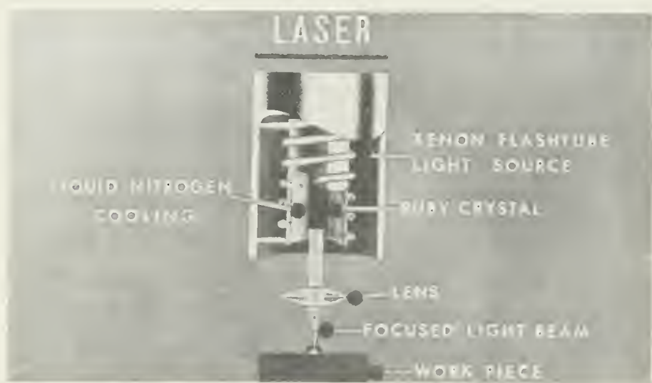
Figure 2. Typical Laser apparatus for pulsed operation.
