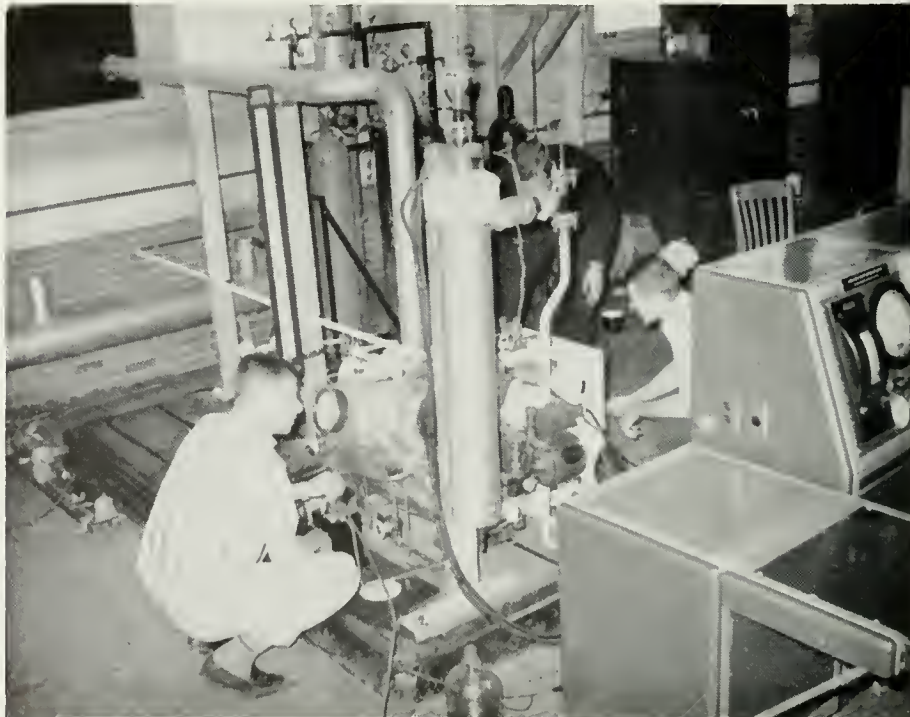
Figure 1. As part of the practical application of the theory taught in the classroom, several Mechanical and Industrial engineering students are shown running tests on the adiabatic compression machine in the Internal Combustion Engine Laboratory.
