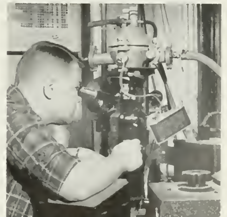
Figure 2. High temperature microscope used in Ceramic Engineering Department to study changes in microstructure of materials during heating to high temperatures.
