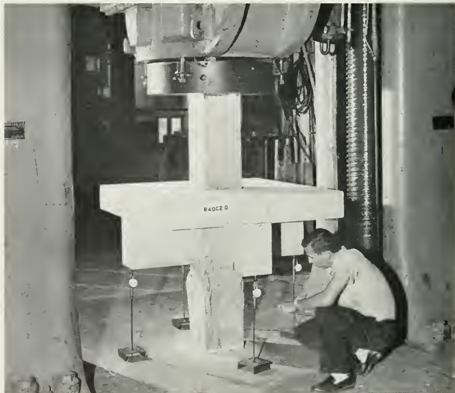
Figure 1. A graduate student is examining the failure in a reinforced concrete specimen. The specimen was loaded by the partly visible machine, which can exert 3,000,000 pounds of compression or expansion.
