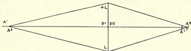
FIG. 6.—Ordinary lens.
