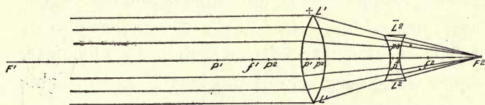
FIG. 5.—Telephoto lens.
