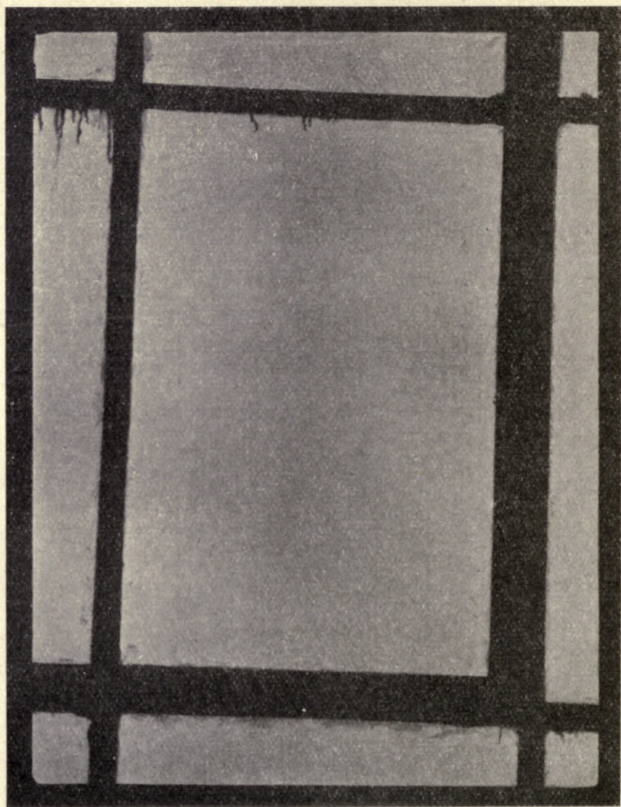
PLATE 10.—WINDOW.—Taken with the Adon with the baseboard tilted at 13^{\circ} to the horizontal, focusing screen perpendicular to the baseboard. Here the inner frame appears wider at the bottom than at the top.
