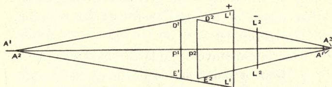
FIG. 7.—Telephoto lens.
