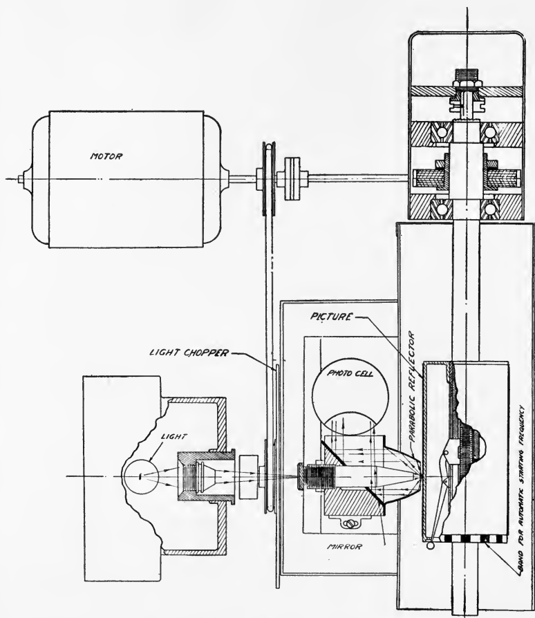
FIG. 69.—Westinghouse facsimile picture transmitter.
