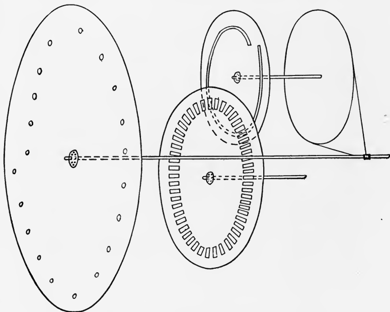
FIG. 76.—Scanning arrangement used in the Baird system.
