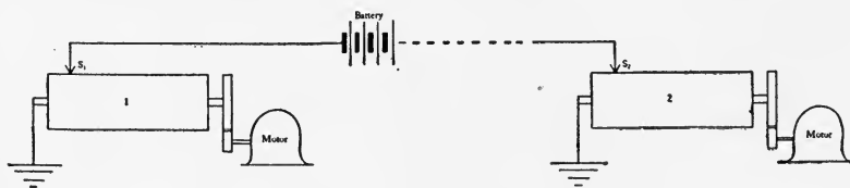
FIG. 2.—Bakewell system.
