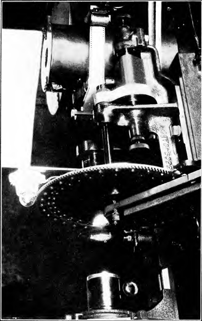
FIG. 129.—The heart of the television motion picture transmitter of the Westinghouse Electric and Manufacturing Company. The scanning-disc is clearly shown as well as the dot of light which is thrown upon the motion picture film. Above the scanning-disc may be seen the synchronizing tube which keeps the disc turning at a predetermined speed.
