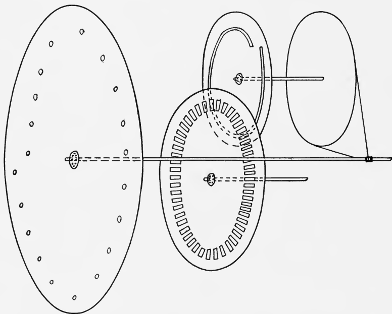
FIG. 47.—Scanning arrangement used in the Baird system.
