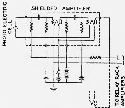
FIG. 94.—Schematic diagram of the first two stages of the vacuum-tube amplifier used with the photoelectric cells in the Bell equipment.
