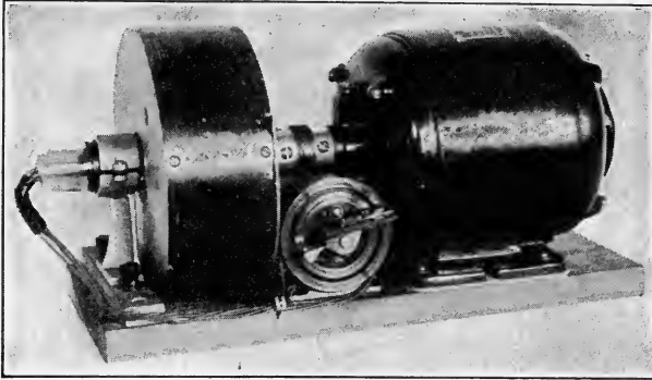
FIG. 117.—Mounting of Jenkins' drum-scanner.
