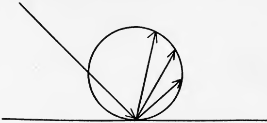
FIG. 10.—In the case of a diffusing surface reflection follows Lambert's cosine law. This is shown above where the length of arrow represents the amount of light reflected in any chosen direction.
