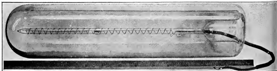
FIG. 92.—Detail of a photoelectric cell of the type used in the Bell apparatus. Note large area of photo-sensitive coating.
