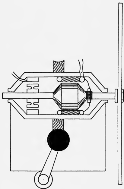
FIG. 56.—Scanning-disc motor and speed control. The large unit, near the disc, is the d.c. drive motor; the smaller unit, at the base of the same shaft, is the synchronous motor used as a speed control.
