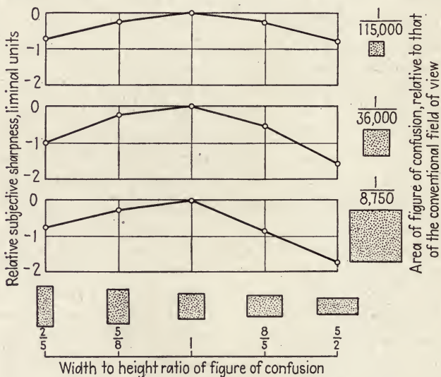
FIG. 63.—Sharpness of motion pictures as a function of the relative values of horizontal and vertical resolution. Field of view as in Fig. 61. Each point represents 150 observations at 30 in. ( M. W. Baldwin, Jr. )
