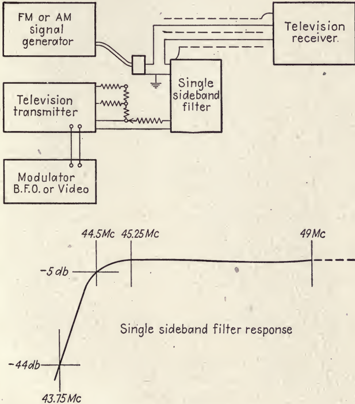
FIG. 17.—Block diagram of setup used in testing the use of f-m sound signals. (W. L. Dunn.)
