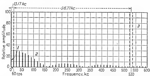
FIG. 84.—Frequency spectra: (1) low-frequency nonserrated field pulse; (2) 8 per cent line pulse, 13,230 c.p.s.; (3) high-frequency field pulse. (Campbell and Lempert.)
