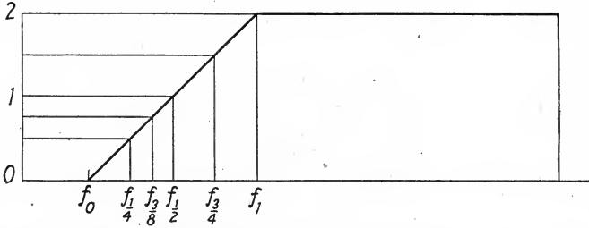
FIG. 65.—Idealized receiver-frequency characteristic. (R. D. Kell.)
