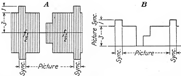
FIG. 66.—Transmitter-output waveforms, method 1. (R. D. Kell.)
