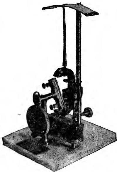
Fig. 12A. Ewing Hysteresis Tester.
