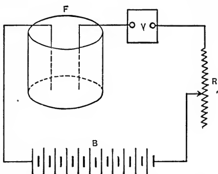
Fig. 23A. Calibration of a Voltmeter by the Voltmeter Method.
