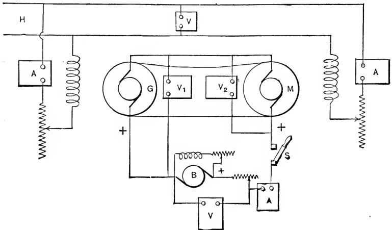
Fig. 75. Potter Method of Testing Dynamo Machines.
