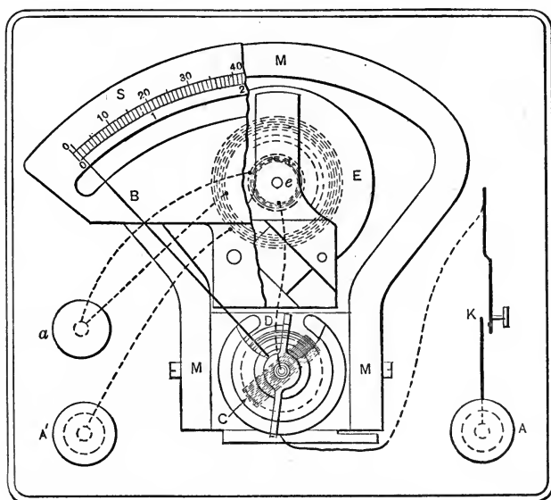
Fig. Lb. Weston Direct Current Voltmeter Connections.
