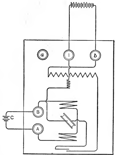
Fig. H. Weston Wattmeter Connections (independent circuits).
