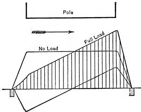
Fig. 42. Magnetic Distribution under a Pole Face.
