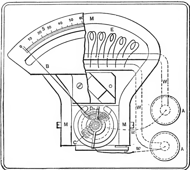
Fig. M. Weston Direct Current Ammeter Connections.
