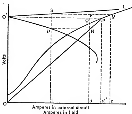
Fig. 34. Graphical Method of Compounding a Shunt Dynamo.
