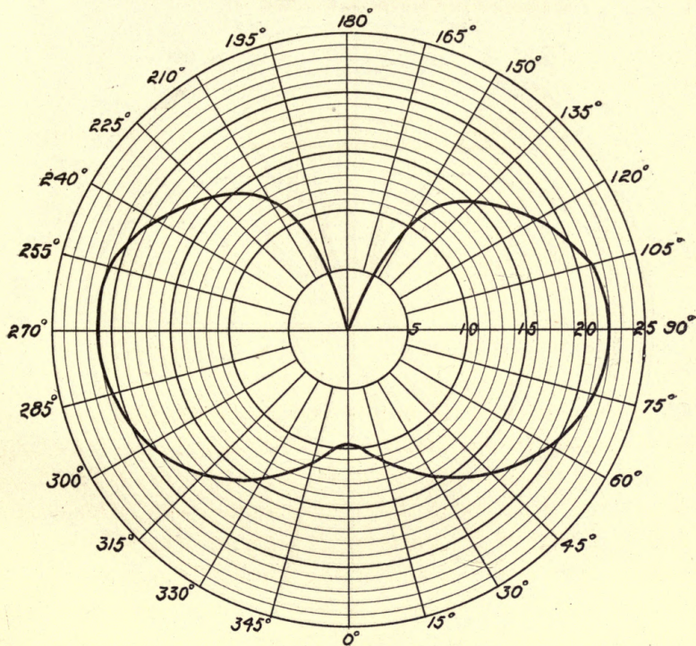
VERTICAL DISTRIBUTION OF C LAMP
