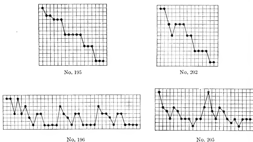
FIG. 40. Plots, Group 7.
