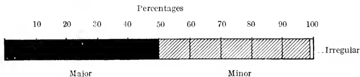
FIG. 1. Tonality.
