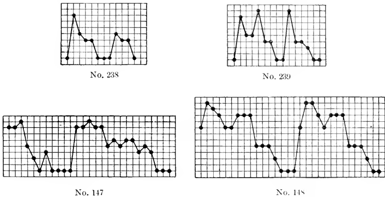
FIG. 43. Plots, Group 8.
