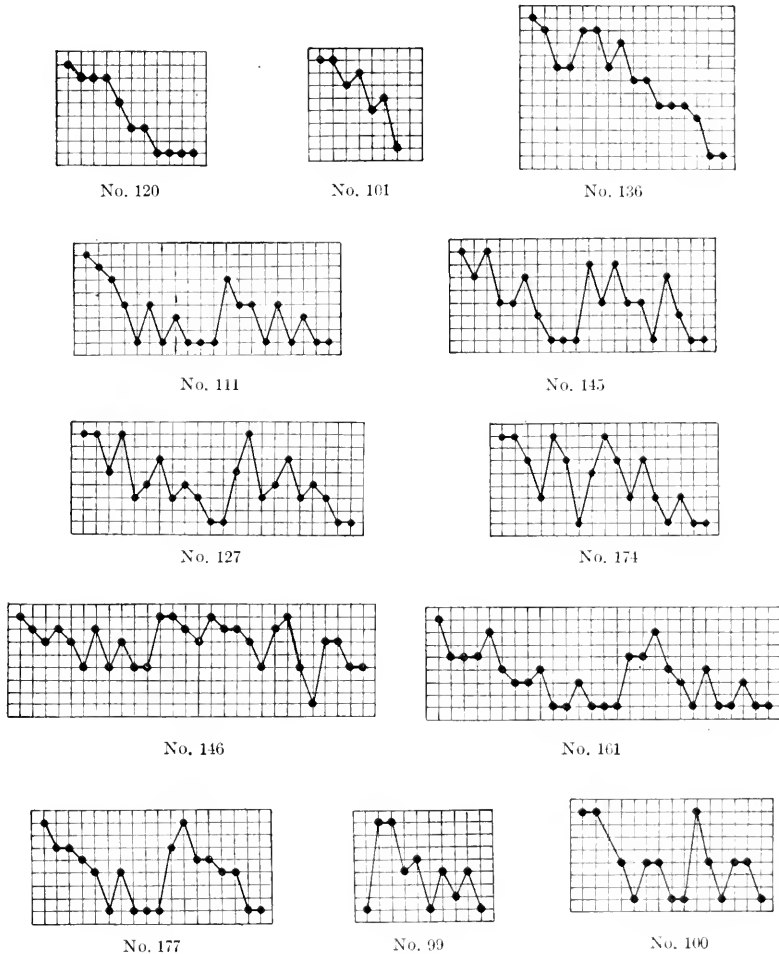
FIG. 35. Plots, Group 5.
