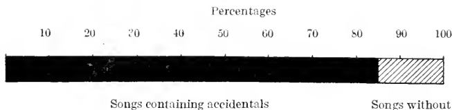
FIG. 8. Accidentals.
