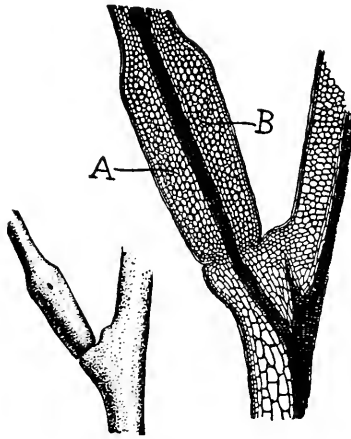
FIG. 47. Pulvinus and section of pulvinus from leaf of sensitive plant, both enlarged. When the leaf is touched, the water in the cells on side A passes outward into the intercellular spaces, causing the cells partially to collapse. The pressure of the cells on side B then forces the leaf downward. Courtesy World Book Co.
