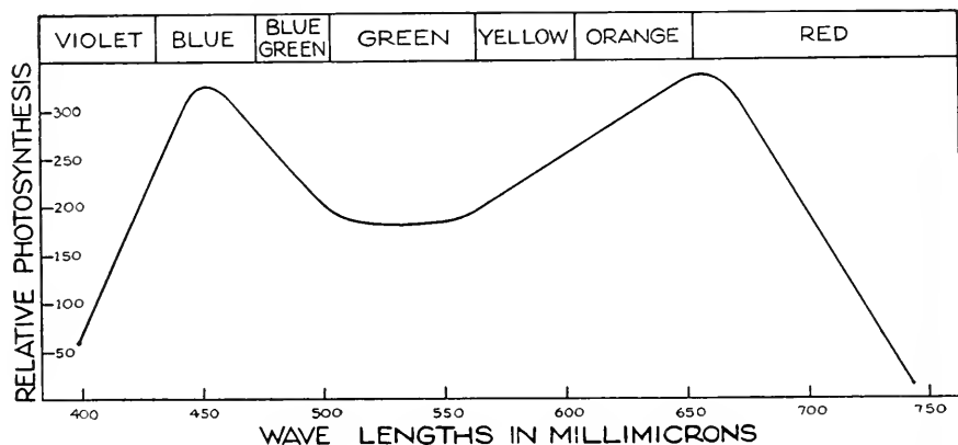
FIG. 54. Relative rates of photosynthesis in different rays of light of equal intensity. After B. S. Meyer and D. B. Anderson.
