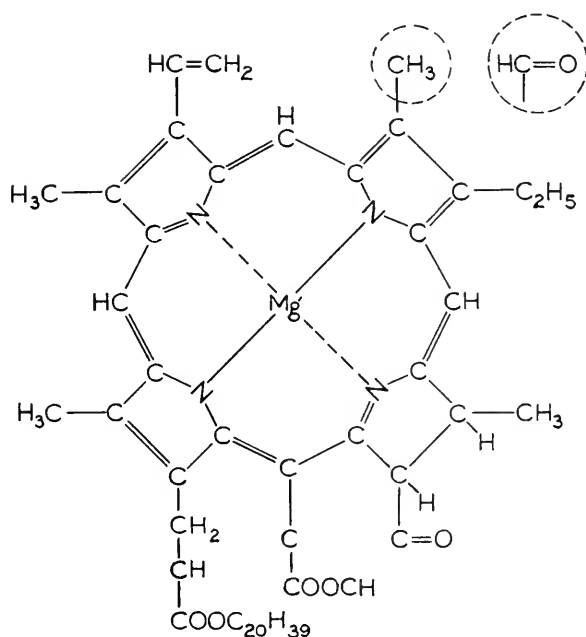
FIG. 56. Diagram representing the arrangement and complexity of the molecule of chlorophyll a. If the group, CHO, in the detached circle is substituted for the CH 3 group nearby, the diagram would represent the molecule of chlorophyll b. From B. S. Meyer and D. B. Anderson, 1939.
