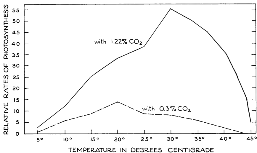
FIG. 58. Rates of photosynthesis in potato leaves in relation to temperature and the concentration of carbon dioxide. Calculated from data by H. G. Lundegardh.
