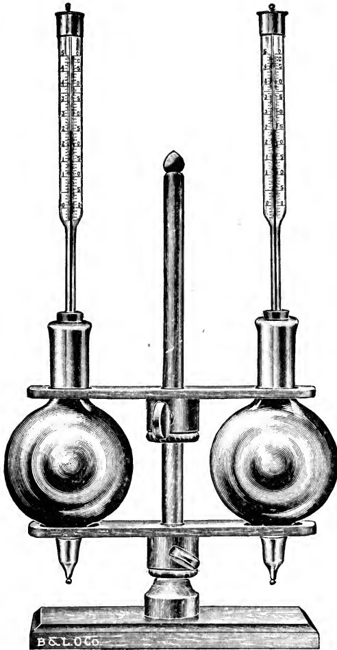
FIG. 117. — A Caloriscopes; \times \frac{1}{5} . The two Dewar bulbs have double walls with a vacuum between (as familiar in "Thermos" bottles), and hence prevent loss of heat. The respiring tissue to be tested is divided into two parts, and placed in the two flasks, but is immediately killed in one. Thus the delicate thermometers are made to record within a few hours the degree of heat released by the respiration of the living tissues.
