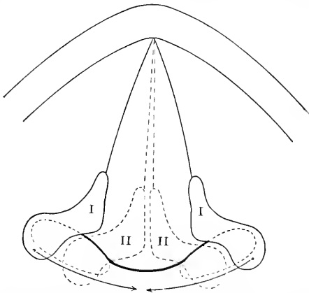
FIG. 434.—Diagrammatic section of larynx to illustrate action of Arytenoideus proprius muscle (after Landois).
