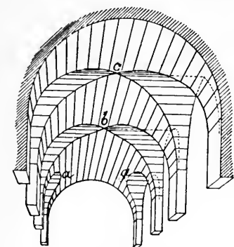
FIG. 112.—PENETRATIONS AND INTERSECTIONS OF VAULTS.
