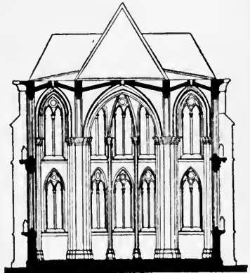
FIG. 145.—SECTION OF ST. ELIZABETH, MARBURG.
