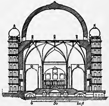
FIG. 86.—TOMB OF MAHMÛD, BIJAPUR. SECTION.
