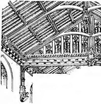
FIG. 143.—ROOF OF NAVE, ST. MARY'S, WESTON-ZOYLAND.
