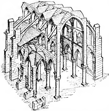
FIG. 108.—CONSTRUCTIVE SYSTEM OF GOTHIC CHURCH, ILLUSTRATING PRINCIPLES OF ISOLATED SUPPORTS AND BUTTRESSING.
