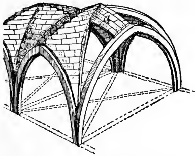
FIG. 122.—GROINED VAULT WITH ZIG-ZAG RIDGE-JOINTS.
