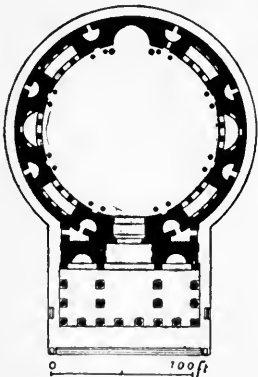
FIG. 54.—PLAN OF THE PANTHEON.
