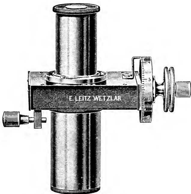
FIG. 207.—Screw micrometer eyepiece (Filar micrometer).
