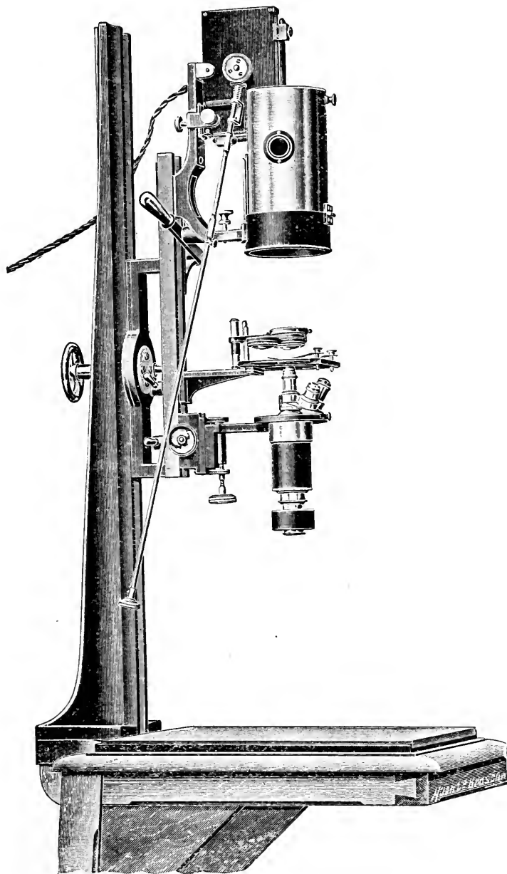
FIG. 235.—Edinger's drawing apparatus arranged for microscopic drawing.
