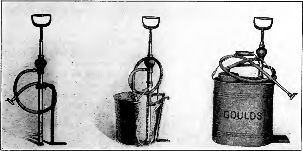
FIG. 238.—Spray pumps isolated and with bucket attachments.
