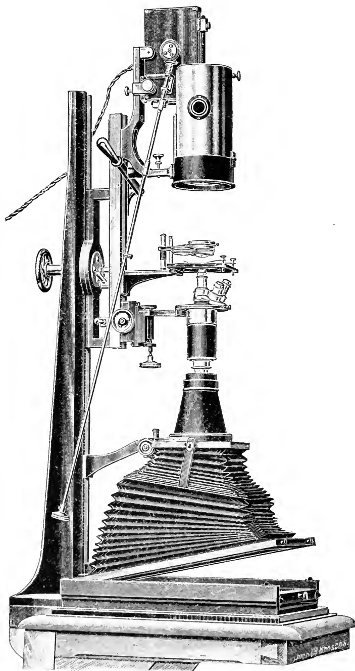
FIG. 236.—Edinger's drawing apparatus with attachment for photo-micrography.
