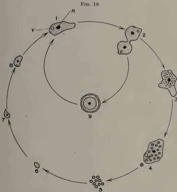
Schematic life cycle of the Entamoeba histolytica : 1, the adult amœba with nucleus (n) and contractile vacuole (v); 2, the same, multiplying by amitotic division; 3, appearance of chromidial granules in cytoplasm, which enlarge and become the spores in 4; these spores become discharged or liberated (5) and develop (6, 7, 8) into the adult amœba, or (9) under other conditions the amœba passes into an encysted stage. (After E. L. Walker.)
