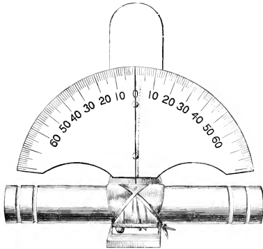
FIG. 33. HÆMATACHOMETER OF CHAUEAU AND LORTET.
