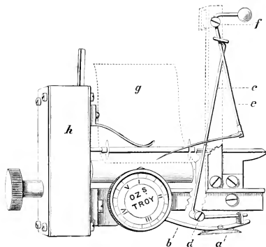
FIG. 43. DIAGRAM OF A SPHYGMOGRAPH (Dudgeon's).
