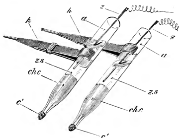
FIG. 18. NON-POLARISABLE ELECTRODES.
