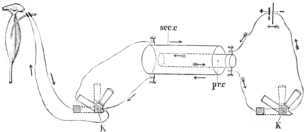
FIG. 4. DIAGRAM OF AN INDUCTION COIL.
