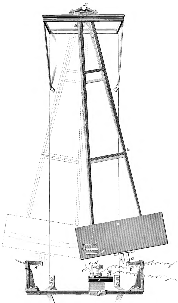
FIG. 10. THE PENDULUM MYOGRAPH.
