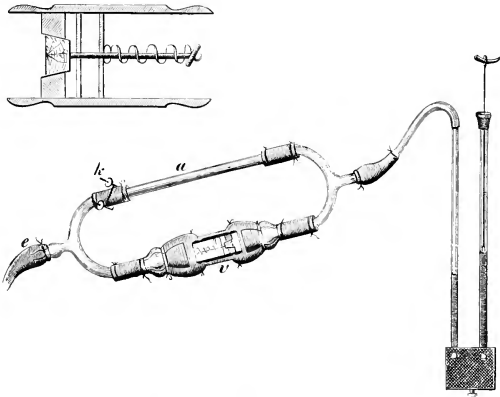
FIG. 36. THE MAXIMUM MANOMETER OF GOLTZ AND GAULE.
