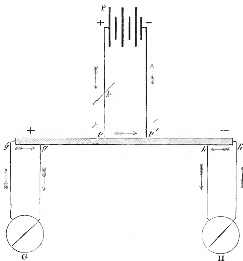
FIG. 23. DIAGRAM ILLUSTRATING ELECTROTONIC CURRENTS.
