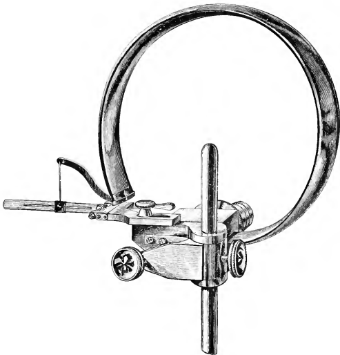
FIG. 42. FICK'S SPRING MANOMETER.
