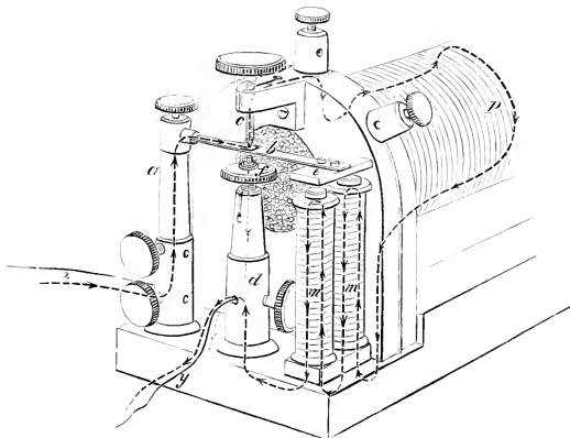
FIG. 5. THE MAGNETIC INTERRUPTOR.
