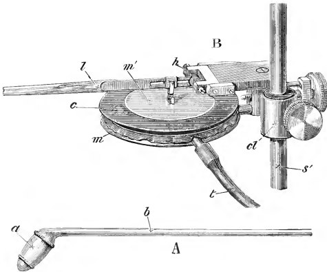
FIG. 37. MAREY'S TAMBOUR, WITH CARDIAC SOUND.
