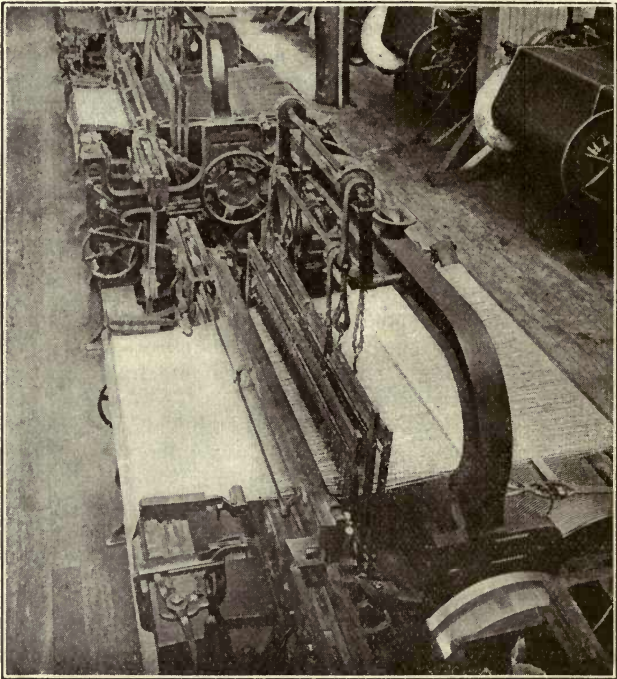
FIG. 25.— MODERN LOOM.
