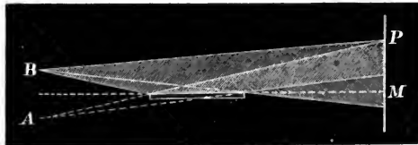
Fig. 83.—Lloyd's Single Mirror.
