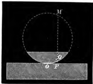
Fig. 96.—Newton's Rings.
