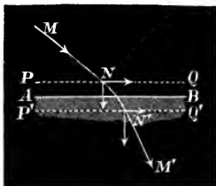
Fig. 2.—Refraction of a Light Molecule.
