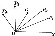
Fig. 12.—Resultant of a system of similar Vibrations.
