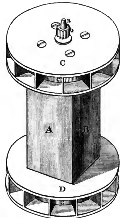
Fig. 224.—The Revolving Mirror.
