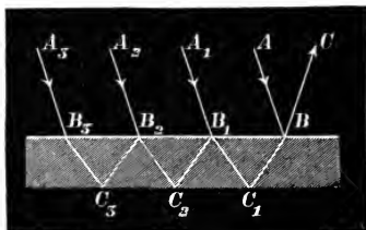
Fig. 94.—Multiple Reflections.
