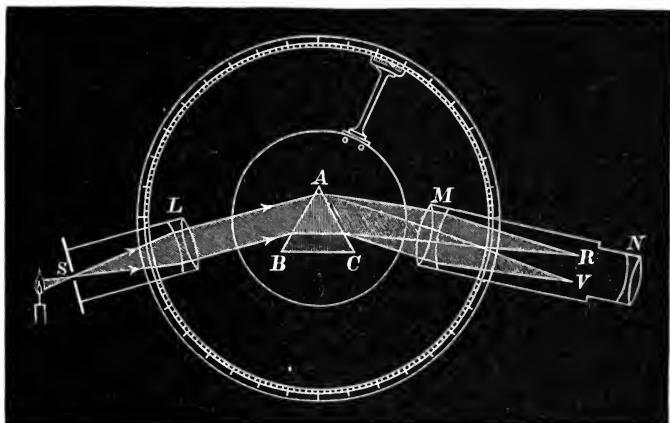
Fig. 73.—The Spectrometer.
