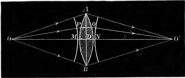
Fig. 58.—Aplanatic Lens.
