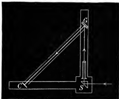
Fig. 118.—Concave Grating.
