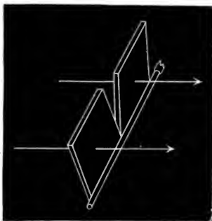
Fig. 104.—The Compensator.
