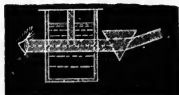
Fig. 92.—Stokes's Modification.
