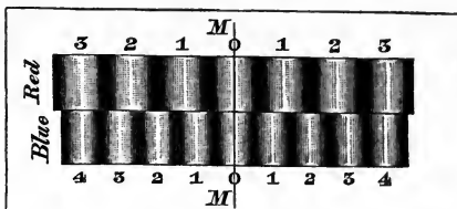
Fig. 85.—Overlapping of the Fringes.
