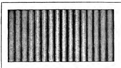
Fig. 5.—Interference Bands.
