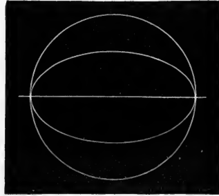
Fig. 152.—Positive Crystals.
