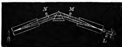
Fig. 89.—Talbot's Bands.
