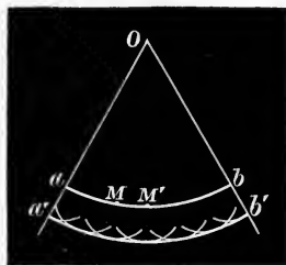
Fig. 23.—Propagation by Secondary Waves.
