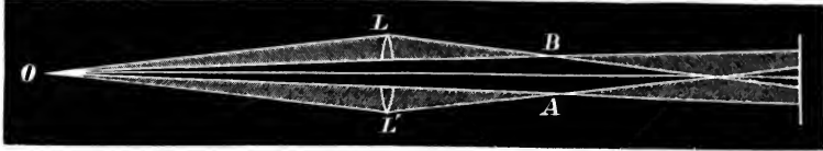
Fig. 87.—Billet's Split Lens.
