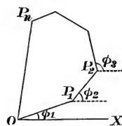
Fig. 13.—The Vibration Polygon.
