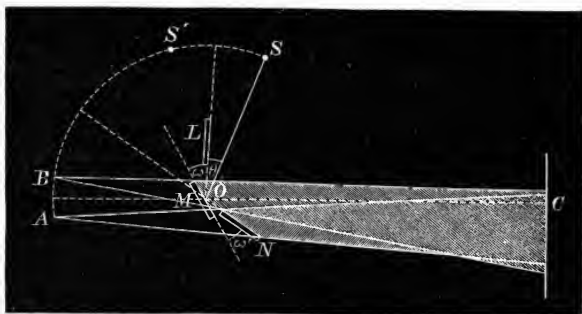
Fig. 84.—Fresnel's Three Mirrors.
