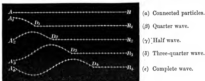
Fig. 7.—Transverse Waves.
