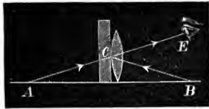
Fig. 97.—Arago's Experiment.
