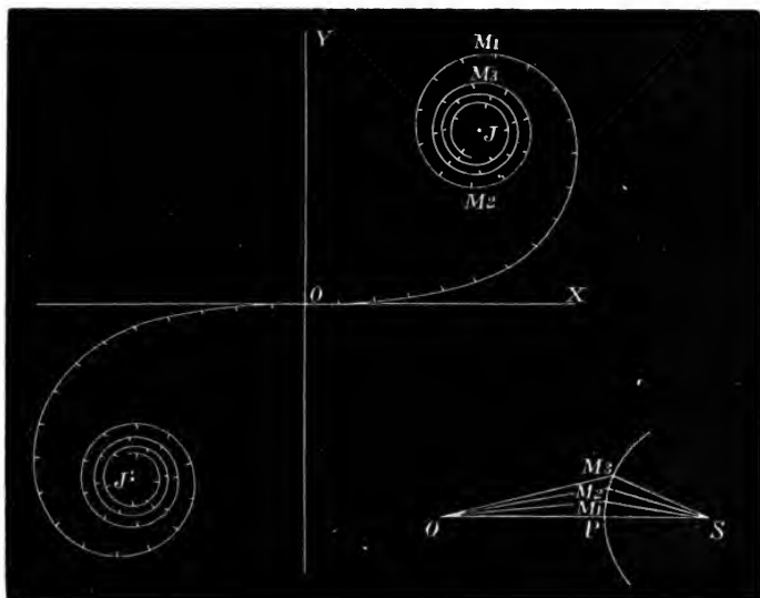
Fig. 145.—Cornu's Spiral.
