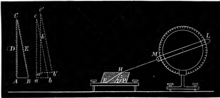
Fig. 157.—Verification of Huygens's Wave Surface.
