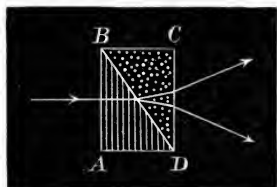
Fig. 163.—Wollaston's Prism.
