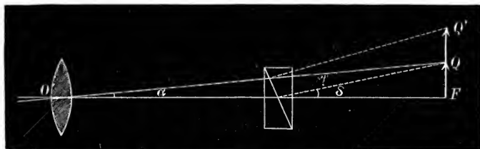
Fig. 162.—Double Image Micrometer.
