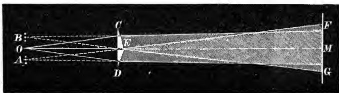
Fig. 81.—Fresnel's Bi-prism.
