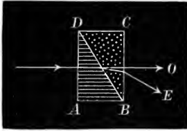
Fig. 161.—Rochon's Prism.
