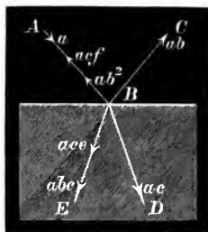
Fig. 95.—Reflection and Refraction Coefficients.
