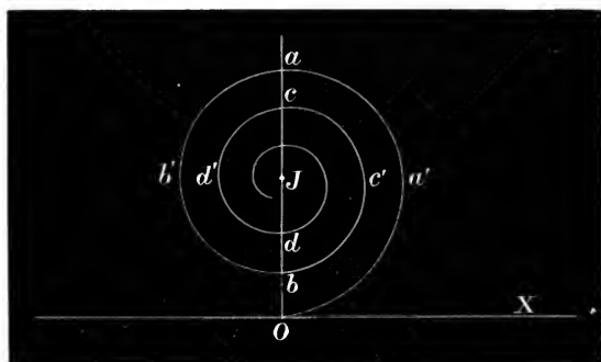
Fig. 121.—Vibration Spiral.
