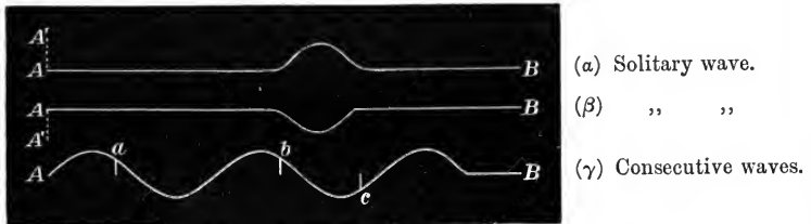
Fig. 6.—Transverse Waves.
