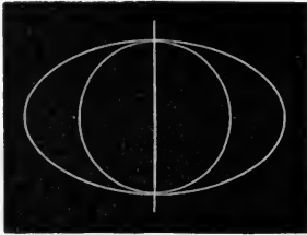
Fig. 151.—Negative Crystals.
