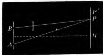
Fig. 86.—Displacement of the Central Band.
