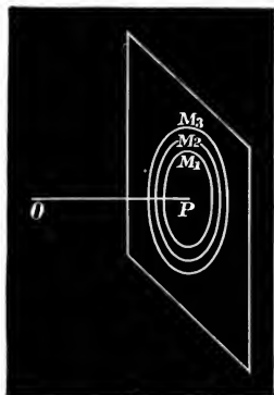
Fig. 24.—Half-period Elements.
