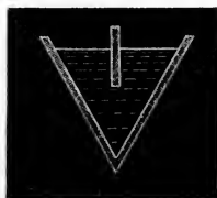
Fig. 90.—Powell's Bands.
