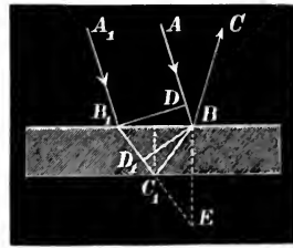
Fig. 93.—Thin Plate, Retardation.
