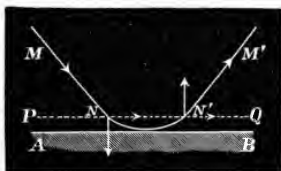
Fig. 1.—Reflection of a Light Molecule.
