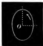
Fig. 20.—Phase Difference a Right Angle.
