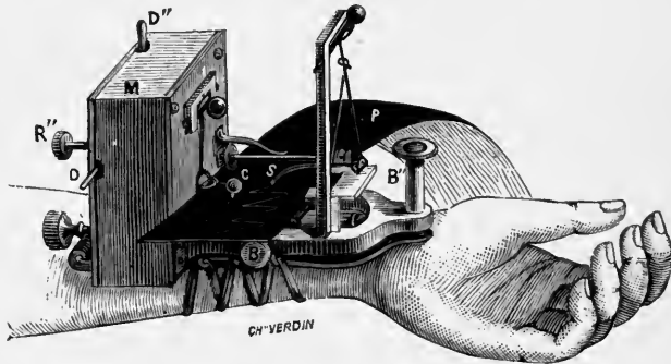
FIG. 123. Dudgeon's sphygmograph.
