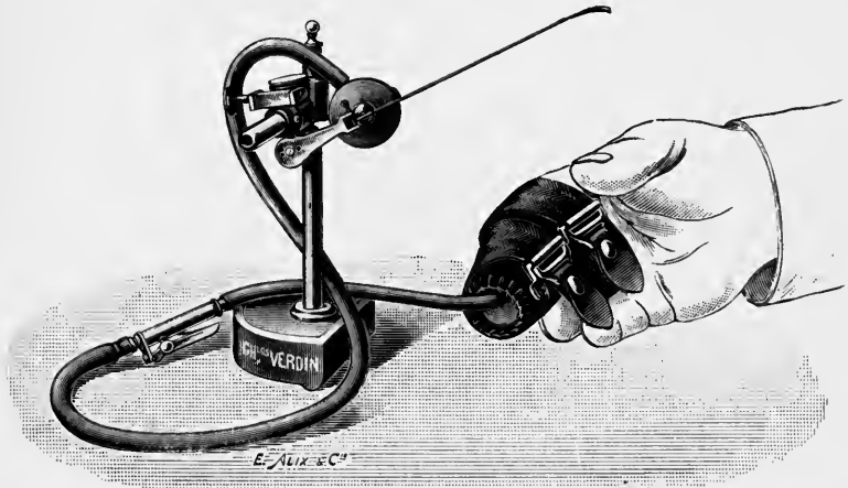
FIG. 94. Plethysmograph of Hallion and Comte.
