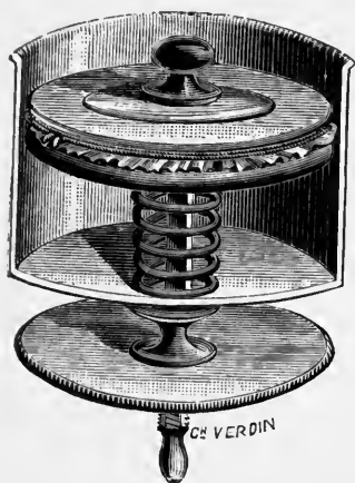
FIG. 106. Marey's cardiograph.
