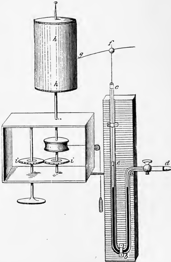
FIG. 71. Ludwig's kymograph, copied from Ludwig's Lehrbuch der Physiologie , 2te Auflage, 2ter Band, p. 122. It consists of a bent glass tube, abc , containing mercury, and connected by d with the artery of an animal. ef is a slender upright rod, swimming on the surface of the mercury, and bearing at its free end, f , a brush, g , which registers the movements of the mercury on the revolving cylinder, hh .
