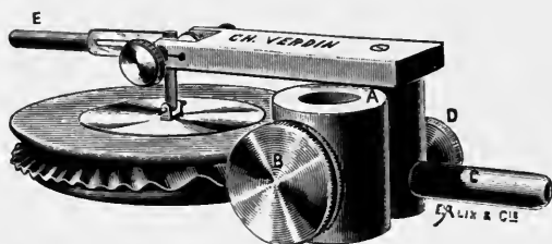
FIG. 104. Marey's tambour for recording movements. It is a metal ring which slides on an upright rod, and can be fixed at any height by the screw B . C is the tube through which the air from the receiving instrument (sphygmograph, cardiograph, etc.) communicates with that inside the tambour and causes the cover E to rise or fall. Into E a long straw is fastened bearing a point which records its movements on a cylinder.
