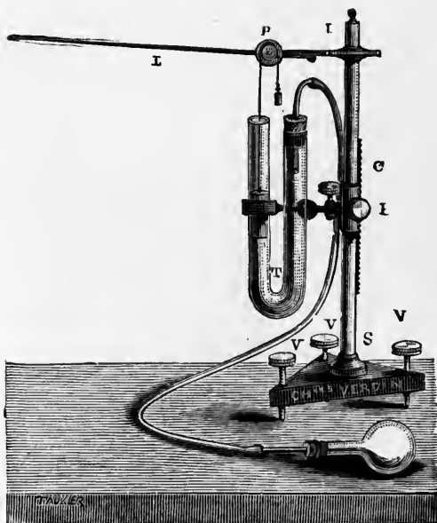
FIG. 9. Lelaunie's manometer. It consists of ( T ) a bent tube containing mercury. The open arm bears a float, the movements of which are transmitted by a pulley ( P ) to the lever ( L ), which amplifies and records them. By means of a pinion ( B ) working on a rack ( C ), the apparatus can be moved up and down on a stand ( S ), which is rendered vertical by three screws ( V V V ). The open end of the tube can be connected with a caoutchouc bag, as in the figure. It was originally designed to record the rectal temperature in a dog during tetanization, but it could be used for other purposes. Burdon-Sanderson's kymograph was similar to this, but the two limbs of the U tube were of unequal width, and the lever was longer.
