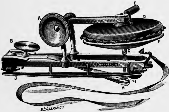
FIG. 122. Marey's transmitting sphygmograph.
