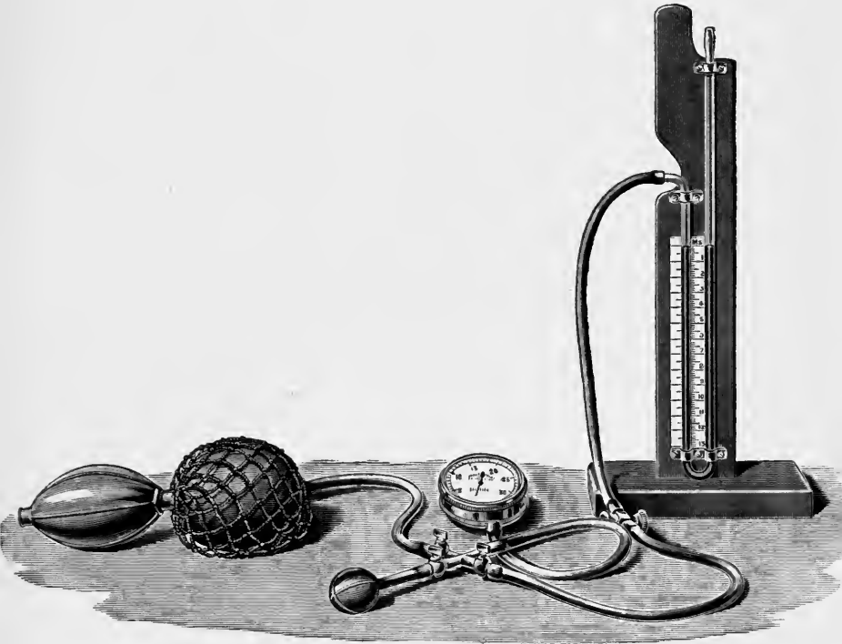
FIG. 103. Author's apparatus for ascertaining the correctness or amount of error in an aneroid sphygmomanometer. By means of a three-way stopcock both the aneroid and a mercurial manometer are put into communication with a pressure bulb of a spray apparatus. The pressure is then raised 50 mm. at a time, and the readings of the mercurial and aneroid compared at each pressure.
