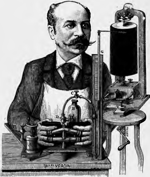
FIG. 93. Mosso's sphygmomanometer. It consists of metal tubes ( EE ) filled with water, which is prevented from coming out by india-rubber finger-stalls into which the fingers are inserted. The apparatus is then quite filled with water from the bottle B , air being allowed to escape at C . The pressure is then raised by compressing the water in the reservoir ( A ) by the screw at its top until the mercury in the manometer ( G ) registers the maximum oscillation, which may be taken as the diastolic pressure. The pressure is then raised until the mercury ceases to oscillate, and this may be taken as the systolic pressure.
