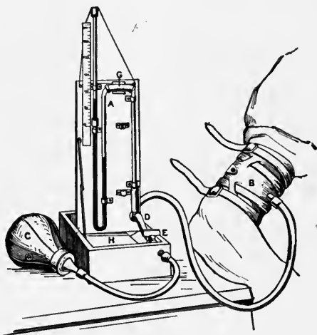
FIG. 234. Janeway's sphygmomanometer.
