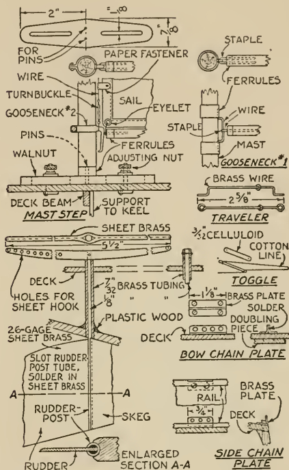
FIG. 57.—Mast step, rudder, two types of gossenecks, toggles, traveler, chain plates.
