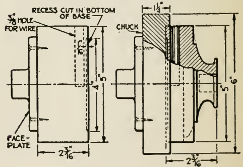
FIG. 50.—The base is roughed out on the faceplate (left), then finished in a wooden chuck with a suitable recess (right).
