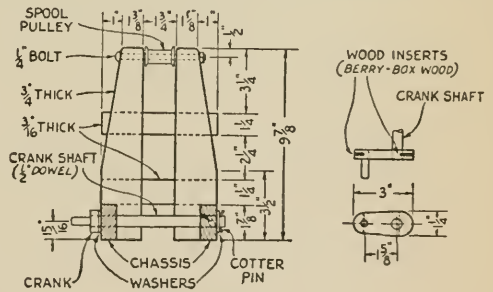
FIG. 10.—How the hoist (left) and crank (right) for the dump truck are made.
