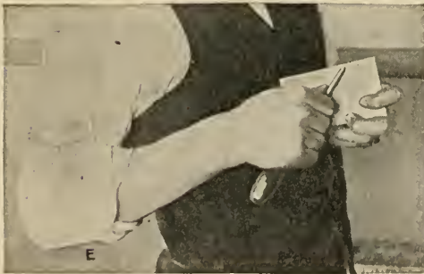
FIG. 8.—Steps in sharpening a cabinet scraper, first by draw filing, second by rubbing it on an oilstone, and third by burnishing it. How a scraper is held in actual use.
