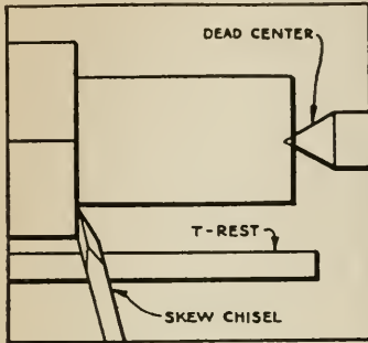
FIG. 37.—Finishing the shoulder of the square cut on the leg.
