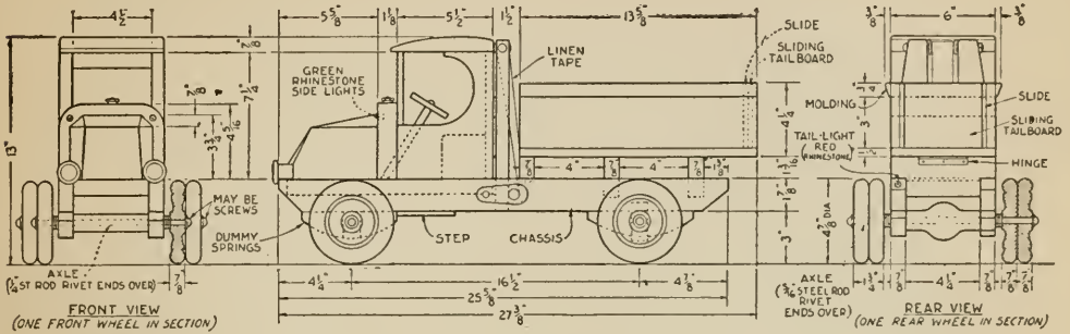
FIG. 9.—Working drawings of the dump truck. Of impressive size, this truck is an exceptionally rugged toy for rough play.
