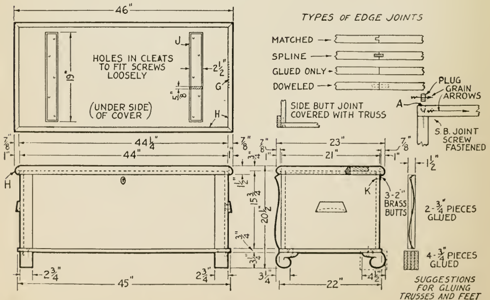
FIG. 8.—Colonial chest with various types of edge joints—matched, splined, butted and glued, doweled, and two kinds of side-butteted and screwed joints. Any of these can be used, of course, in making any types of chest.
