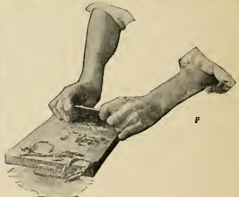
FIG. 8.—Steps in sharpening a cabinet scraper, first by draw filing, second by rubbing it on an oilstone, and third by burnishing it. How a scraper is held in actual use.
