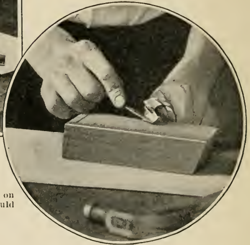
FIG. 4 (above).—How the lips of the bit are sharpened on top by means of an auger bit file.
