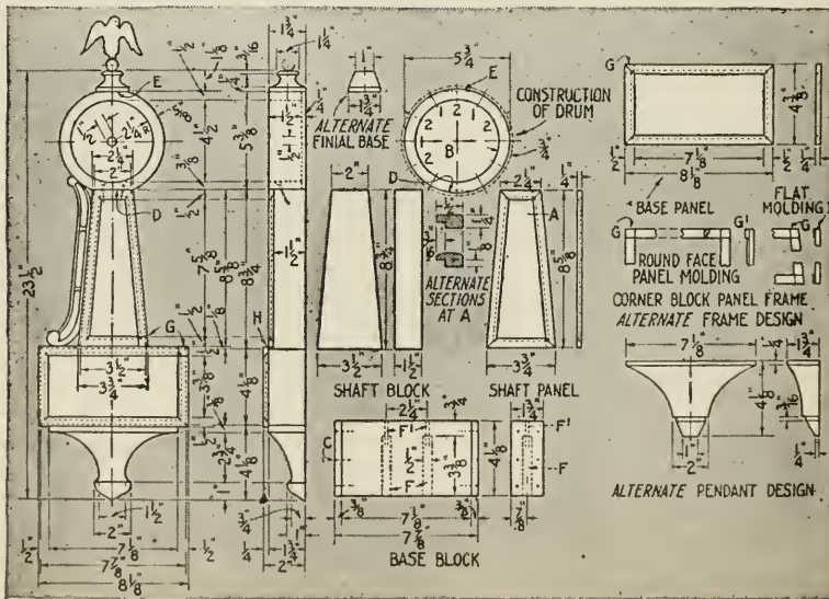
FIG. 22.—Front and side views of a banjo clock case; construction of drum; the shaft and base clocks; panels and moldings; base and pendant designs.
