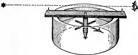
FIRST PIVOTED COMPASS (PEREGRINUS, 1269).
