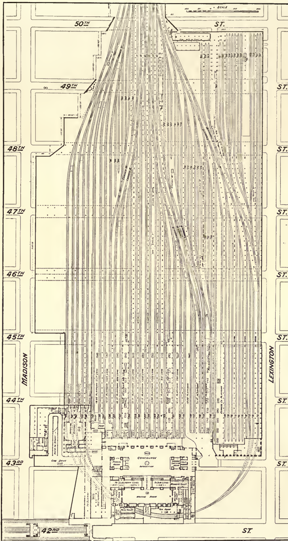
PLATE 36. ONE OF THE TWO SUB-STORY TRAIN YARDS OF THE GRAND CENTRAL TERMINAL, NEW YORK.
