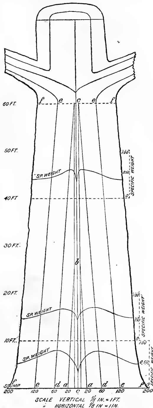
FIG. 2.—Schematic section through stem of Longleaf Pine, showing variation of specific weight with height, diameter, and age at twenty ( aba ), sixty ( ded ), one hundred and twenty ( eee ), and two hundred ( fff ) years.
